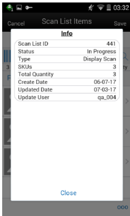
Figure 10–20 Scan List items Info Screen
