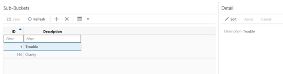
Figure 4-5 Sub-buckets
