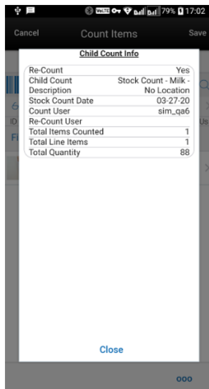
Figure 11–14 Child Count Info Screen
