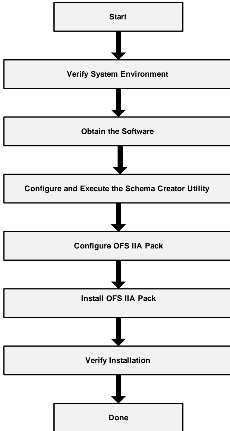
Figure 2–1 Installation Overview
