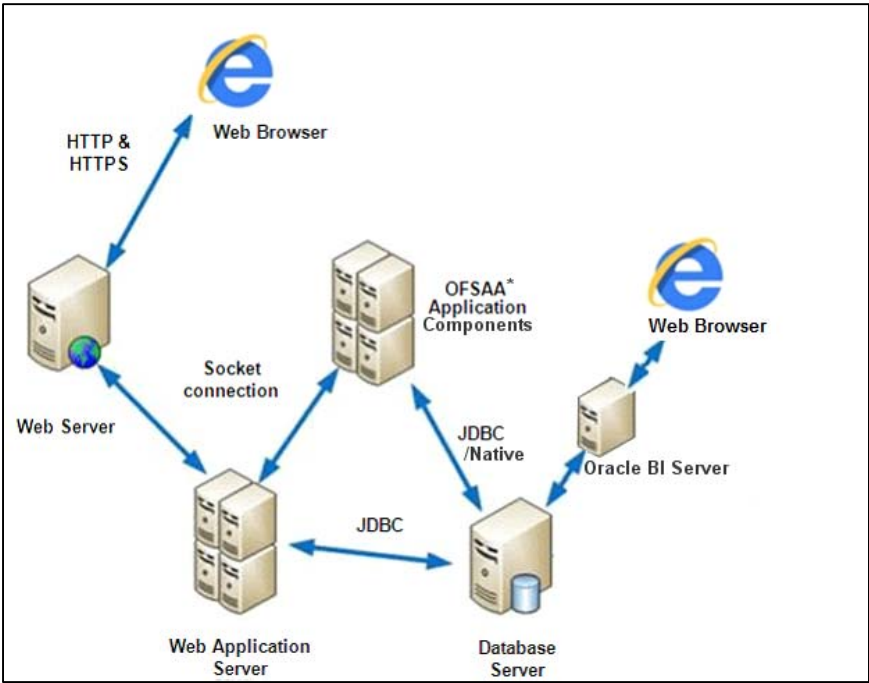
Figure 2-2 Deployment Topology
