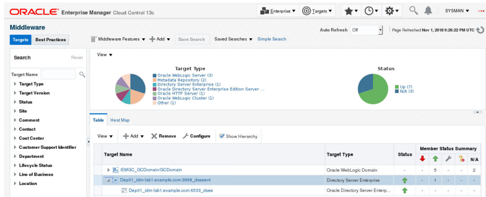
Figure 19-2 Middleware Targets
