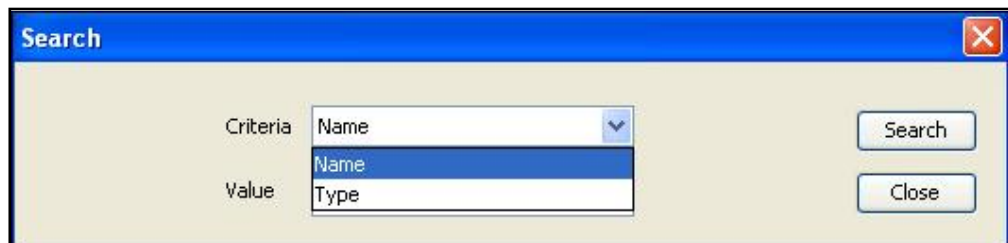
Figure 6–5 Search dialog
