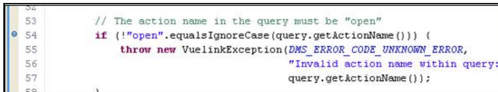
Figure 5-1 Set breakpoint
