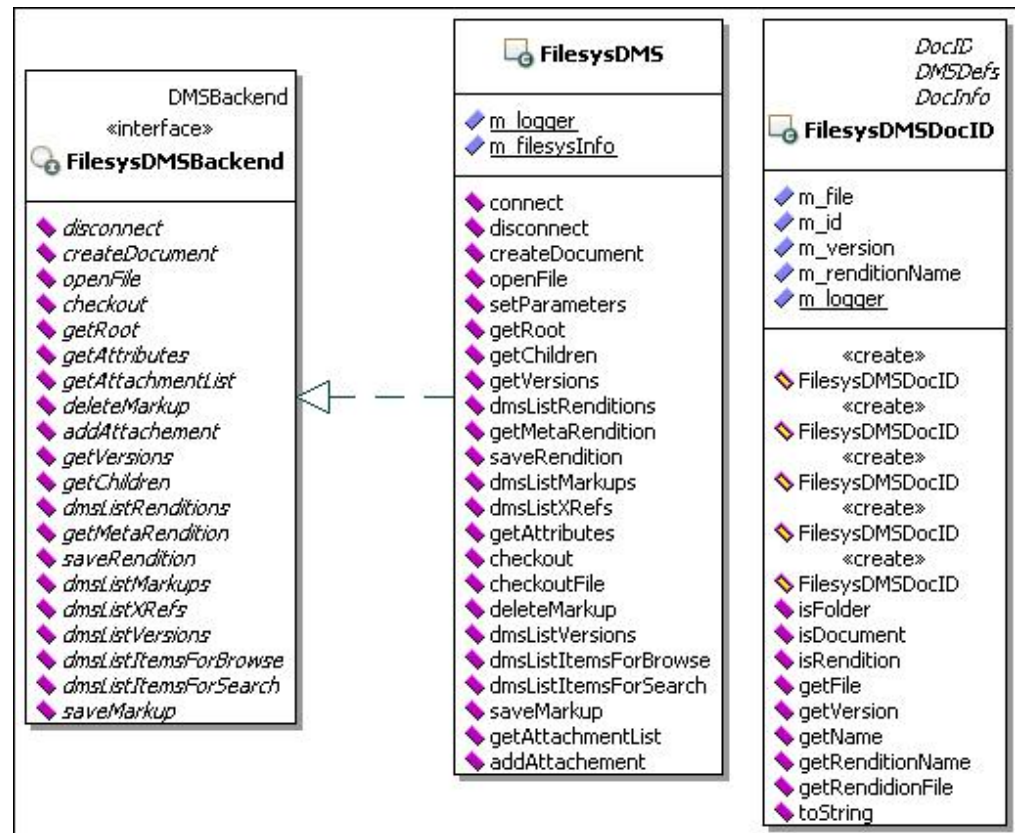
Figure B–3 Backend classes
