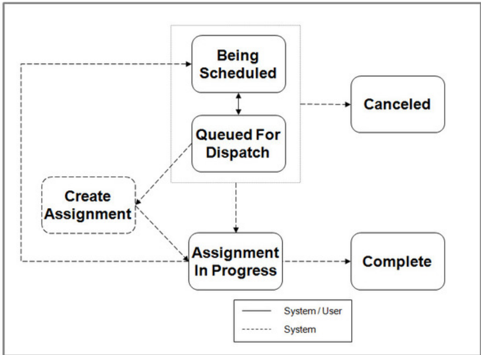
Figure 5: Visit Task Lifecycle
