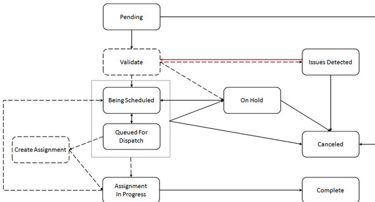
Figure 8: Depot Transfer Activity States
