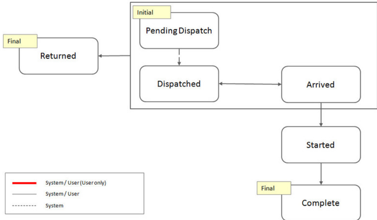
Figure 9: Loading Assignment States
