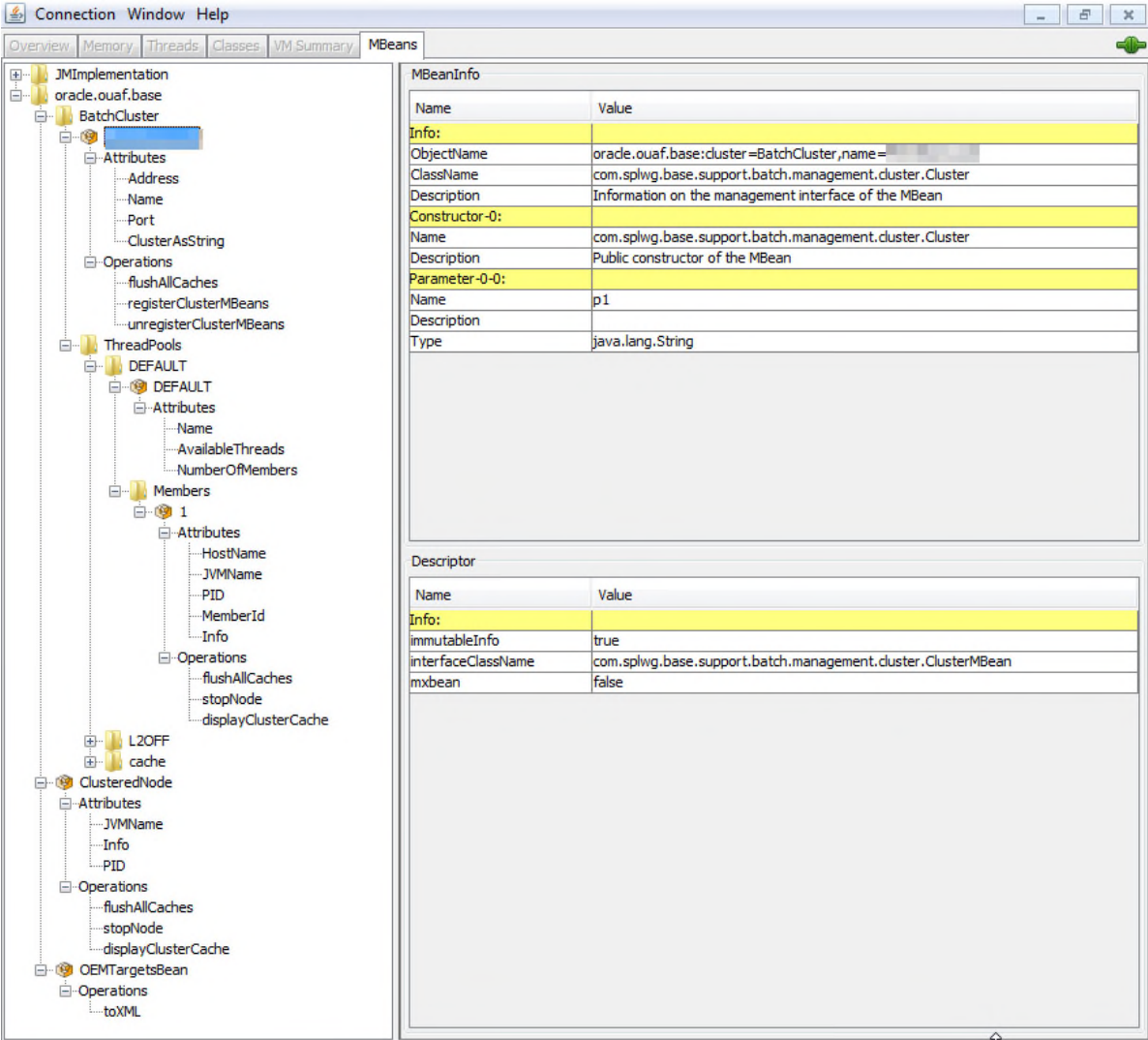
Figure 15 – Example Batch Server Mbeans in jconsole
