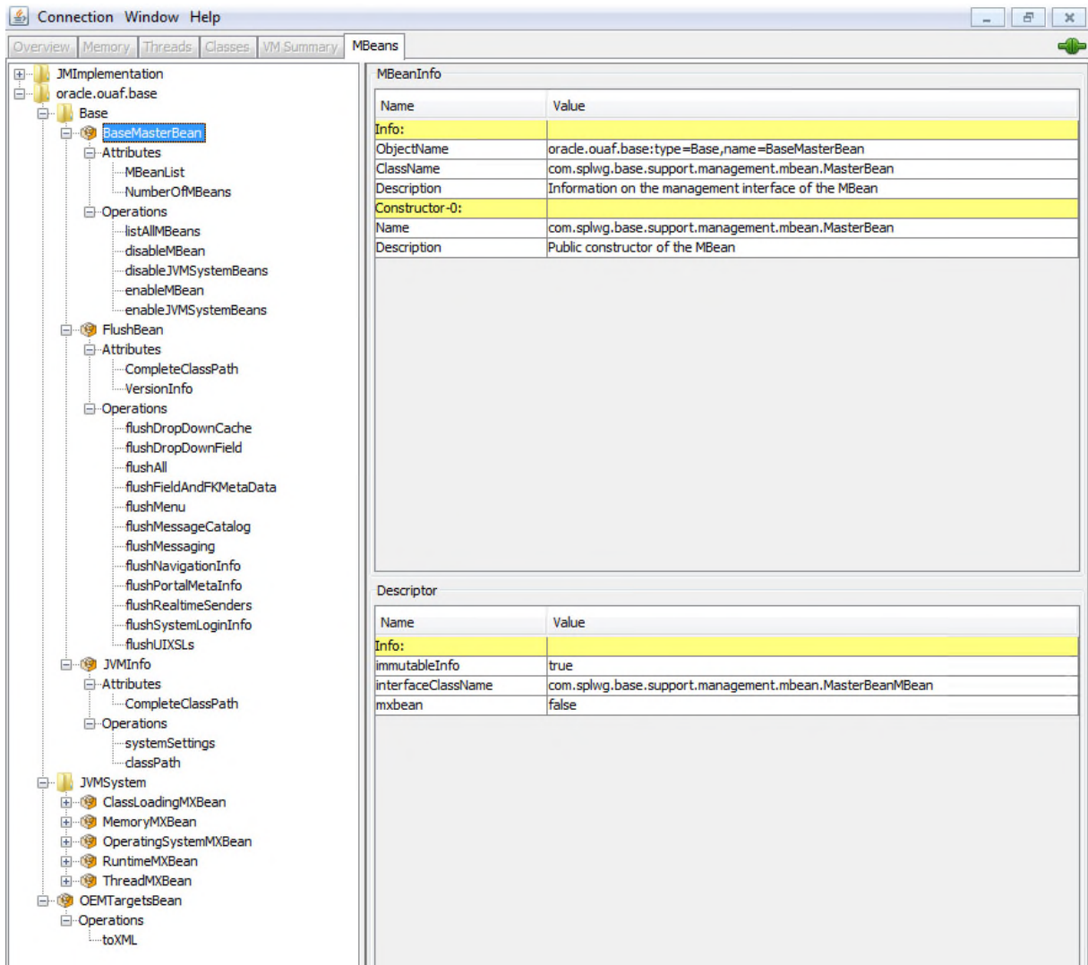
Figure 11 – Example Web Application Server Mbeans in jconsole The structure of the Mbean is shown by the figure below:
