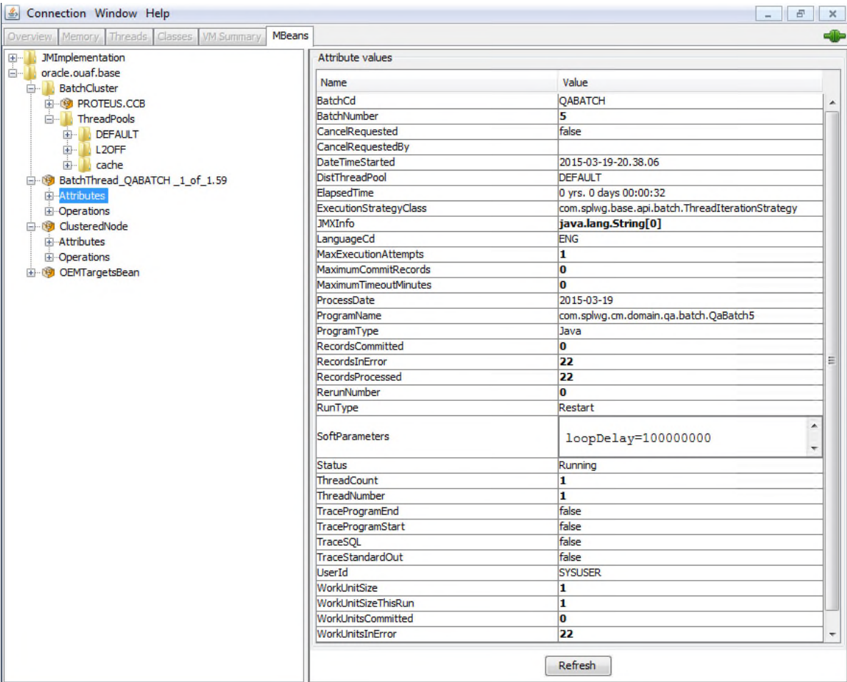
Figure 16 – Example Batch Thread Mbean in jconsole
