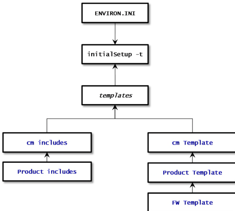
Figure 41 – Template Hierarchy
