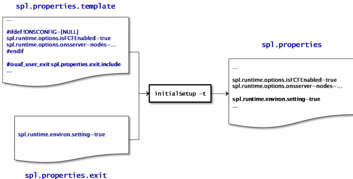
Figure 40 – Include files
