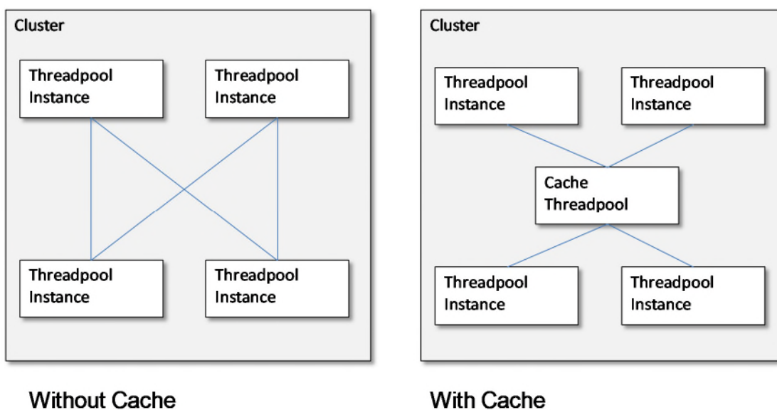
Figure 37 – Cache Architecture
