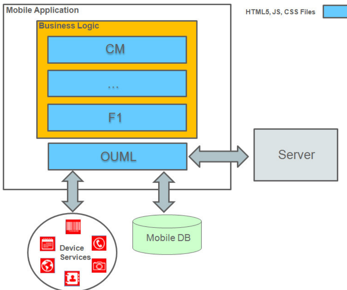
Figure 5: Mobile Application Architecture
