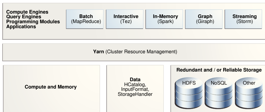
Figure 5-1 Hadoop 2.0 Architecture
