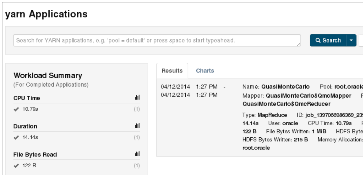
Figure 3-1 Monitoring a YARN Job in Cloudera Manager
