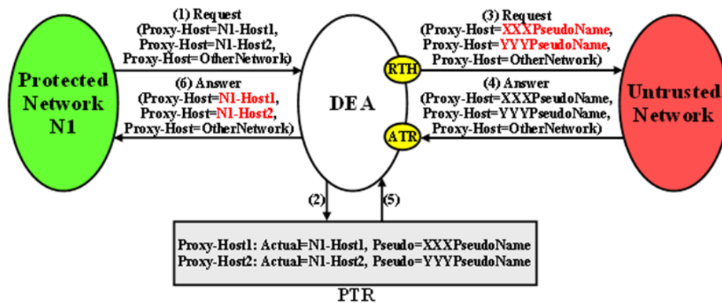
Figure 9-10 Proxy-Host Hiding
