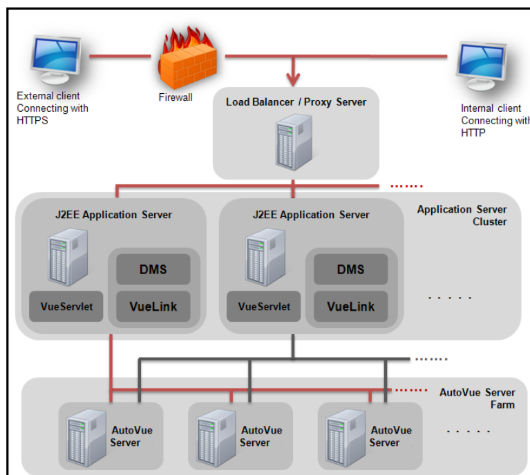
Figure 4–7 Failover Deployment
