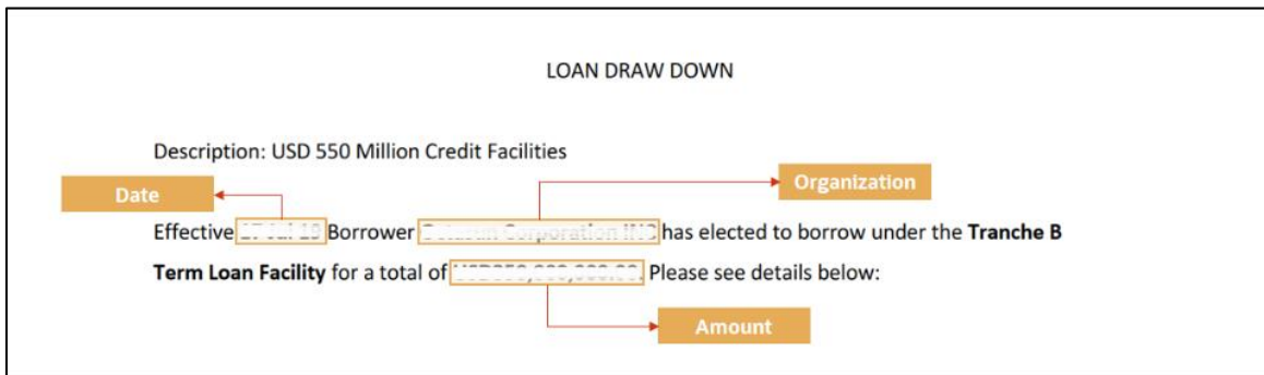
Figure 236: Annotator
