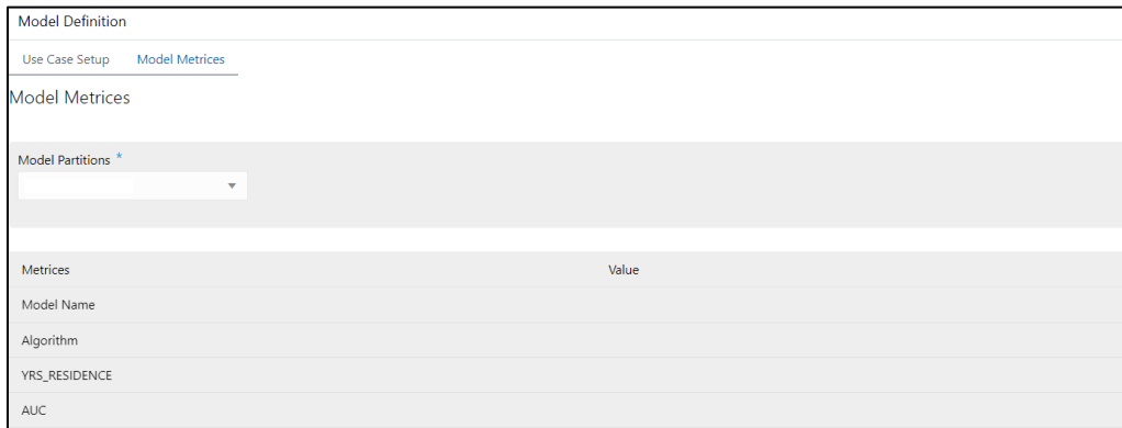
Figure 263: Model Metrics
