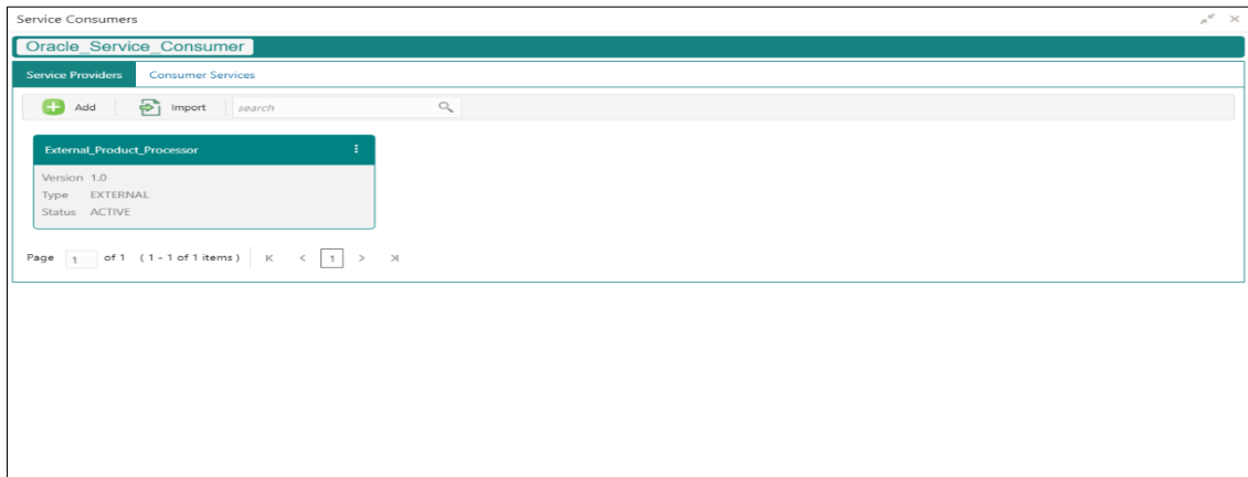
Figure 81: Service Providers
