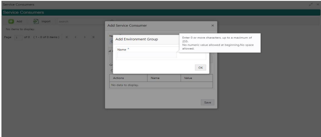
Figure 121: Environment Variables
