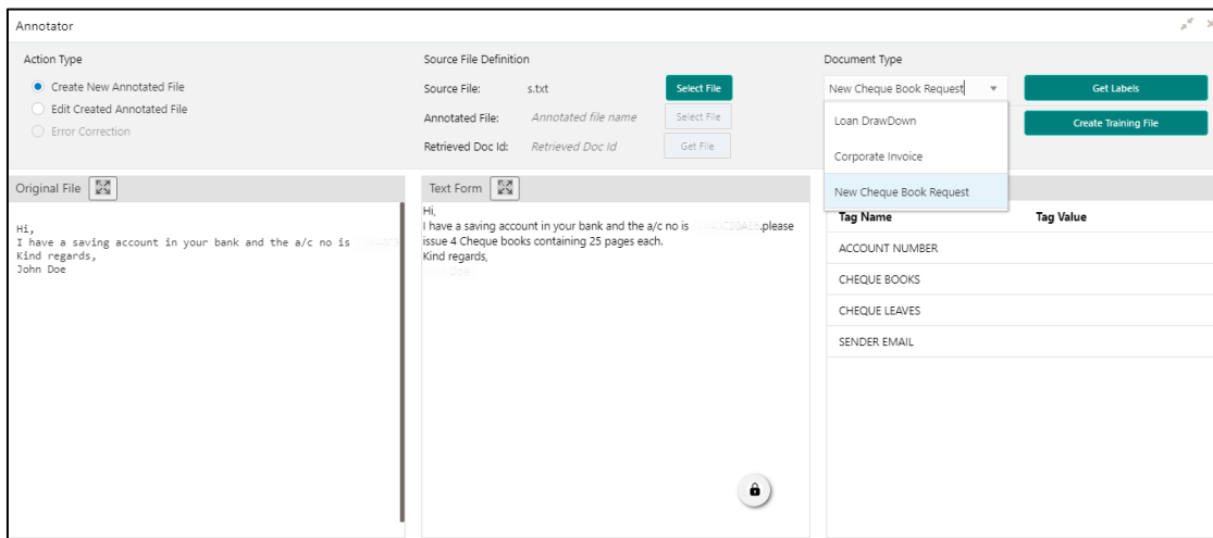
Figure 237: Annotator
