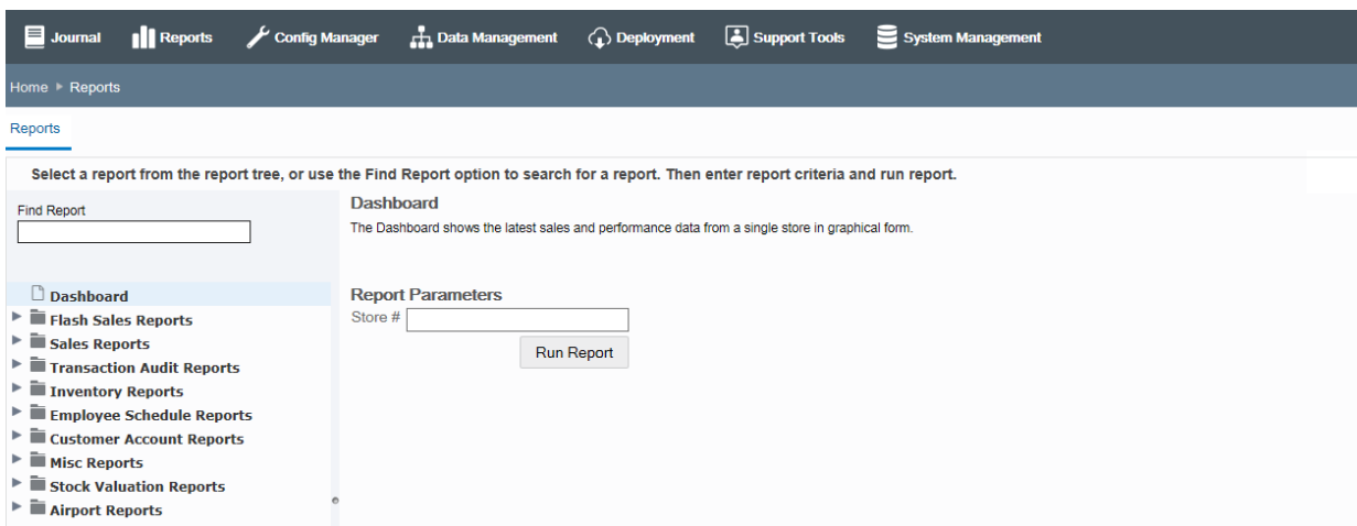
Figure 9–3 Reports - Dashboard
