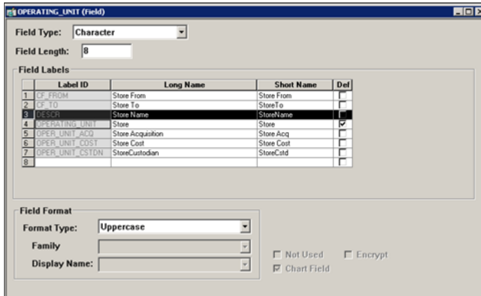
Application Designer: Field dialog box
