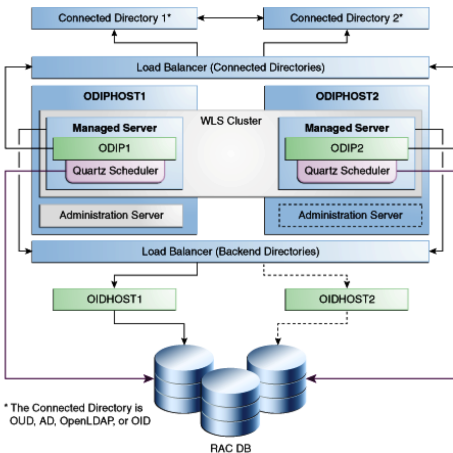
Figure 12-2 Oracle Directory Integration Platform with Oracle Internet Directory (Back-End Directory) in a High Availability Architecture
