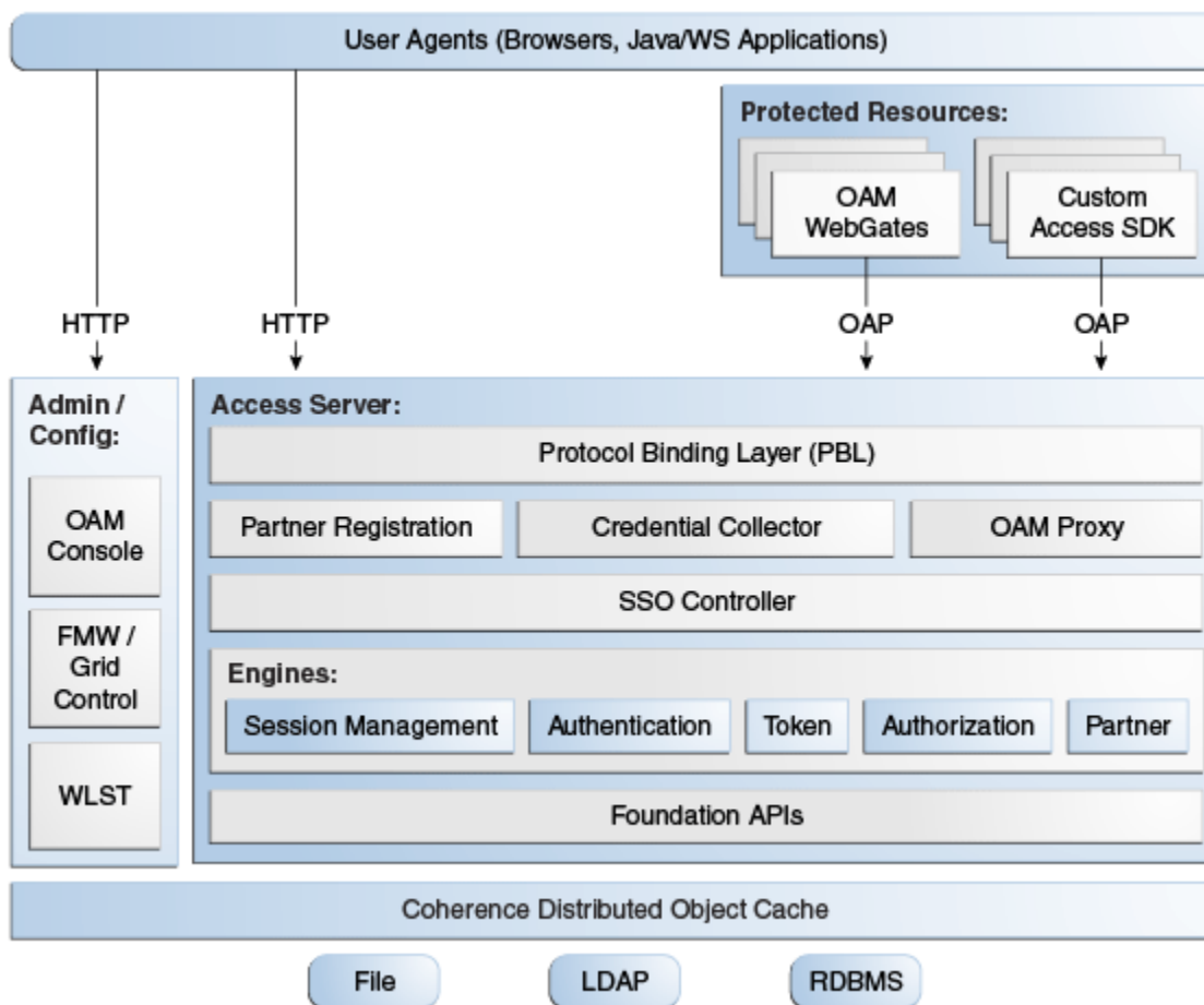
Figure 11-1 Access Manager Single Instance Architecture
