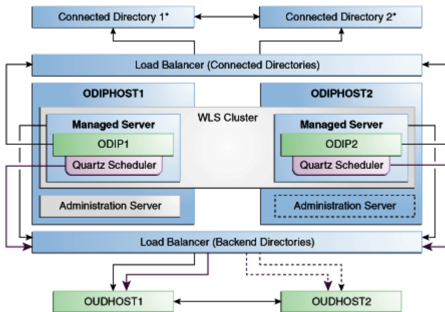
Figure 12-3 Oracle Directory Integration Platform with Oracle Unified Directory (Back-End Directory) in a High Availability Architecture
