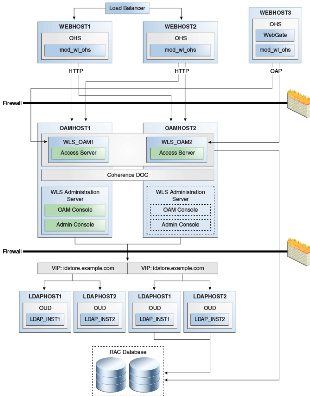
Figure 11-2 Access Manager High Availability Architecture
