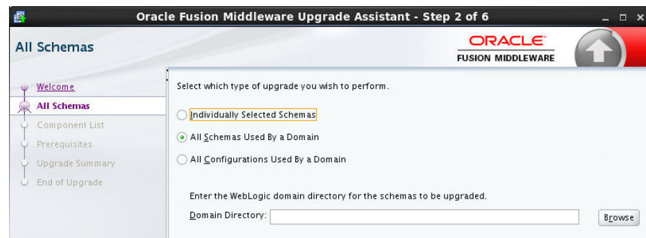
Figure 4-1 Upgrade Assistant: All Schemas Screen
