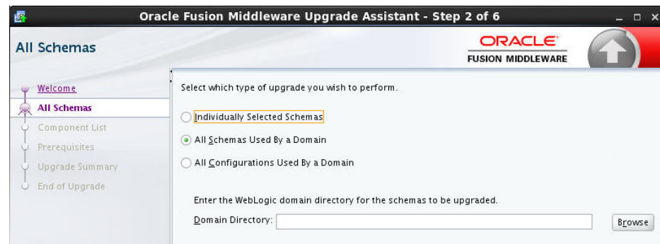
Figure 6-1 Upgrade Assistant: All Schemas Screen
