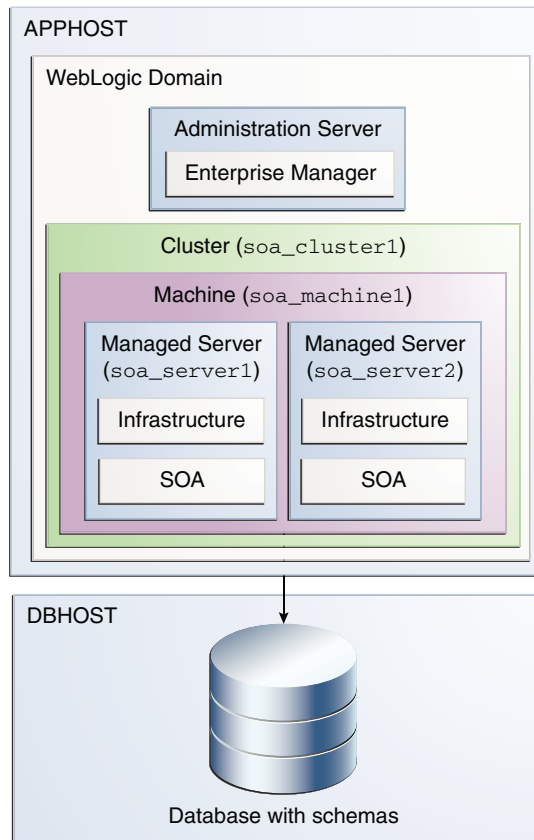
Figure 1-1 Standard Topology for Oracle B2B
