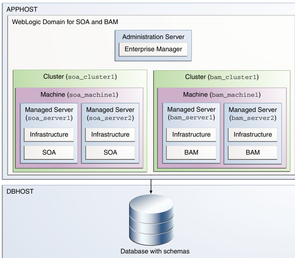
Figure 1-3 BAM Standard Installation Topology
