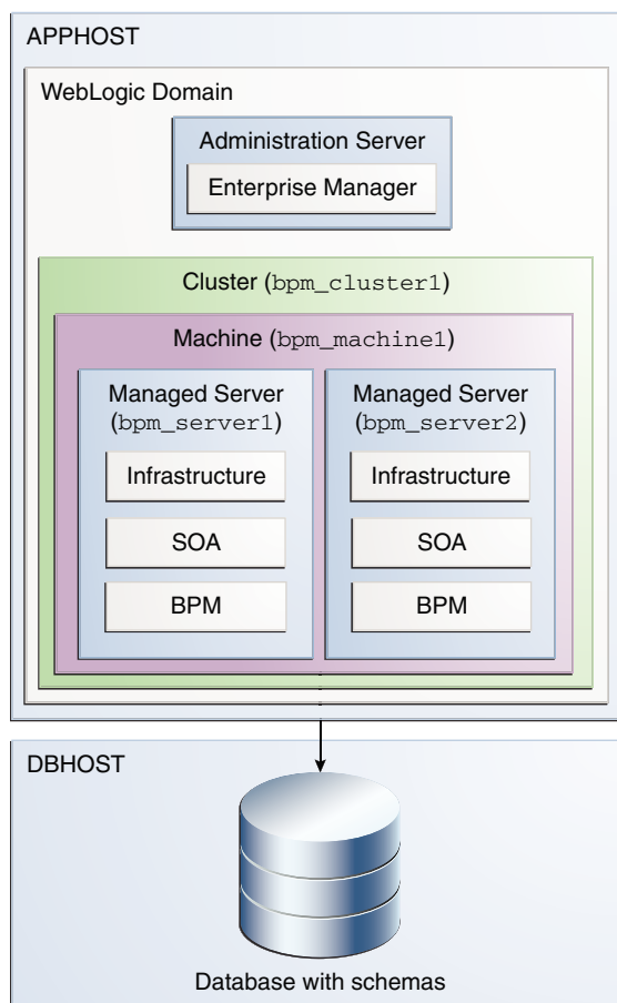
Figure 1-2 BPM Standard Installation Topology
