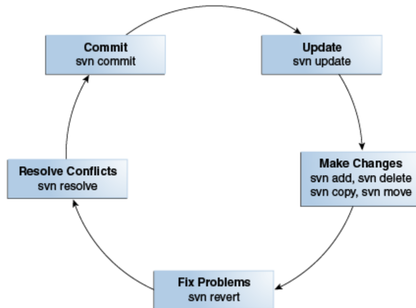
Figure 3-1 SVN Workflow
