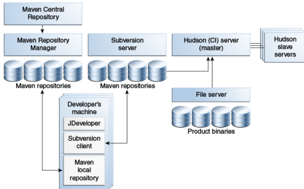
Figure 2-1 Reference Continuous Integration Environment Architecture
