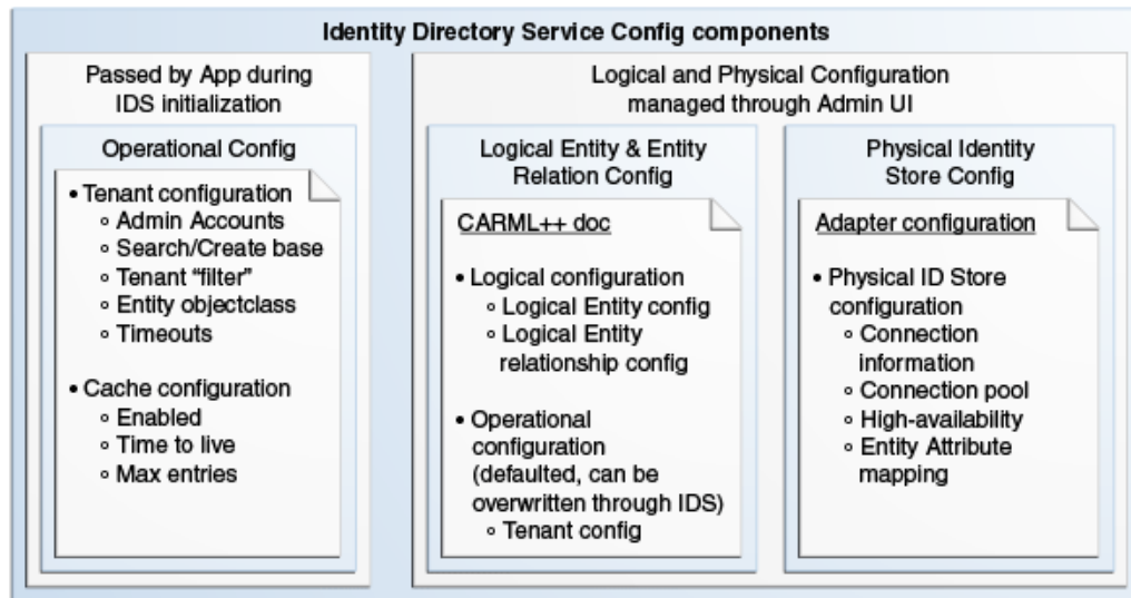
Figure 2-2 Identity Directory API Components
