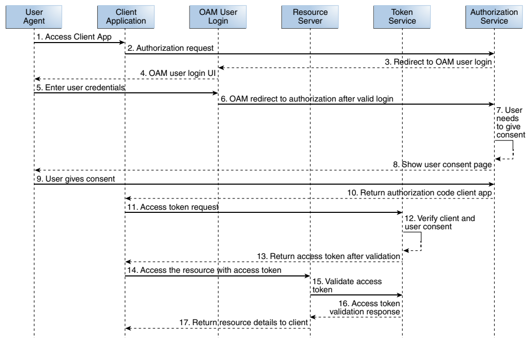
Figure 37-1 OAuth 3-Legged Flow Diagram
