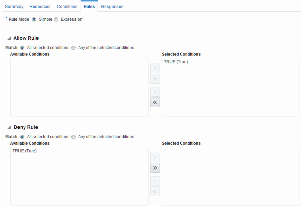
Figure 25-27 Authorization Policy Rules Tab: Simple Mode
