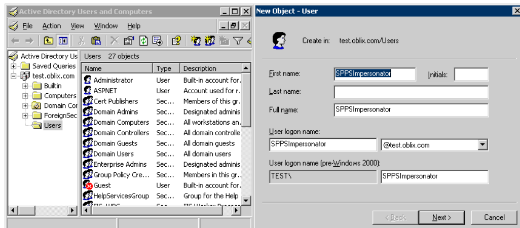
Figure 50-1 Setting up a Trusted User Account for Windows Impersonation
