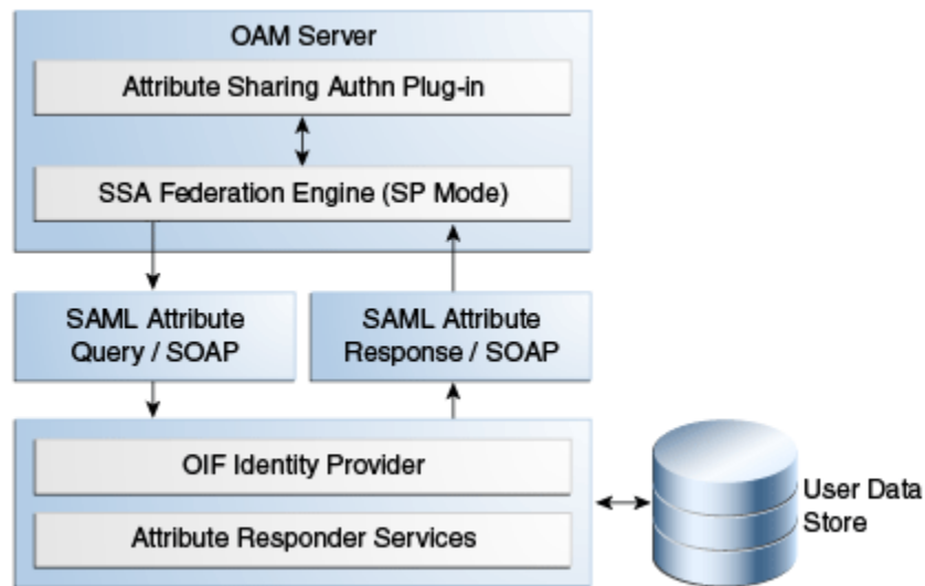
Figure 30-4 Attribute Sharing Plug-in Design
