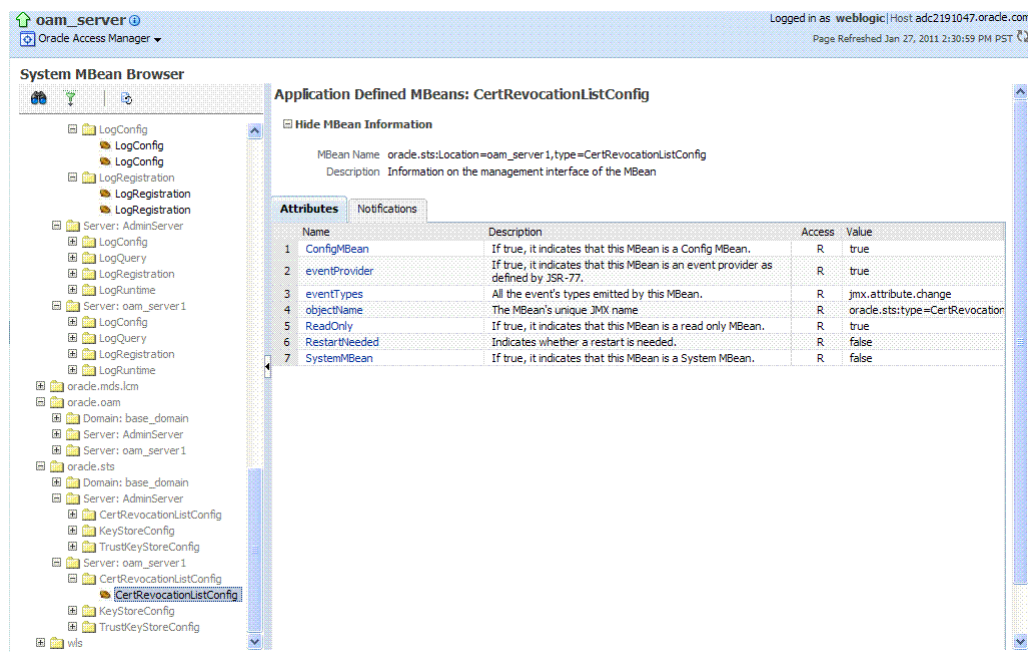
Figure 12-18 System MBean Browser and Attributes Tab
