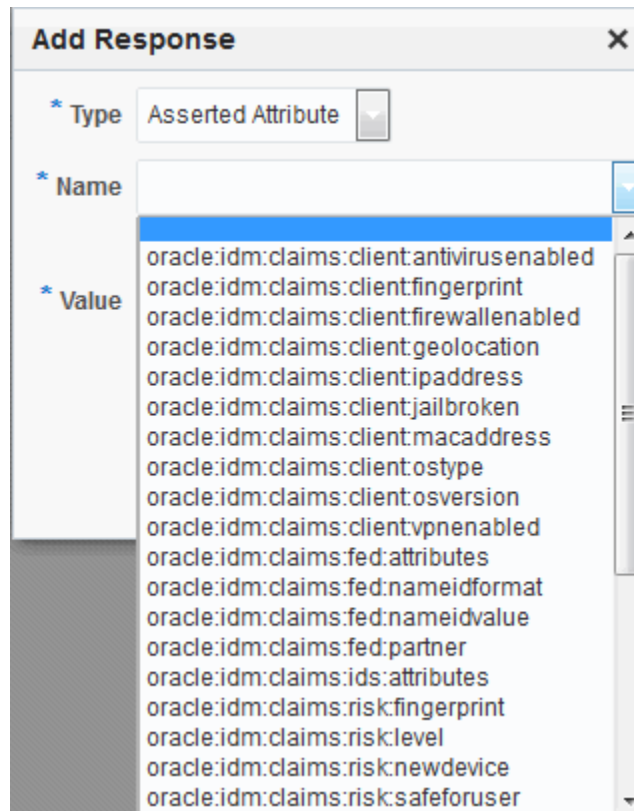
Figure 32-8 Adding a Federation Response Attribute to an AuthZ Policy
