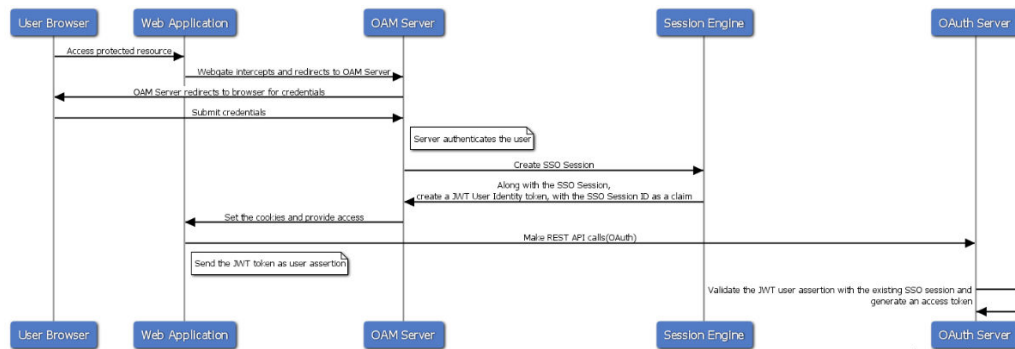
Figure 38-3 Use case flow for SSO Session Linking for OAuth Tokens
