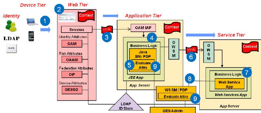
Figure 42-3 Identity Context Process Flow
