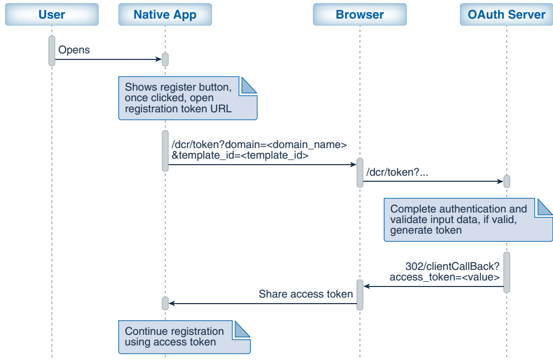
Figure 38-1 Diagram Showing the Flow for Getting Registration Token
