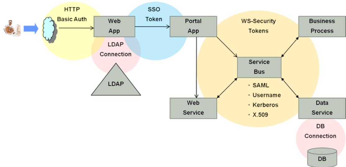
Figure 42-1 End to End Identity Context Process
