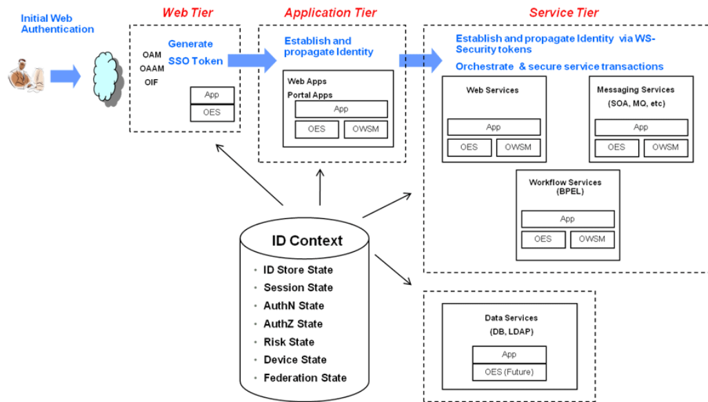
Figure 42-2 End To End Identity Context Process Components
