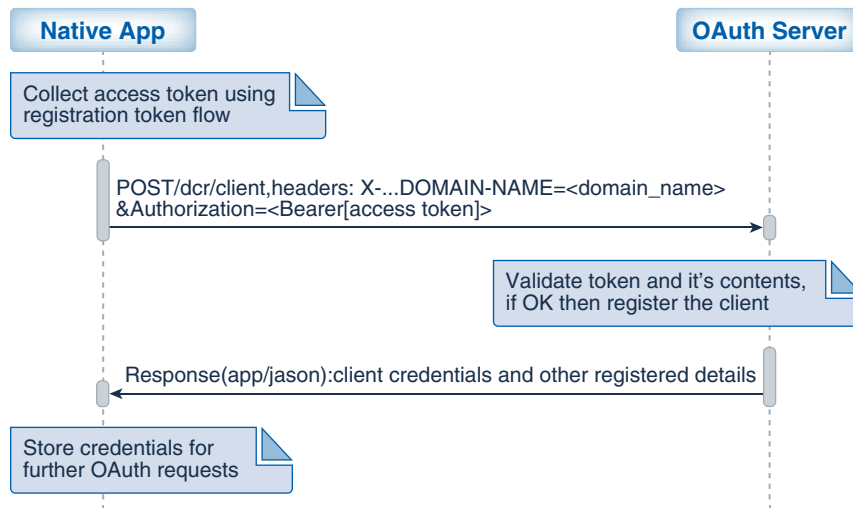
Figure 38-2 Diagram Showing the Flow for Client Registration
