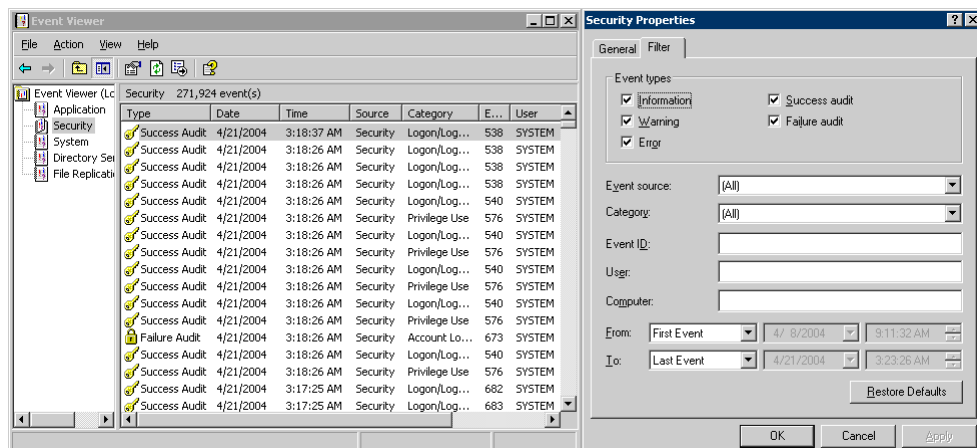
Figure 50-3 Verifying Event Viewer Settings
