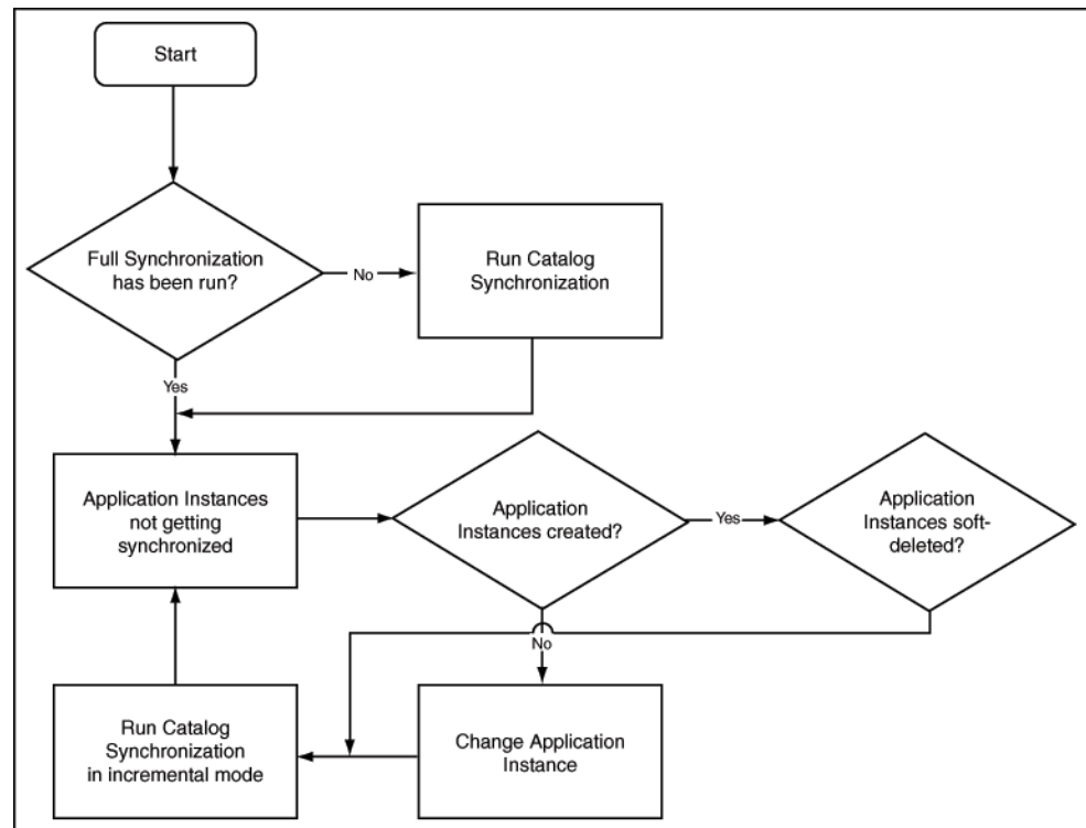
Figure 12-4 Trouble Shooting Synchronization Application Instances Flowchart
