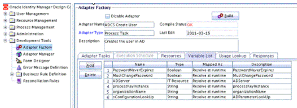
Figure 10-24 The Variable List Tab of the Adapter Factory Form
