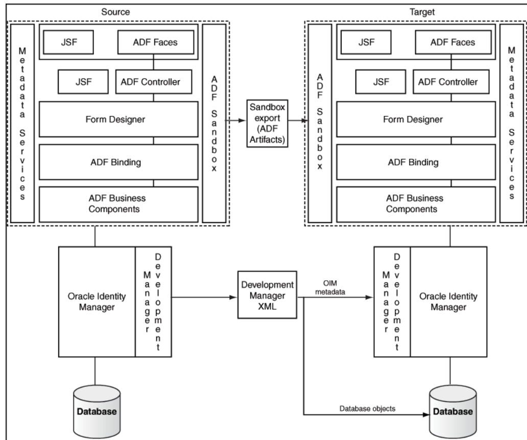
Figure 12-2 Test to Production Process for Catalog
