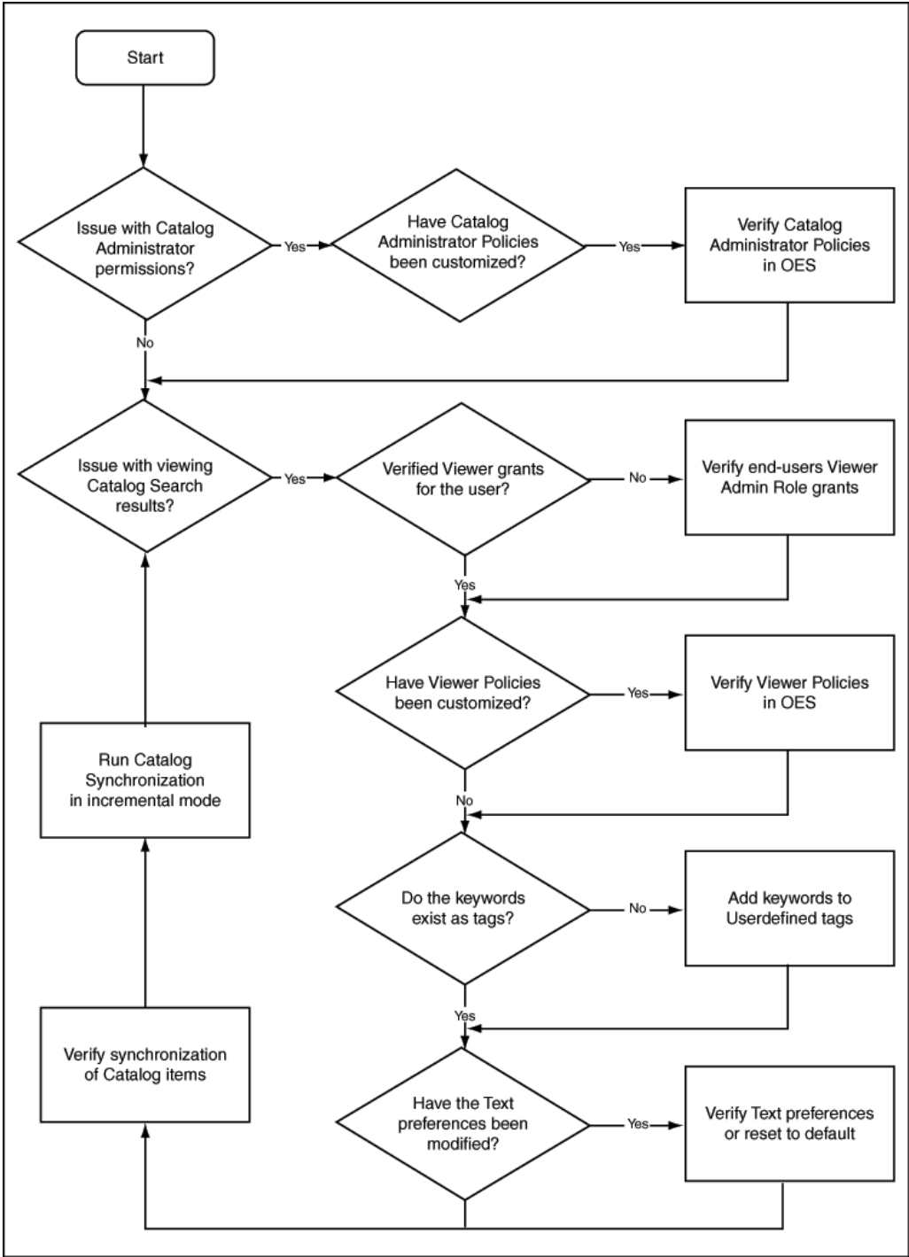
Figure 12-6 Diagnostic Flowchart With Security Issues
