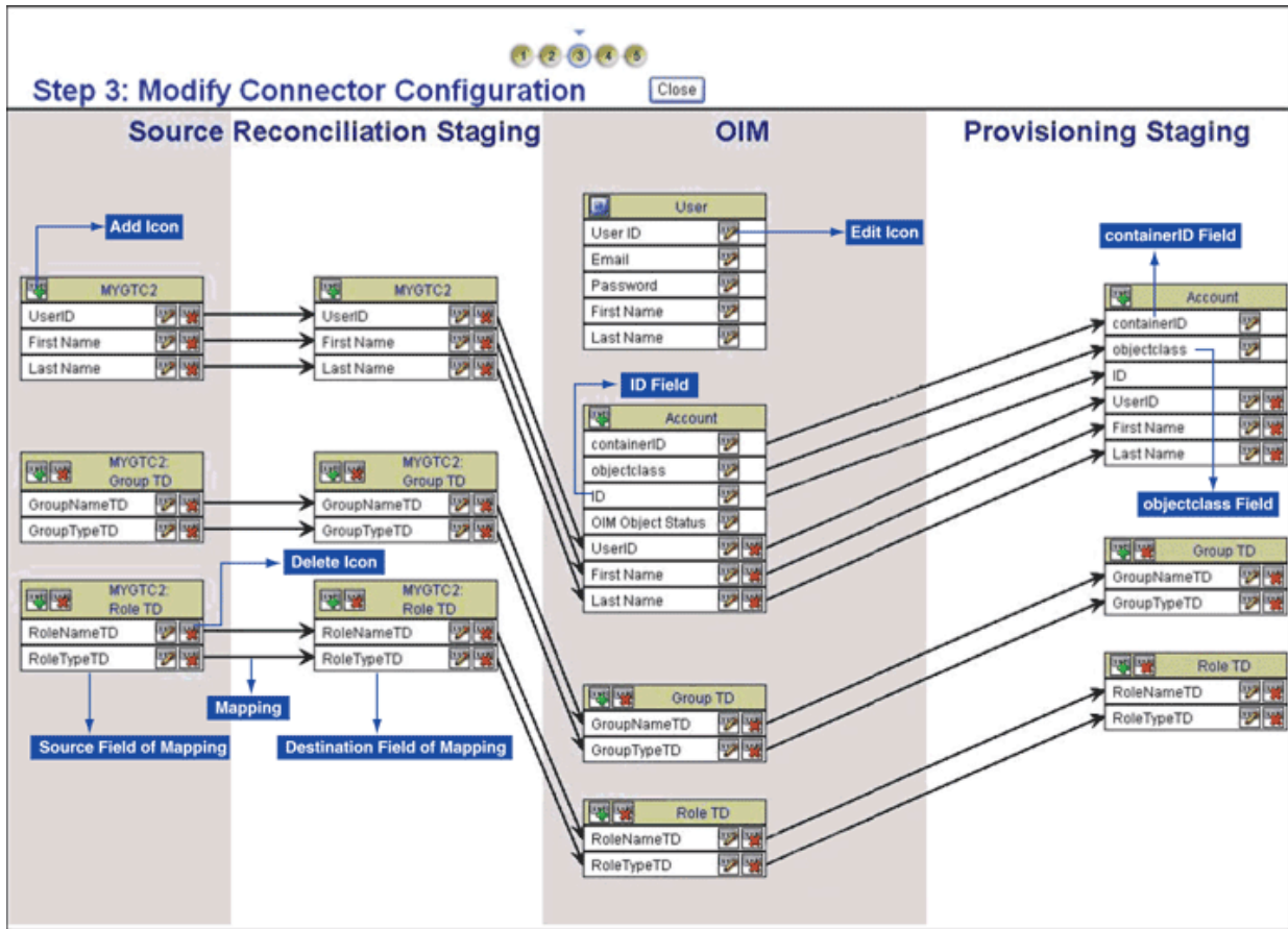
Figure 8-1 Step 3: Modify Connector Configuration Page
