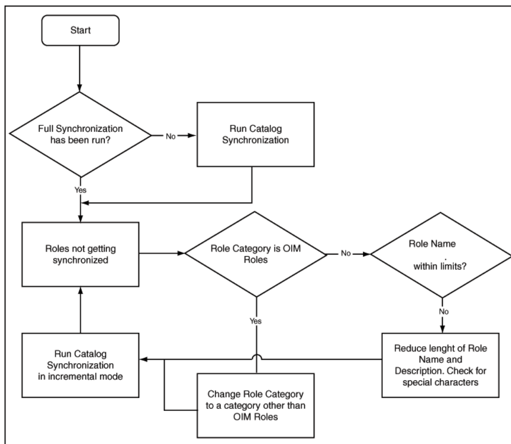
Figure 12-3 Catalog Synchronization Diagnostic Flowchart
