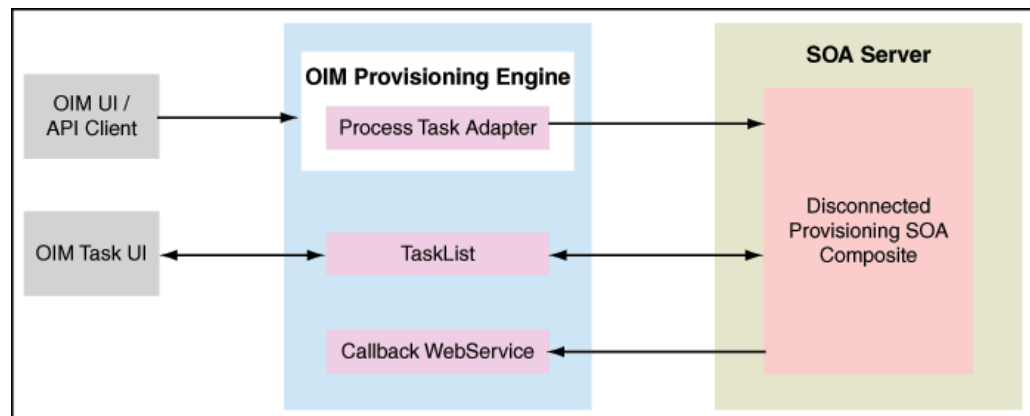
Figure 9-3 Disconnected Resource Architecture
