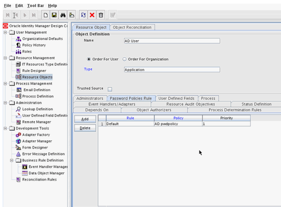
Figure 9-2 Attach Password Policy to Application Instance
