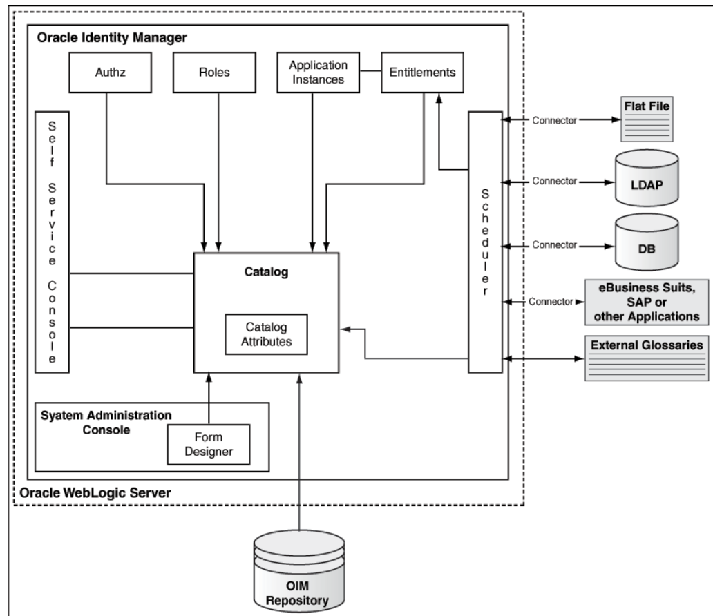
Figure 12-1 High-Level Catalog Architecture
