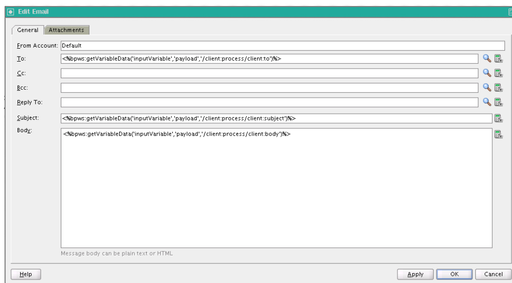
Figure 18-3 Sample Mapping of Composite Payload
