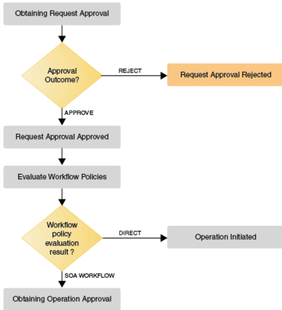
Figure 4-5 In-Flight Requests Awaiting Request Approval
