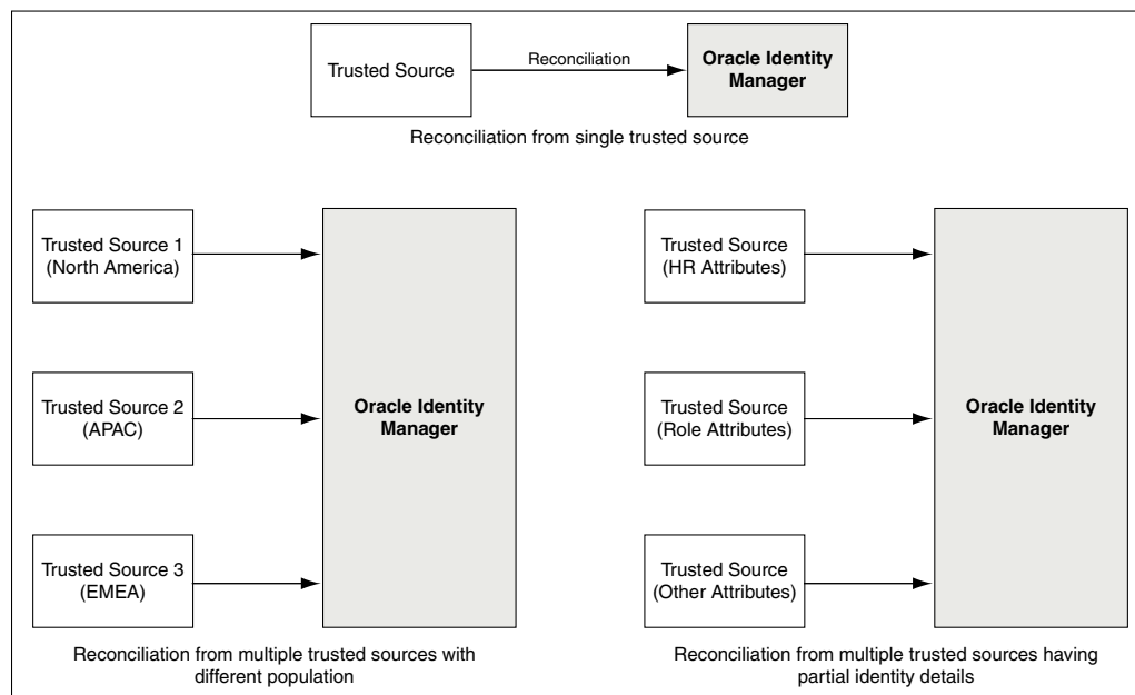
Figure 11-2 Trusted Source Reconciliation from Single and Multiple Authoritative Sources
