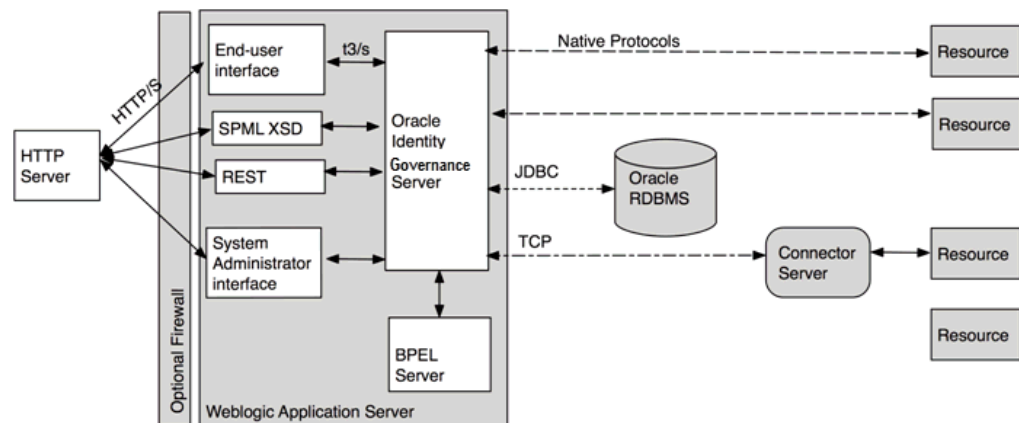
Figure 2-1 Oracle Identity Governance Components
