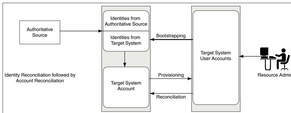
Figure 11-4 Identity and Account Reconciliation
