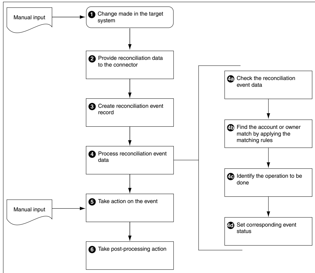
Figure 11-5 Reconciliation Process Flow
