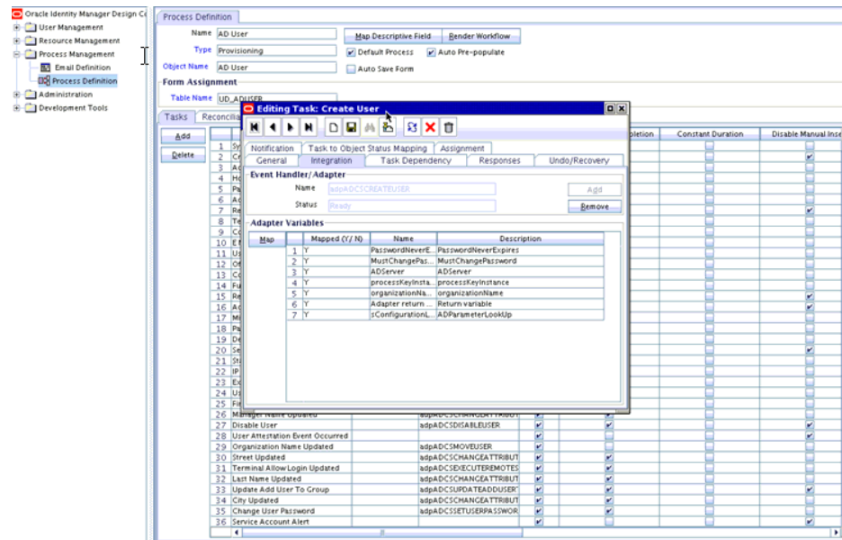
Figure 10-26 The Integration Tab of the Editing Task Dialog Box
