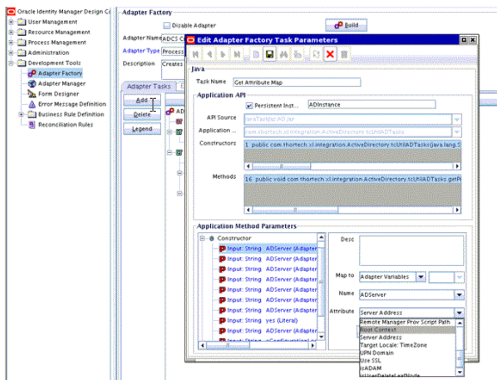
Figure 10-25 The Edit Adapter Factory Task Parameters Dialog Box
