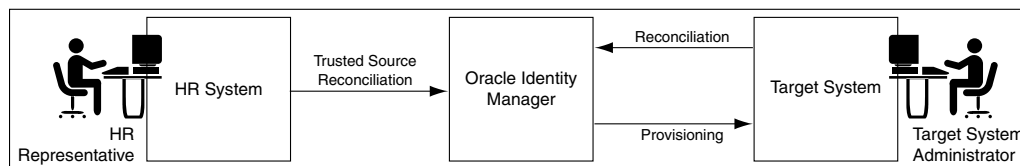
Figure 11-1 Provisioning and Reconciliation
