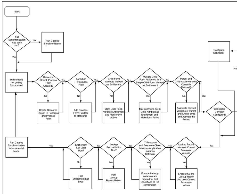
Figure 12-5 Troubleshooting Synchronizing Entitlements Flowchart
