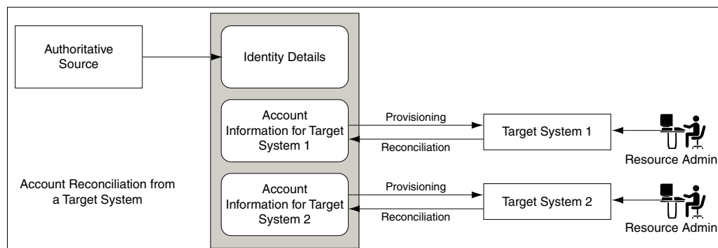
Figure 11-3 Account Reconciliation From a Target System
