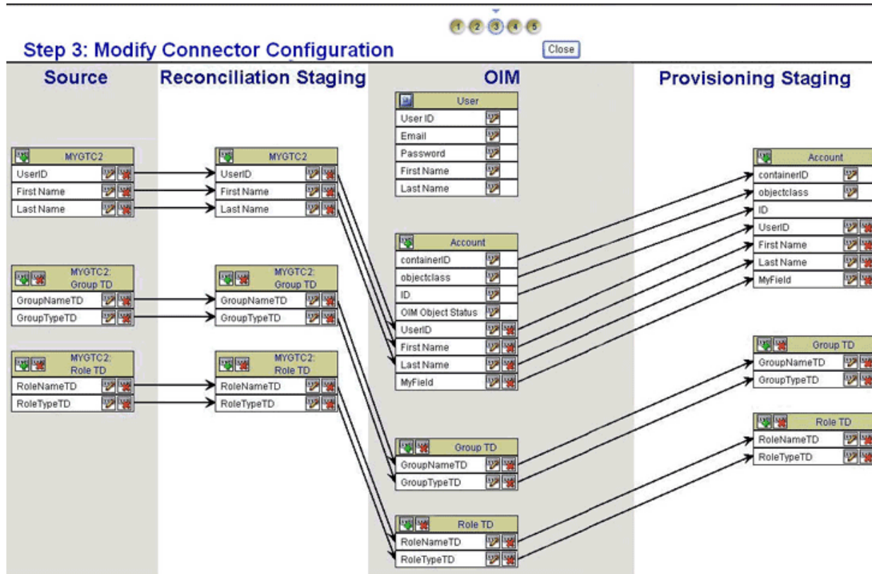
Figure 8-2 Step 3: Modify Connector Configuration Page After Addition of a Field
