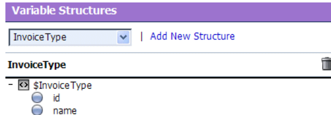
Figure 13-5 Variable Structures—InvoiceType
