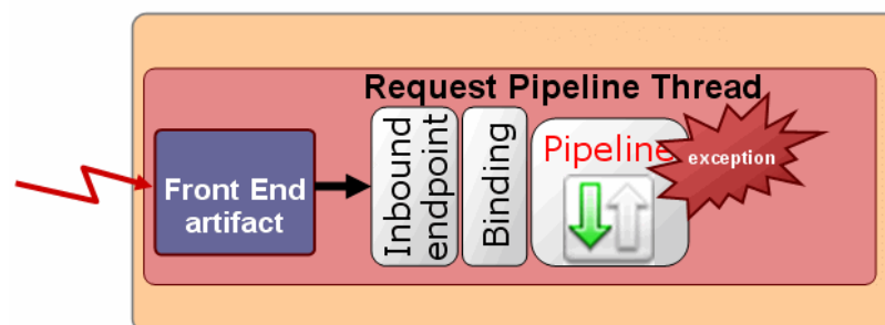
Figure 40-2 Error Case 1
