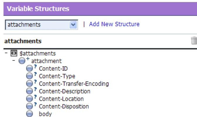
Figure 13-9 Variable Structures—attachments
