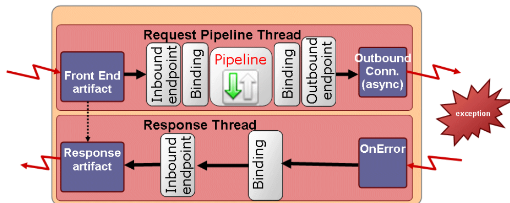
Figure 40-3 Error Case 2
