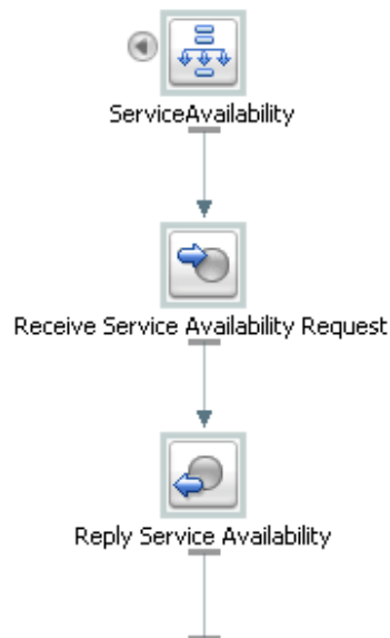
Figure 10-5 New Split-Join
