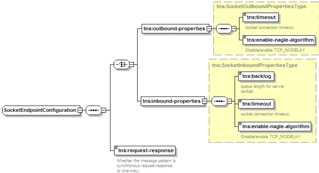
Figure 43-2 SocketEndpointConfiguration Properties
