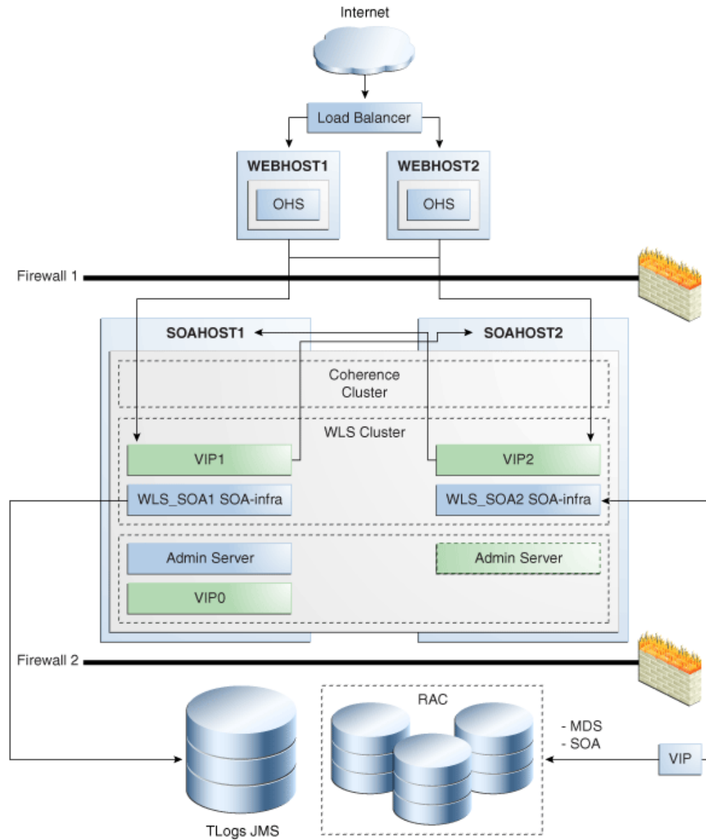
Figure C-1 Oracle SOA Service Infrastructure High Availability Architecture
