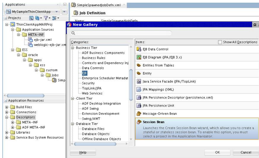
Figure 6-17 New Gallery Dialog
