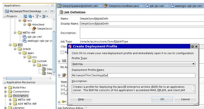
Figure 6-12 Create Deployment Profile Dialog
