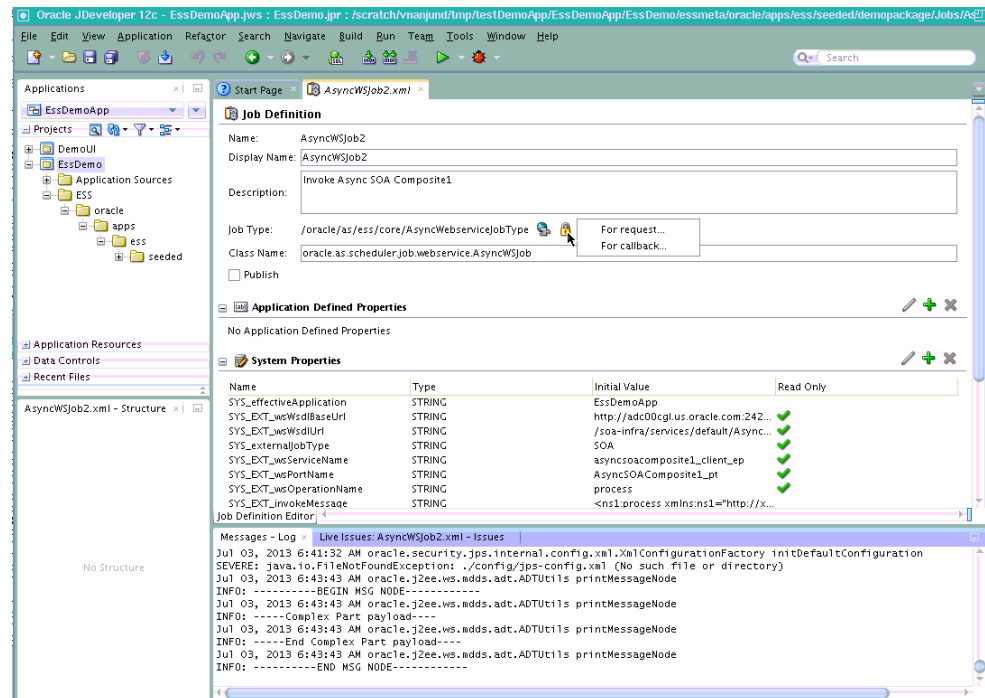
Figure 13-3 Oracle JDeveloper: Job Definition Tab
