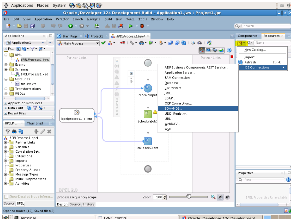
Figure 16-4 Creating a Connection to the Metadata Server
