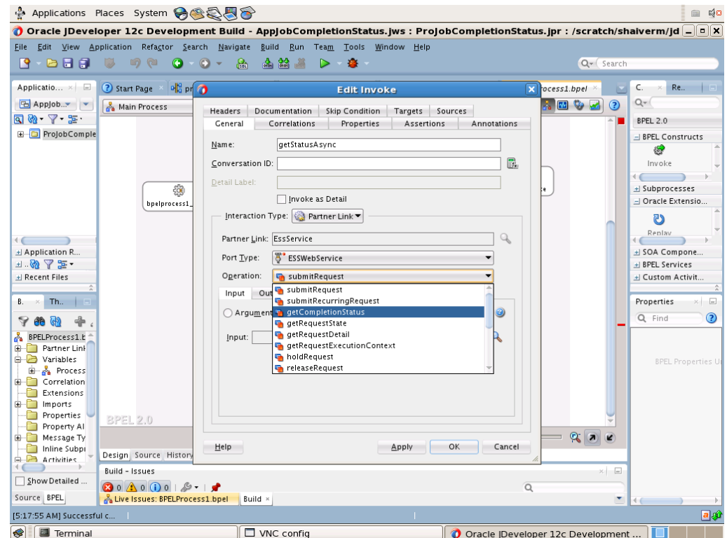
Figure 16-16 The Edit Invoke Dialog
