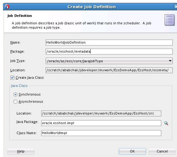
Figure 7-4 Creating a Job Definition with the Job Definition Creation Wizard
