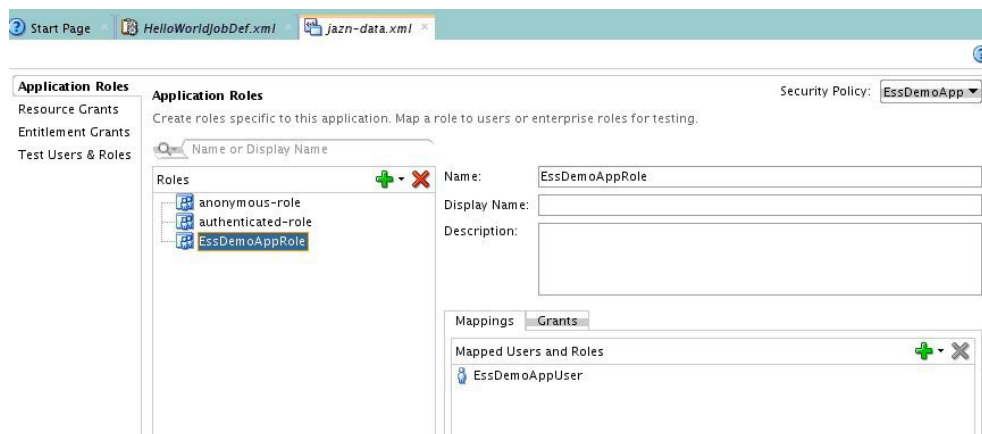
Figure 7-17 Configuring Security
