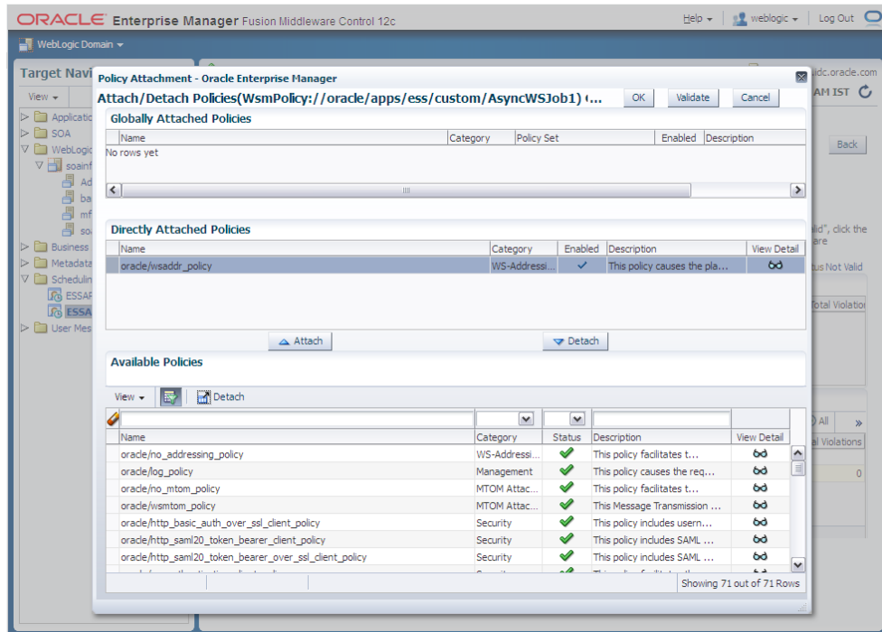
Figure 13-10 Fusion Middleware Control Console: Policy Attachment Popup
