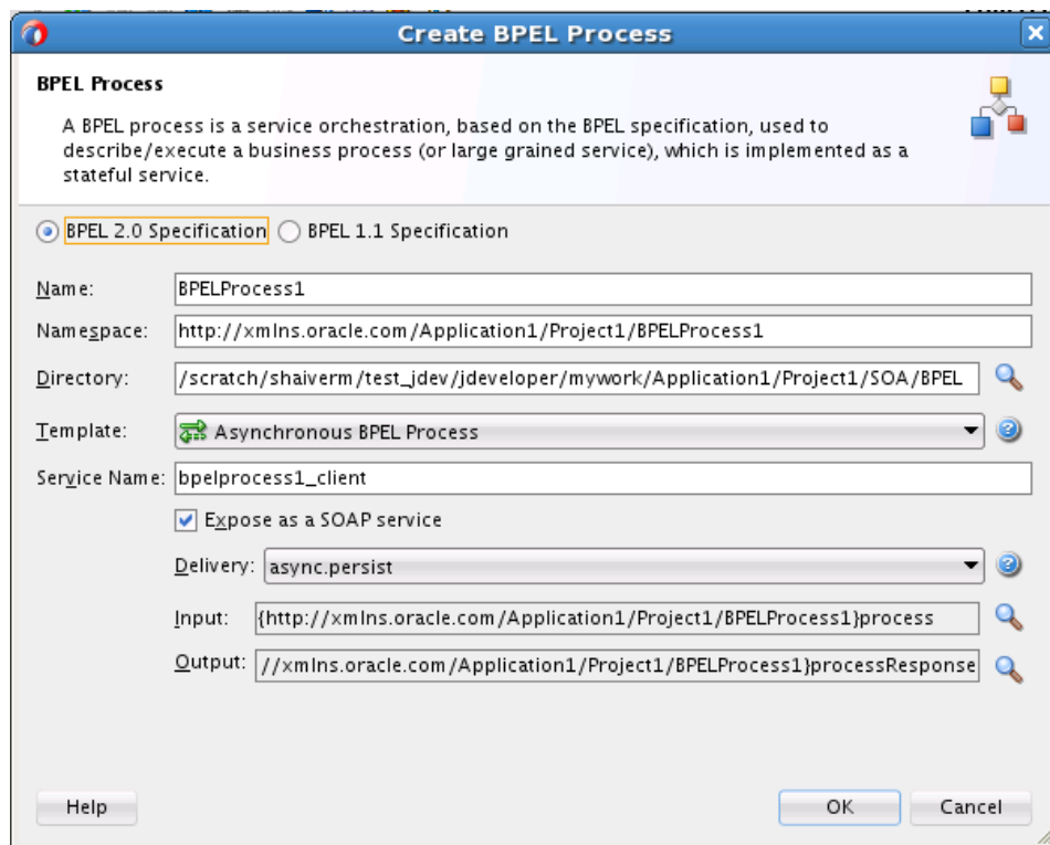
Figure 16-1 Choose a BPEL Specification
