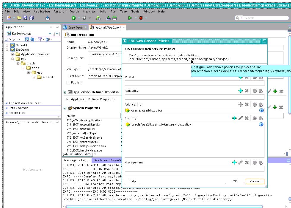
Figure 13-5 Oracle JDeveloper: ESS Web Service Policies Popup
