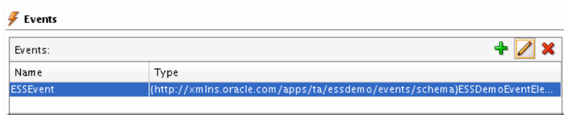
Figure 21-10 Events List
