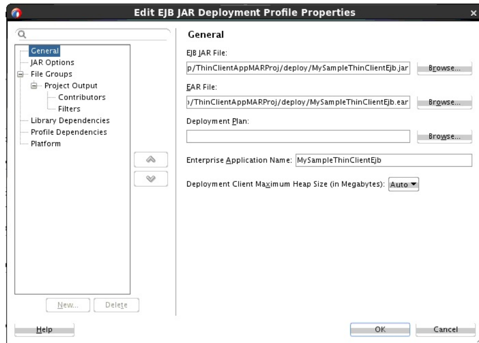
Figure 6-13 Create the EJB-JAR Deployment Profile
