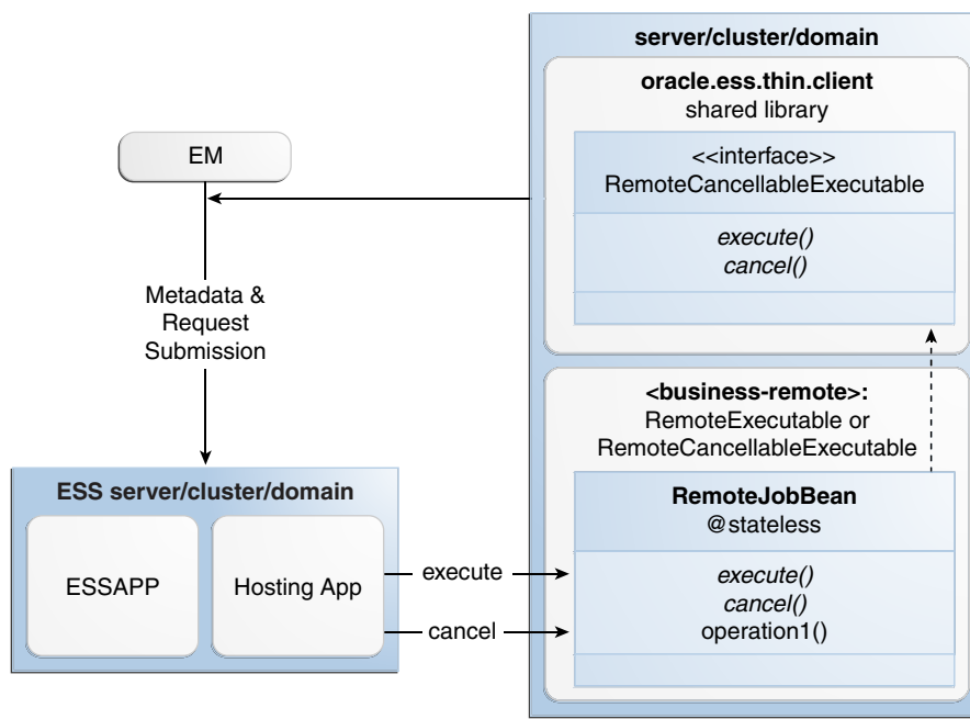
Figure 12-1 EJB Job Environment
