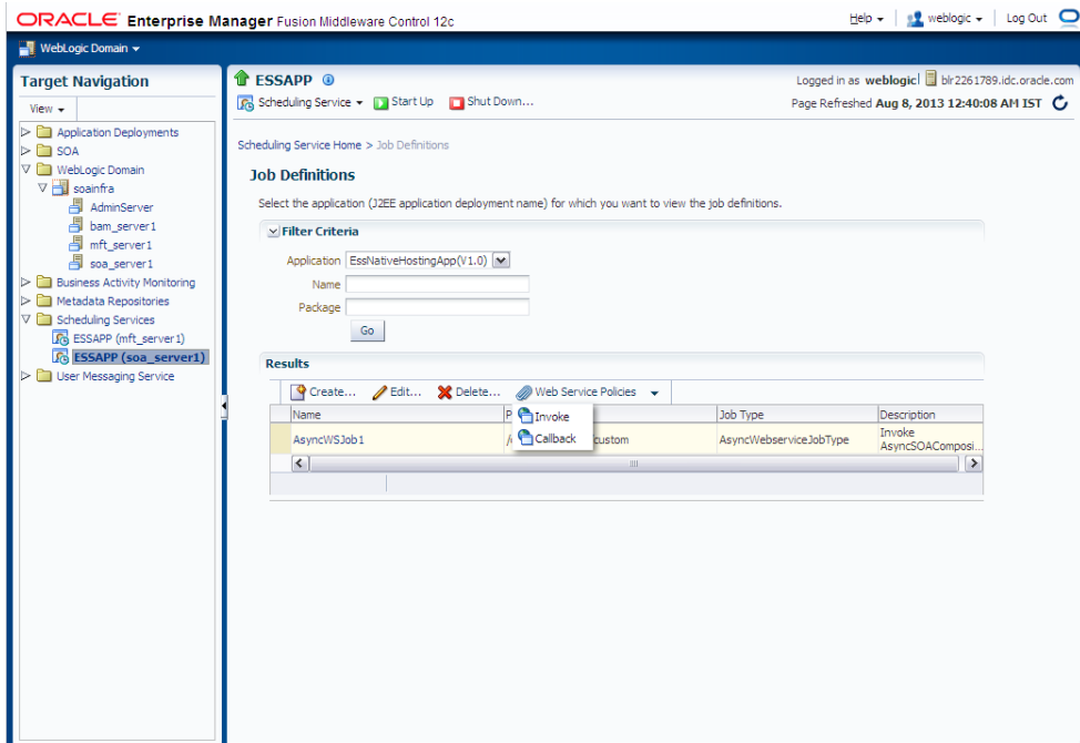
Figure 13-8 Fusion Middleware Control Console: Job Definitions Page
