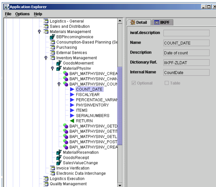
Figure 1-12 Application Explorer
