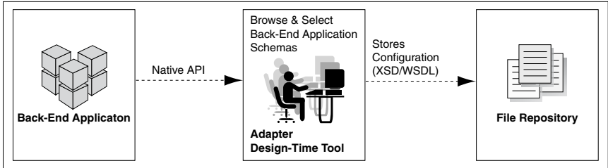
Figure 1-18 Metadata Service
