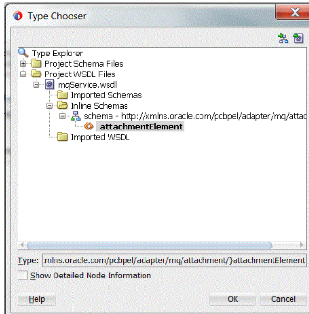
Figure 10-105 Selecting attachmentElement
