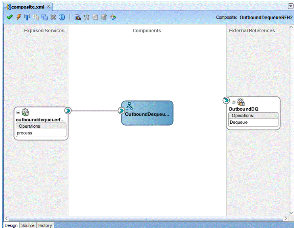
Figure 10-100 The JDeveloper-composite.xml
