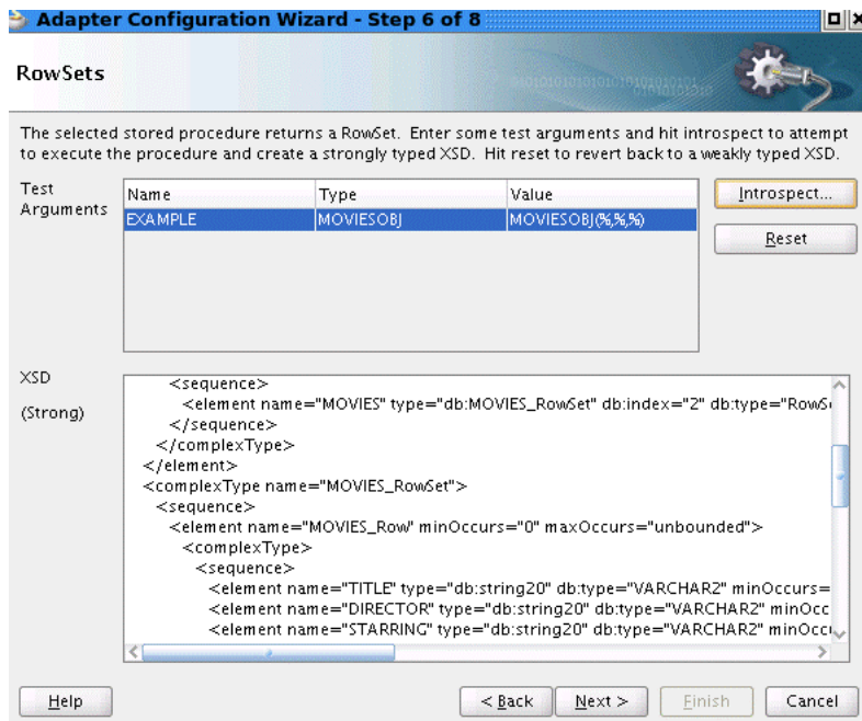
Figure 9-51 RowSets Page
