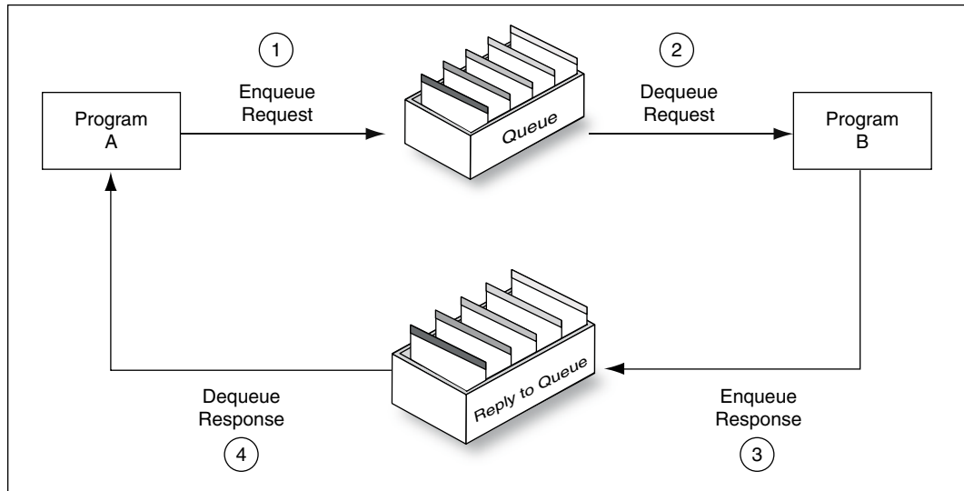
Figure 10-2 Request/Response Interaction
