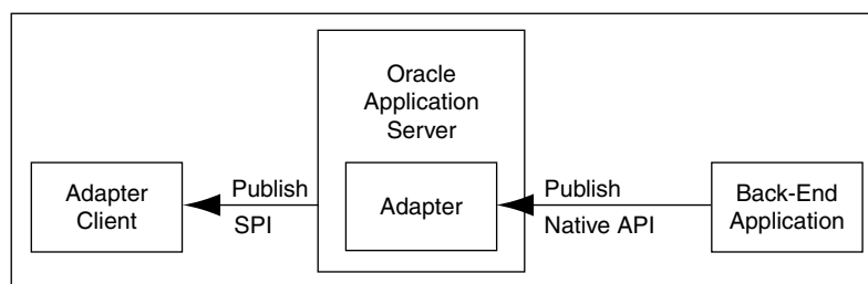
Figure 1-17 Event-Notification Service
