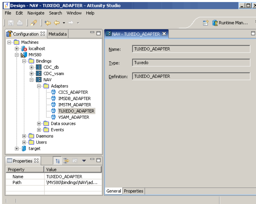
Figure 1-8 Oracle Studio
