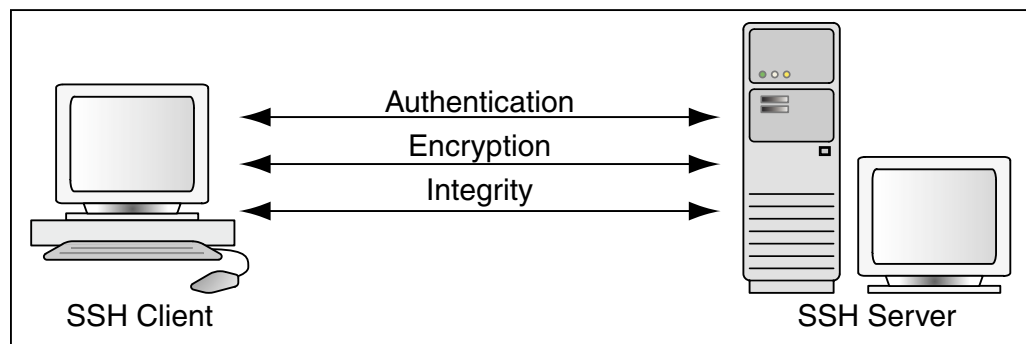
Figure 5-52 SFTP Communication
