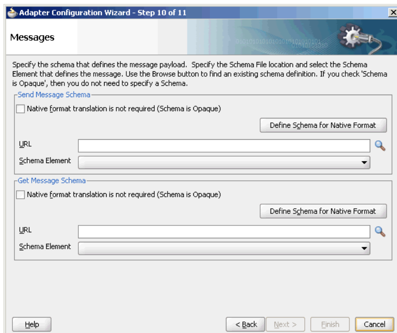
Figure 10-16 Messages Page
