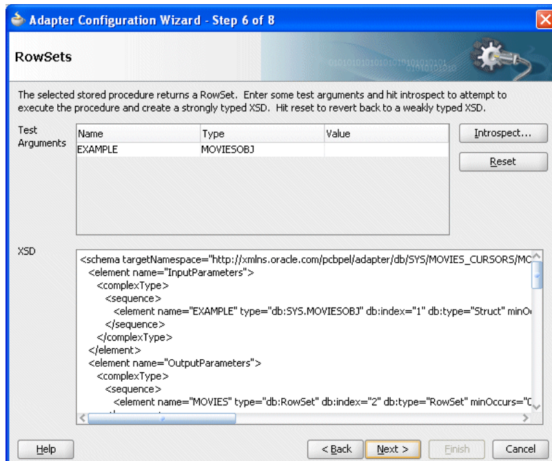
Figure 9-56 RowSets Page
