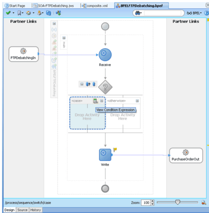
Figure 5-162 BPELFTPDebatching.bpel Page
