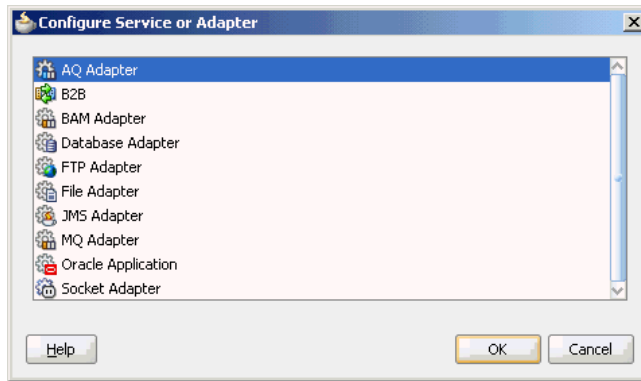
Figure 3-7 Adapter Types
