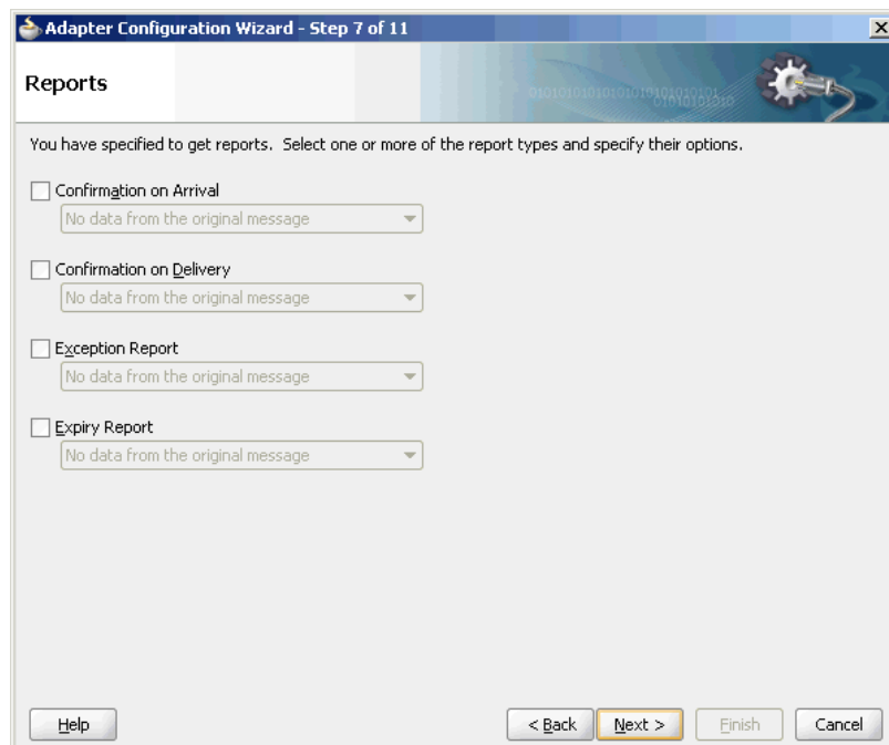
Figure 10-14 Reports Page
