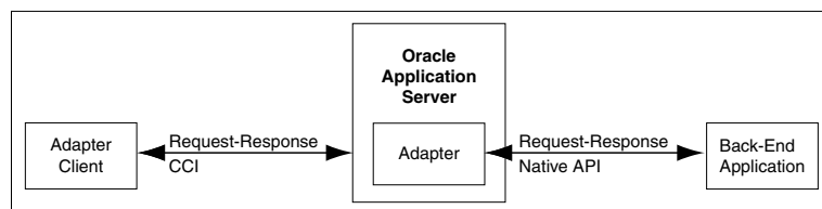
Figure 1-16 Request-Response Service
