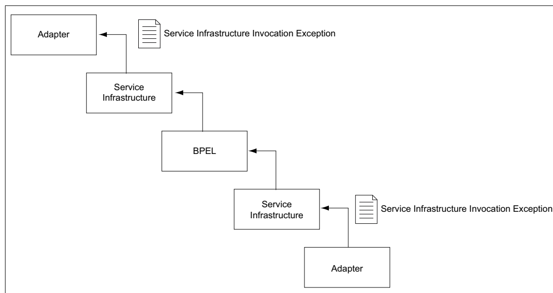
Figure 2-13 Fault Propagation
