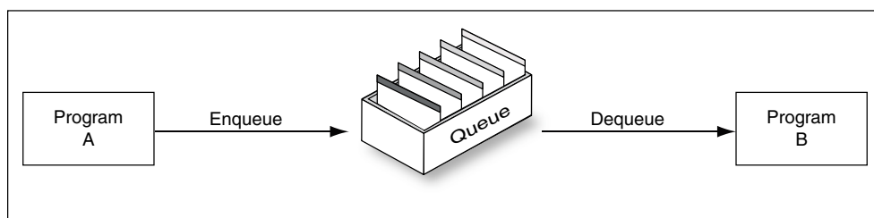
Figure 10-1 Enqueue/Dequeue
