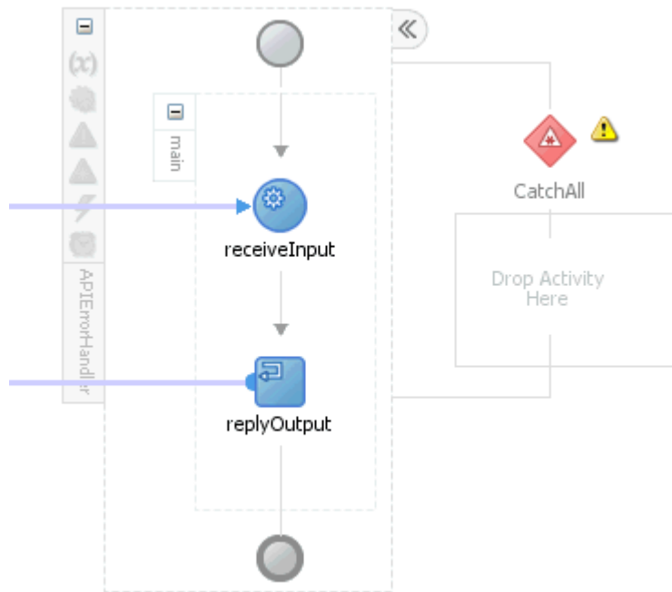
BPEL Diagram with the CatchAll Activity Added
