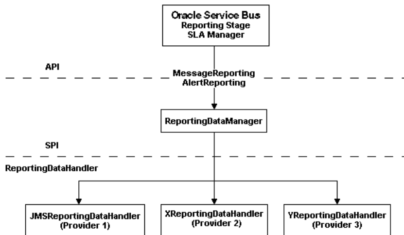
Figure 13-1 Reporting Framework
