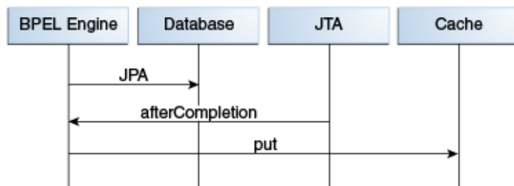
Figure 18-1 Dehydration Process
