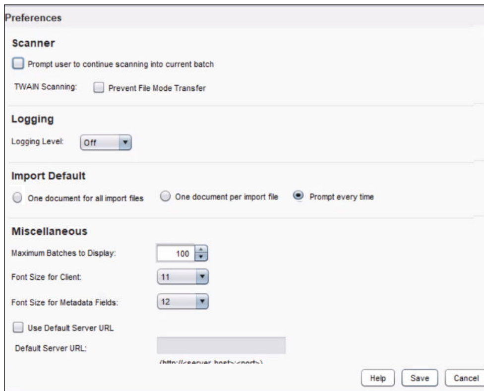
Figure 1-5 Preferences Window
