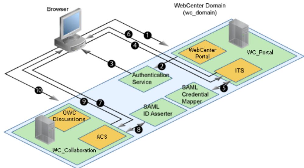
Figure 27-4 SAML Single Sign-on Components and Topology (POST Profile Configured)
