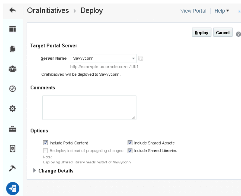
Figure 33-2 Deploying a Portal
