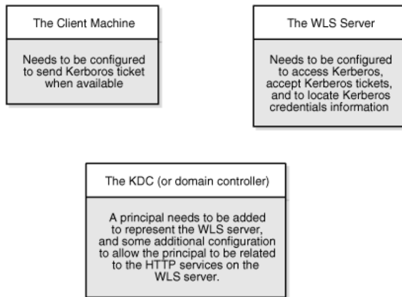
Figure 27-17 Configuring SSO with Microsoft Clients
