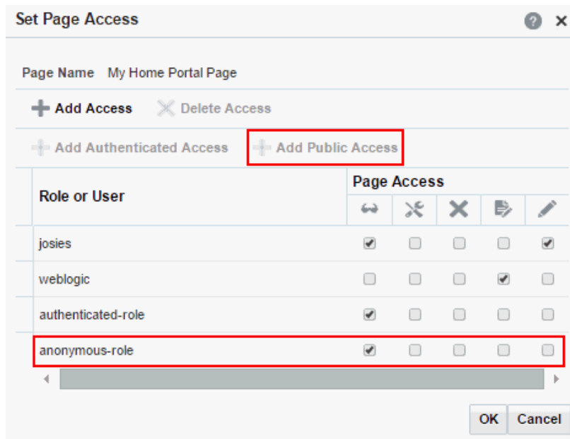
Figure 43-3 Anonymous Role Access
