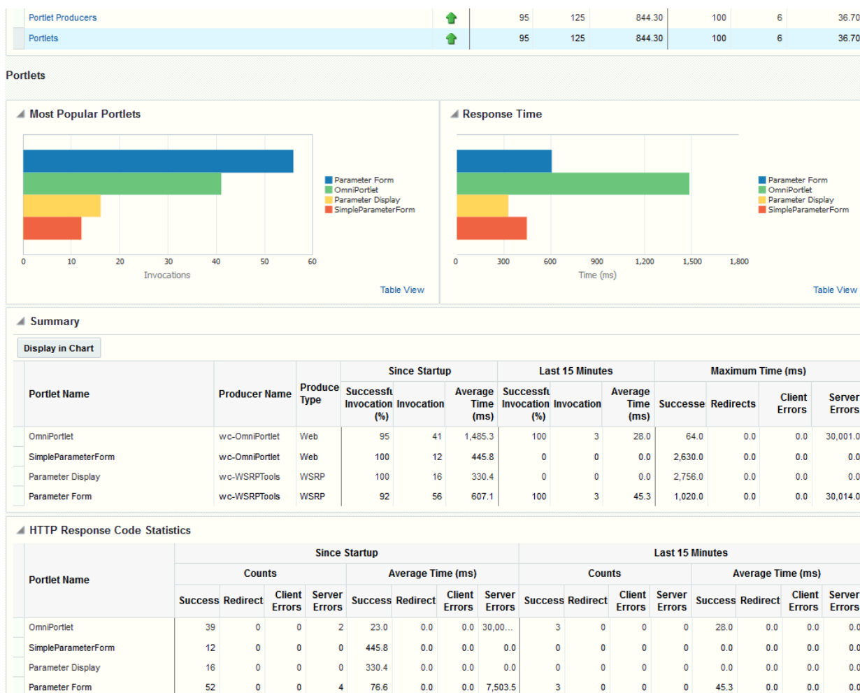
Figure 21-8 Portlet Metrics
