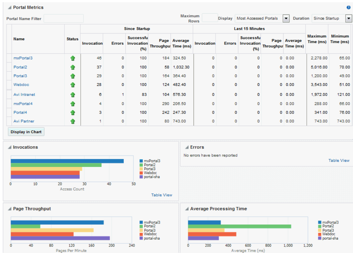
Figure 21-13 Portal Metrics
