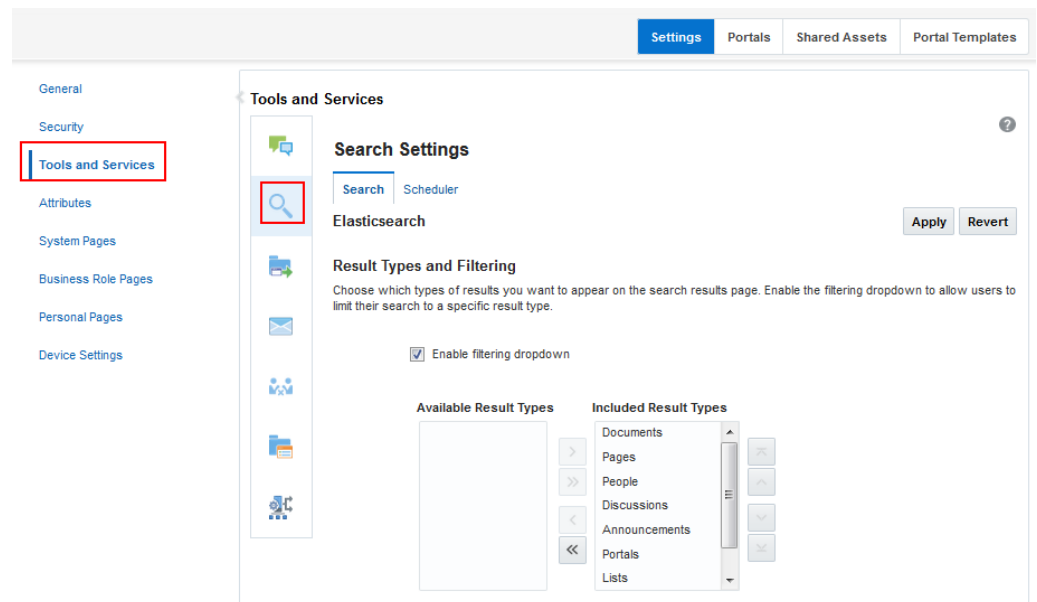
Figure 10-22 Elasticsearch Settings
