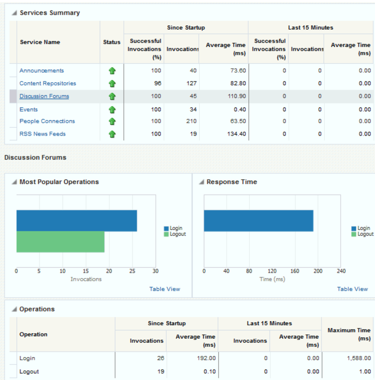
Figure 21-17 Discussion Metrics
