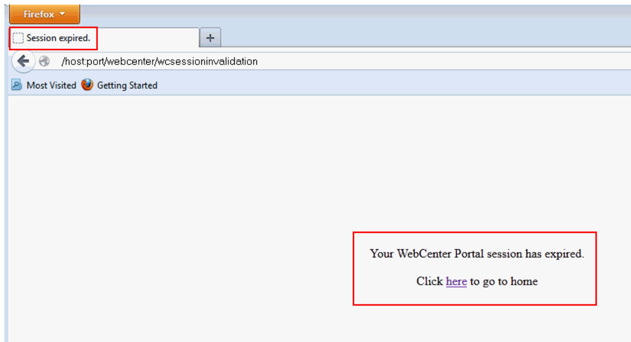
Figure 38-21 Timeout Page
