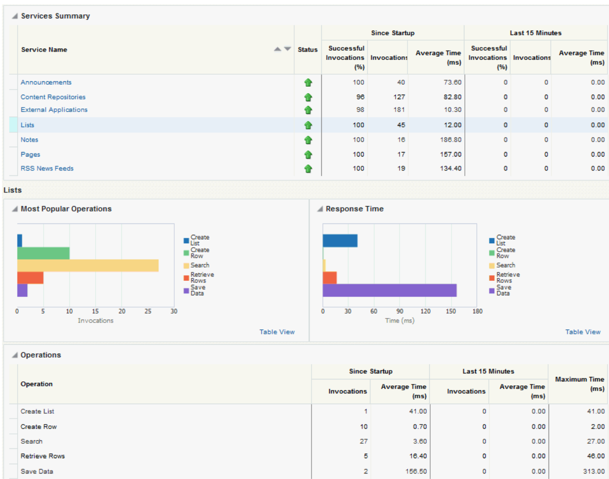
Figure 21-22 List Metrics
