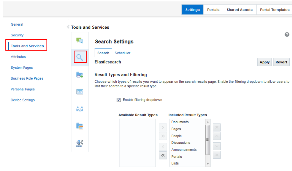
Figure 10-8 Elasticsearch Settings
