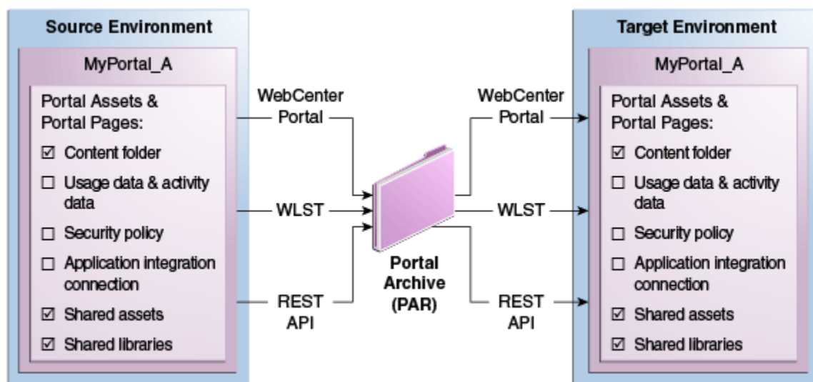
Figure 33-7 Deploying Portal Archives
