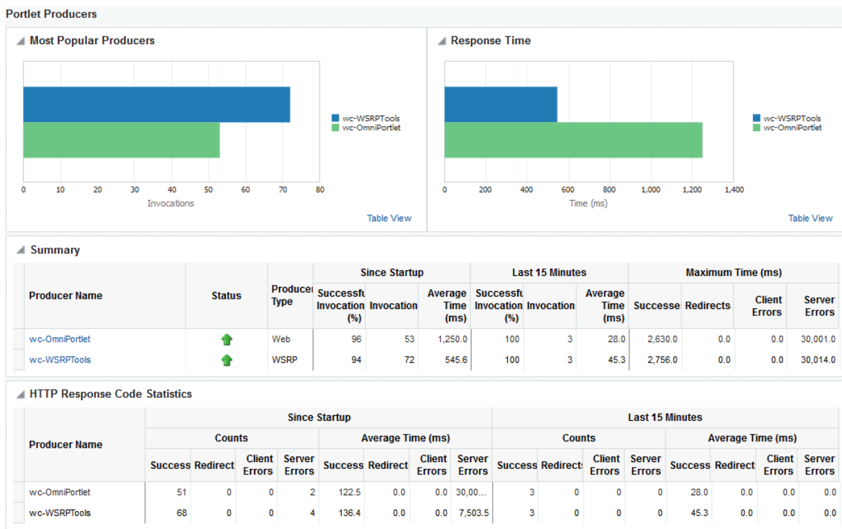
Figure 21-7 Portlet Producer Metrics
