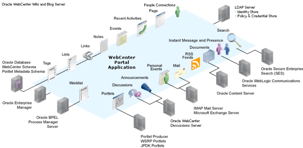
Figure 24-2 WebCenter Portal Application Architecture with Back-End Server Connections
