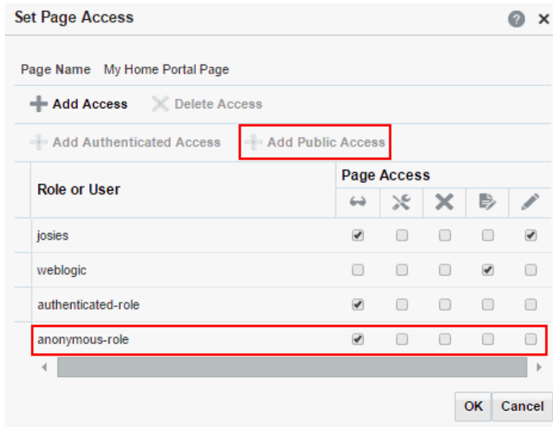
Figure 42-6 Anonymous Role Access
