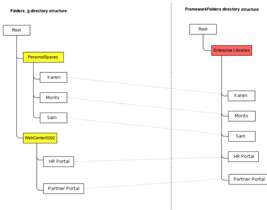
Figure F-1 Folders_g and FrameworkFolders Folder Structure on Content Server
