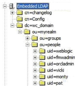
Figure 25-1 Embedded LDAP Directory Information Tree
