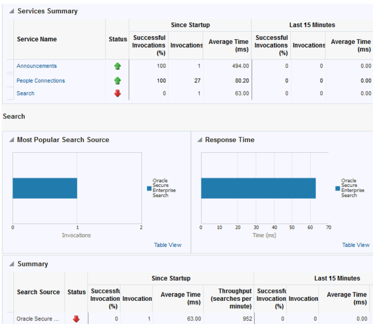
Figure 21-28 Search Metrics
