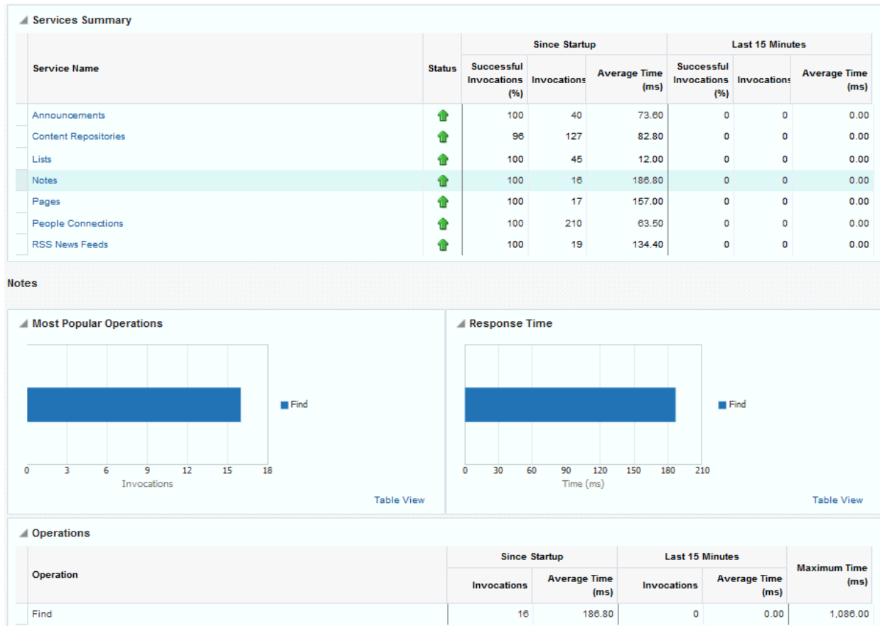
Figure 21-24 Notes Metrics
