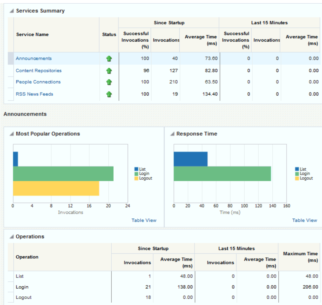
Figure 21-14 Announcements Metrics
