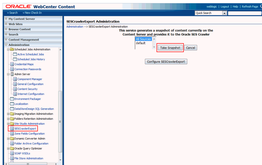
Figure B-14 Content Server Snapshot
