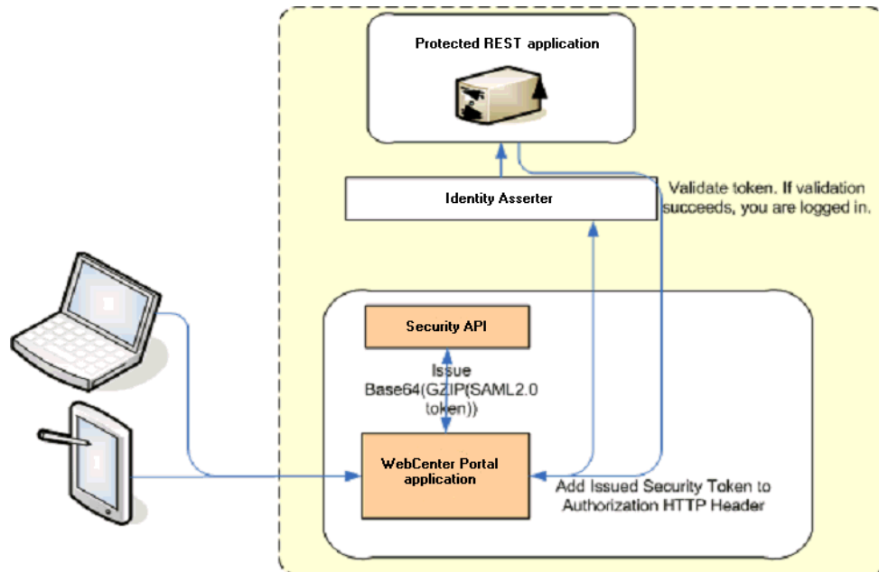
Figure 25-7 REST Identity Propagation and Assertion
