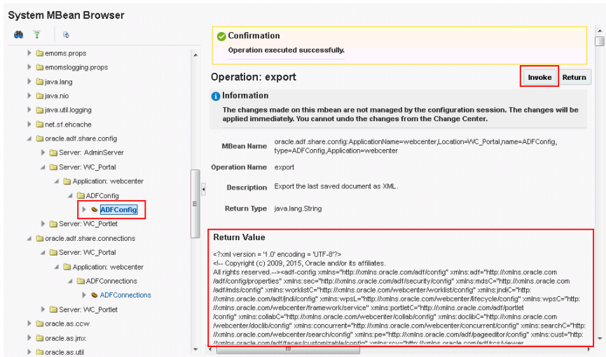
Figure C-1 Exporting Configuration Files with MDS Customizations
