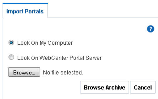
Figure 33-12 Importing Portals
