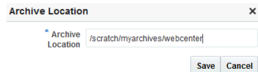
Figure 34-6 Archive Location
