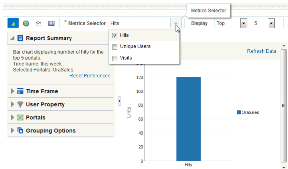
Figure 44-11 Analytics Task Flow - Metrics Selection
