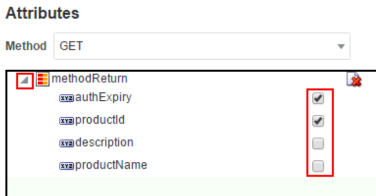
Figure 28-3 Create New Business Object: Attributes
