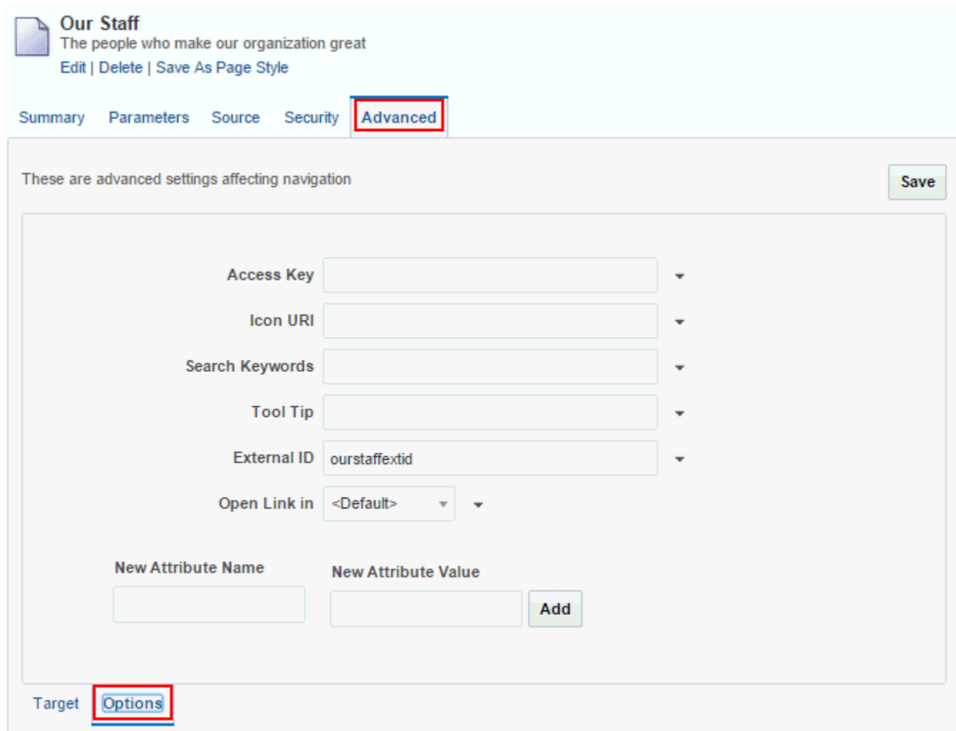
Figure 9-18 Setting Navigation Options for a Page: Options Tab (in Portal Editor)
