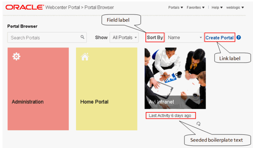
Figure 61-1 User Interface Elements Displayed in WebCenter Portal
