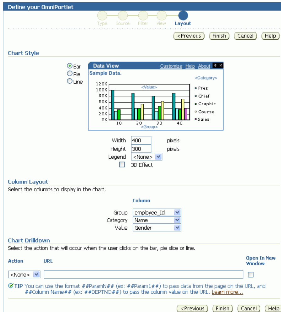
Figure 13-13 Layout Tab: Chart
