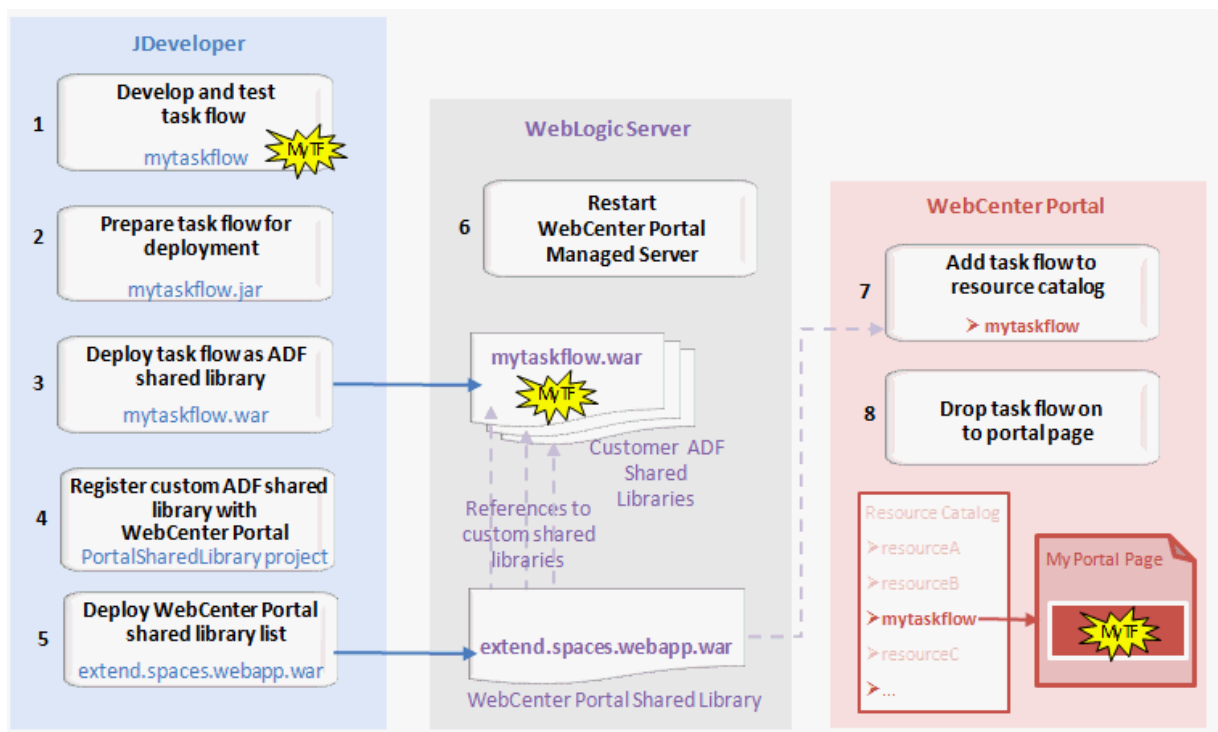
Figure 21-1 Development Lifecycle for an ADF Task Flow
