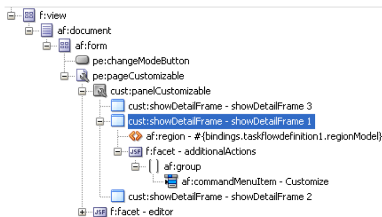
Figure 23-2 Page1.jspx in Structure Navigator
