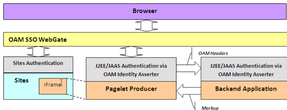
Figure 20-26 Pagelet Producer Calling the Backend Application Directly
