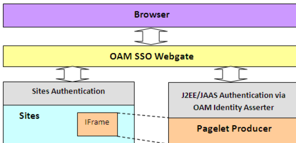
Figure 20-23 Ideal Frontend Authentication Configuration Using OAM
