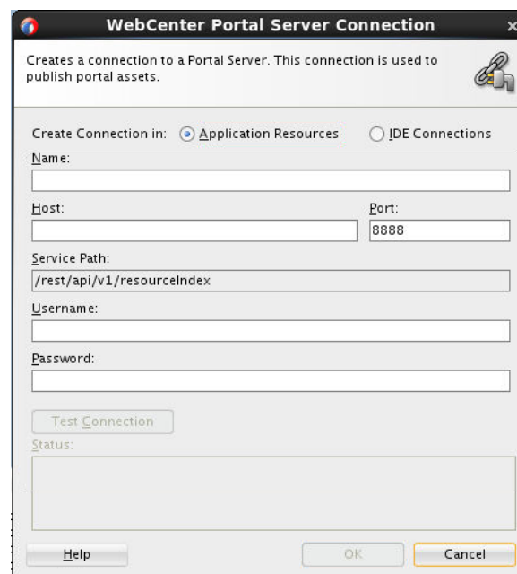
Figure 4-7 WebCenter Portal Server Connection Dialog
