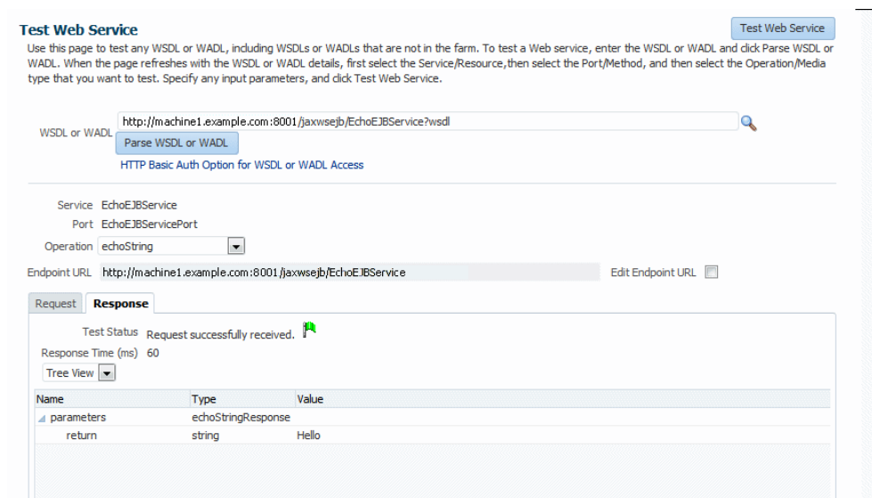
Figure 5-3 Successful Test for a WSDL
