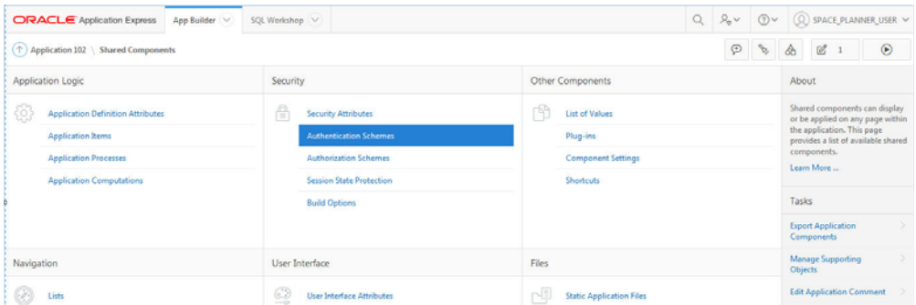
Figure 16–18 Authentication Scheme
