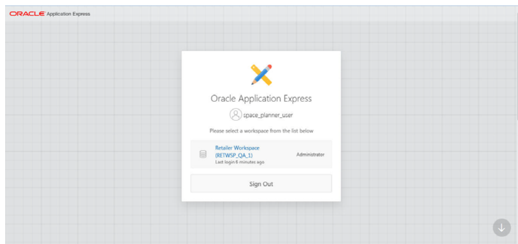
Figure 16–38 Retailer Workspace
