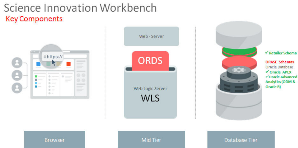
Figure 16–1 Innovation Workbench Key Components
