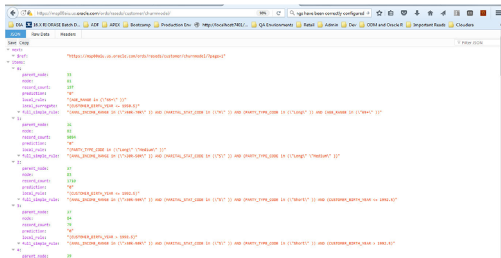
Figure 16–37 RESTful Refresh
