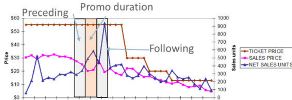
Figure 17–4 Promotion Window
