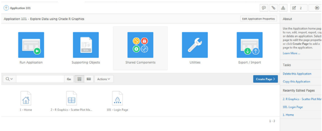
Figure 16–17 Shared Components
