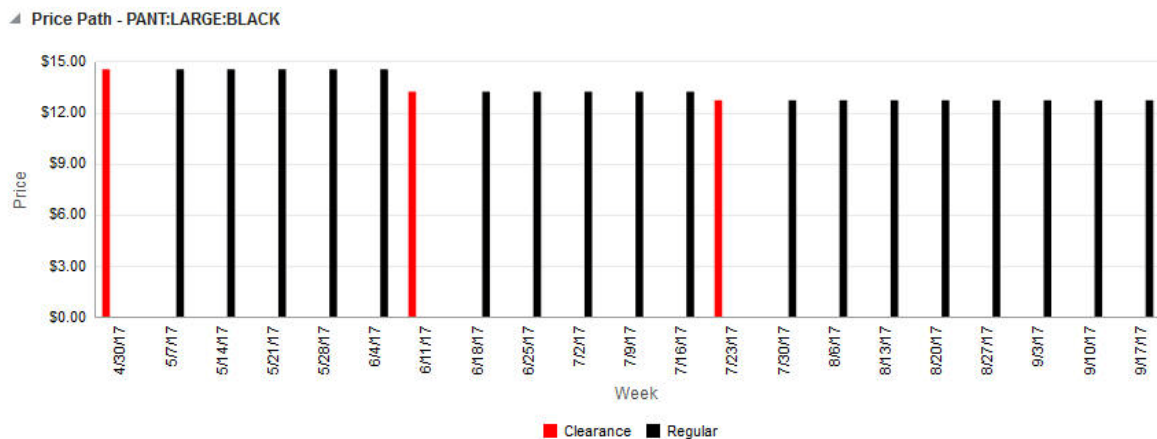
Figure 10-30 Markdown Price Path
