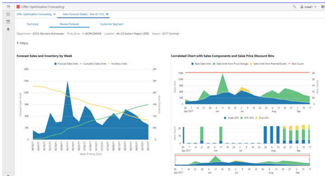
Figure 10–38 Review Forecast Tab
