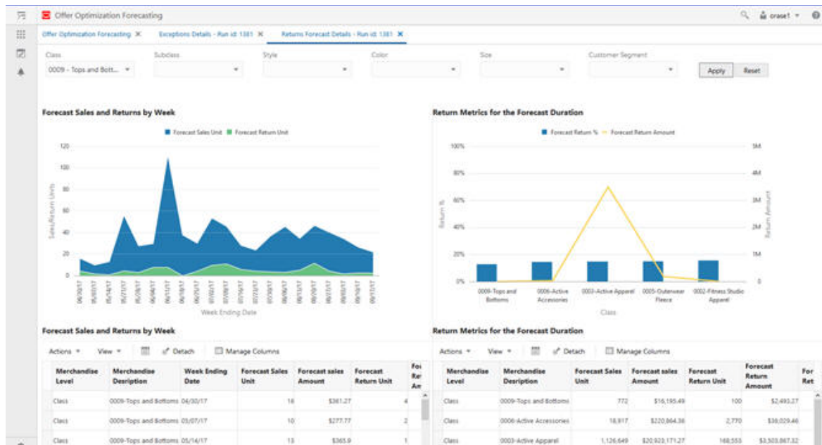
Figure 10-46 Compare Return Metrics
