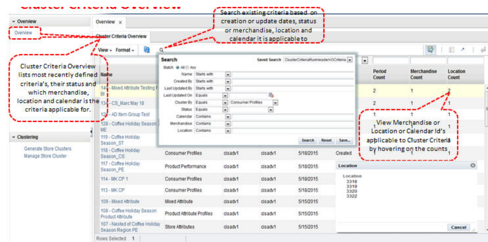
Figure 4–1 Cluster Criteria Overview Tab
