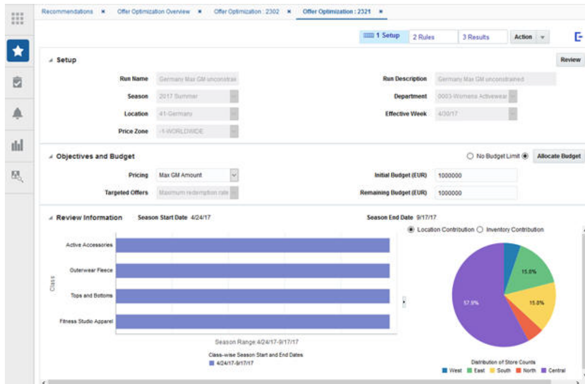
Figure 10–7 Offer Optimization Run Tab
