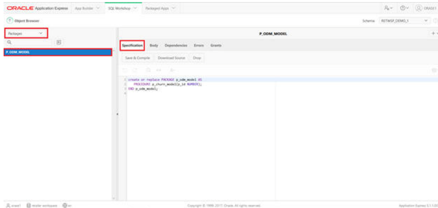
Figure A-57 Packages and Specification
