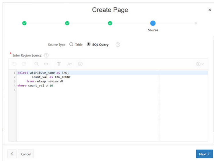
Figure A–40 SQL Query
