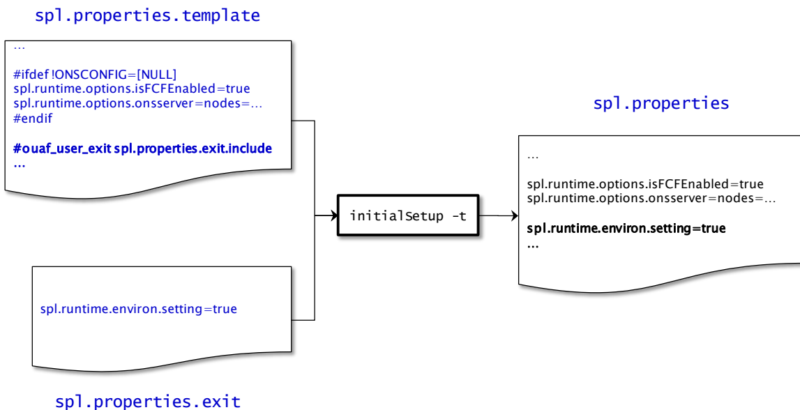
Figure 40 – Include files
