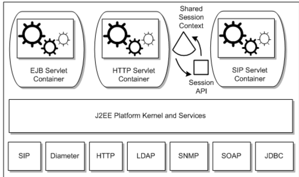
Figure 1–2 Converged Application Server Extended Java EE for Next Generation Networks
