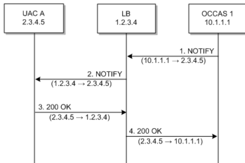
Figure 5–7 NOTIFY Sequence
