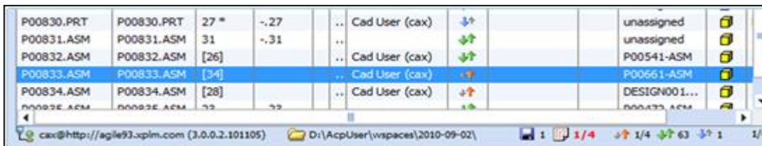
Figure 166: Status Information
