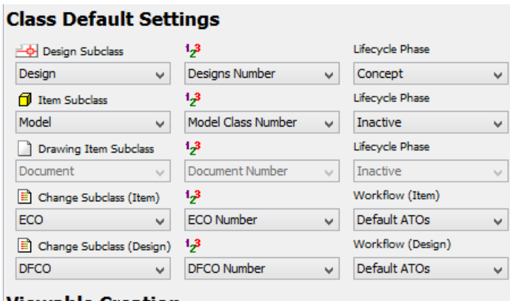
Figure 17: Class Preferences
