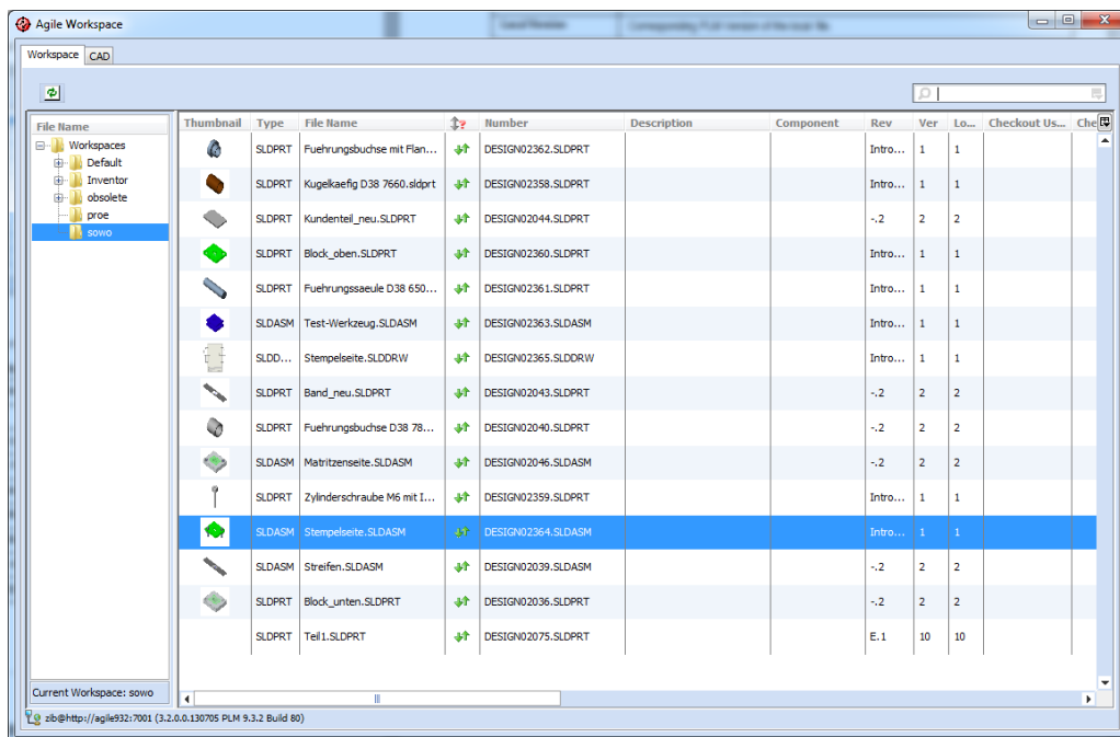
Figure 32: Agile Workspace
