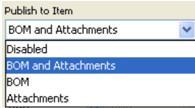
Figure 11: Publish Behavior
