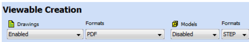
Figure 14: Viewable Creation
