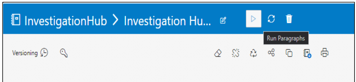
Figure 14: Execute Notebook
