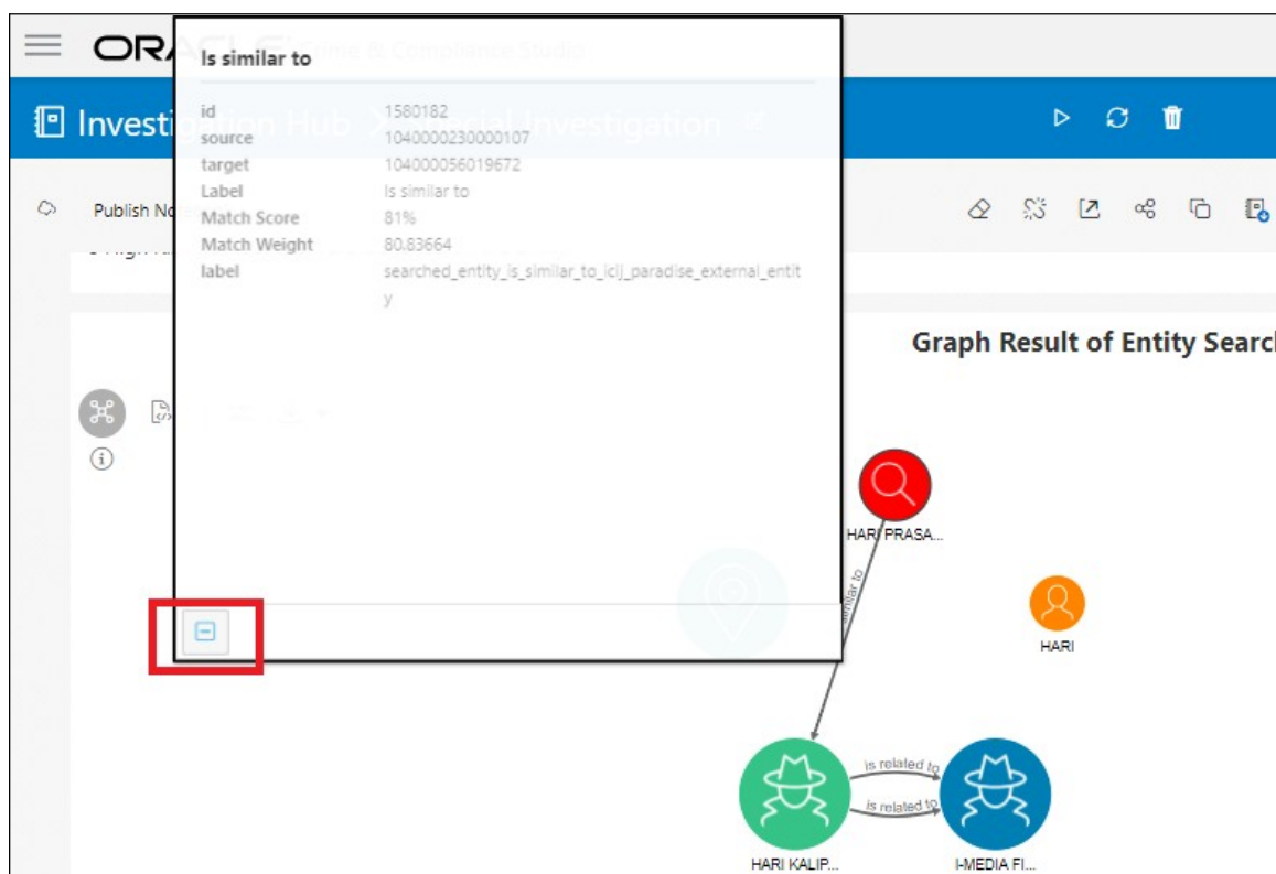
Figure 53: Removing an Edge
