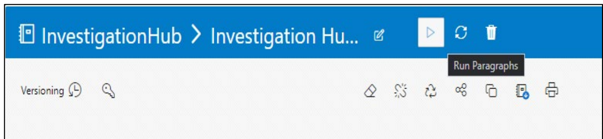
Figure 15: Execute Notebook
