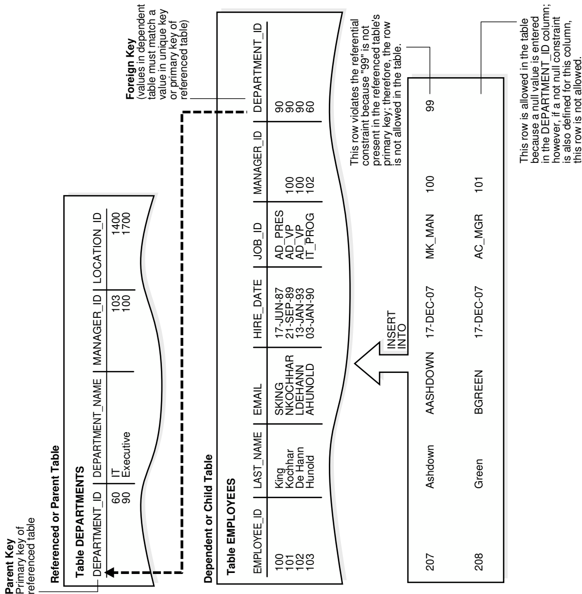
Figure 5-1 Referential Integrity Constraints
