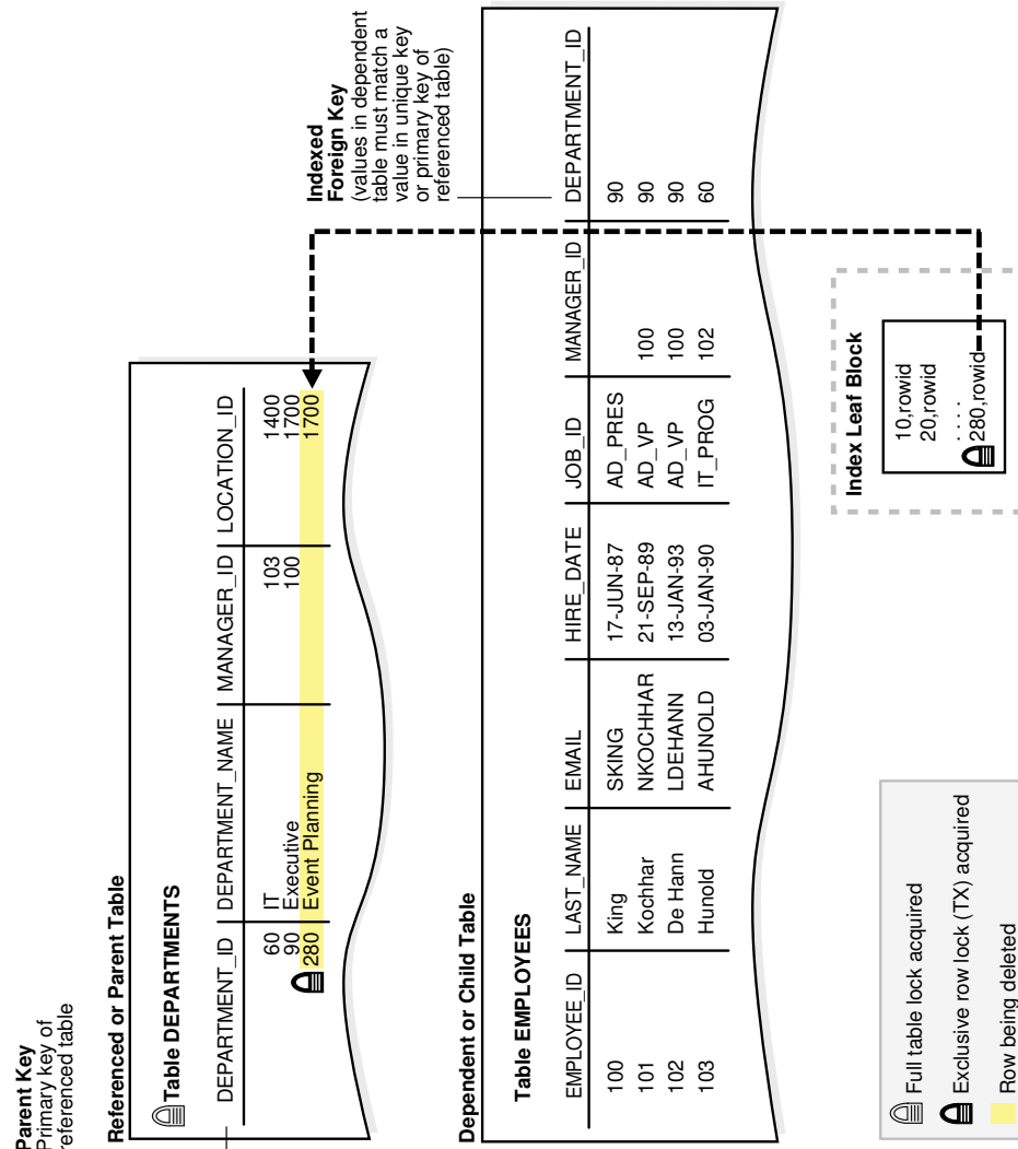
Figure 10-4 Locking Mechanisms with Indexed Foreign Key
