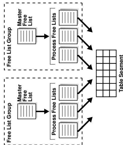
Figure 13-5 Free List Groups
