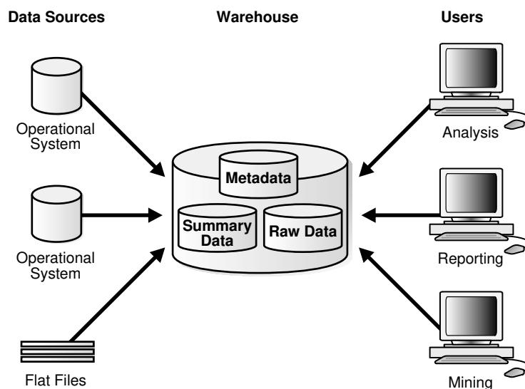
Figure 18-3 Architecture of a Data Warehouse
