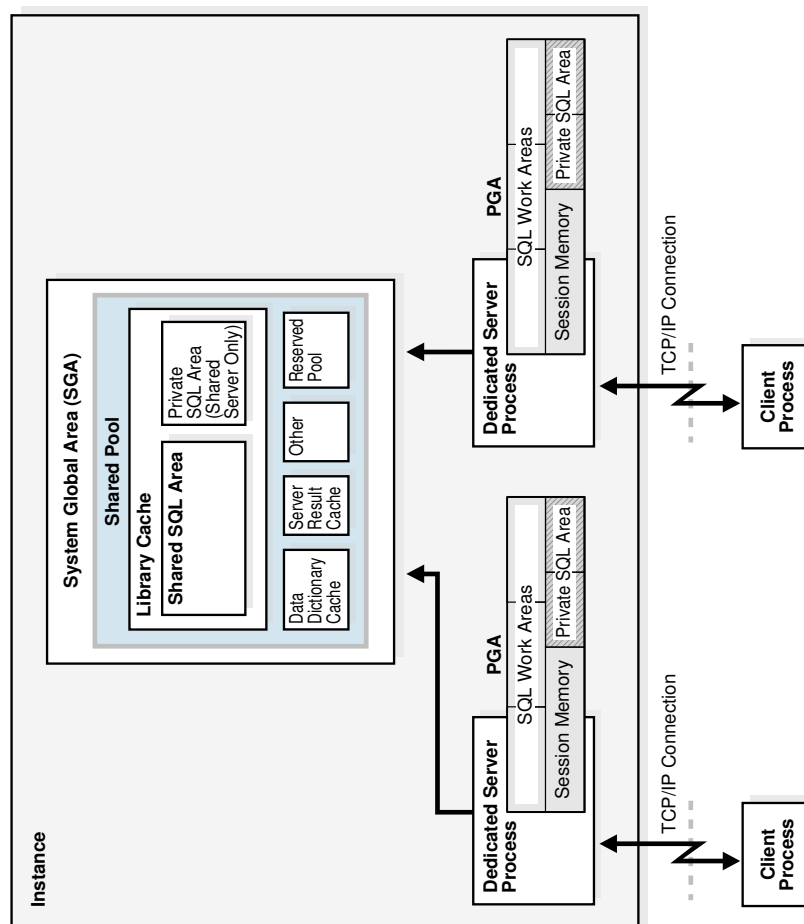
Figure 17-7 Oracle Database Using Dedicated Server Processes
