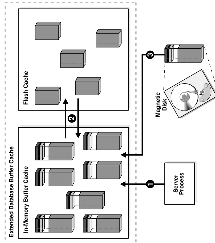
Figure 15-6 Buffer Search
