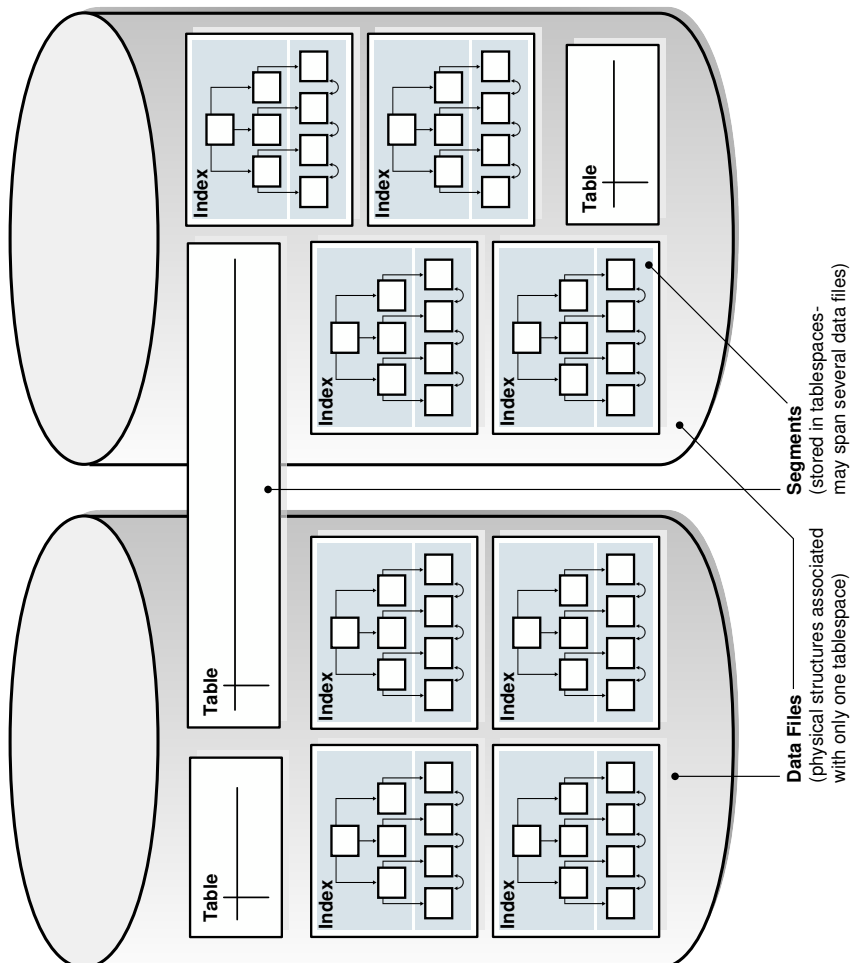
Figure 8-2 Optimizer Components
