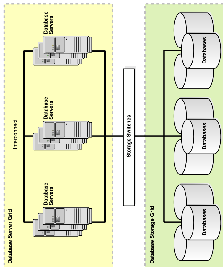
Figure 18-2 Grid Computing Environment
