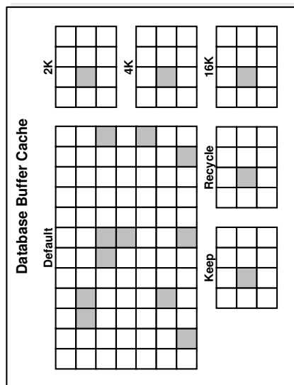
Figure 15-7 Database Buffer Cache
