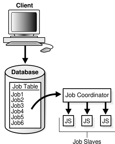
Figure 19-8 Scheduler Components
