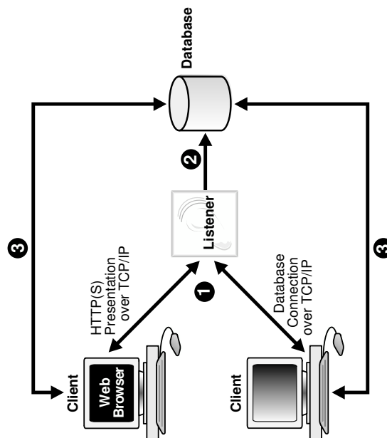
Figure 17-5 Listener Architecture
