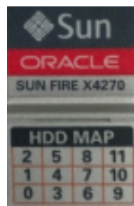
Figure 10 Disk Layout in Exadata Storage Server with Sun Fire X4270 M2 Servers
