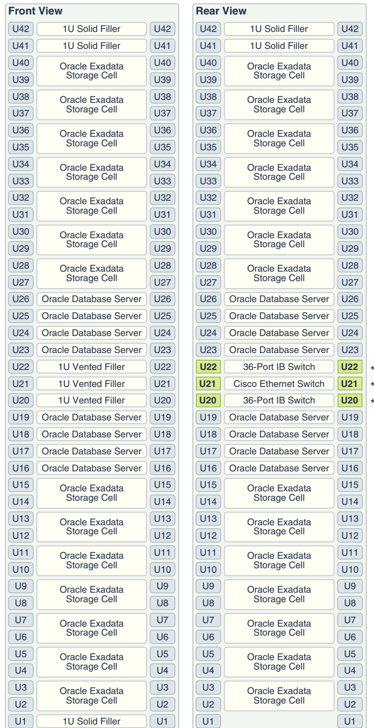
Figure 5-1 Rack Layout of Oracle Exadata Database Machine X8-2 and X7-2 Full Rack
