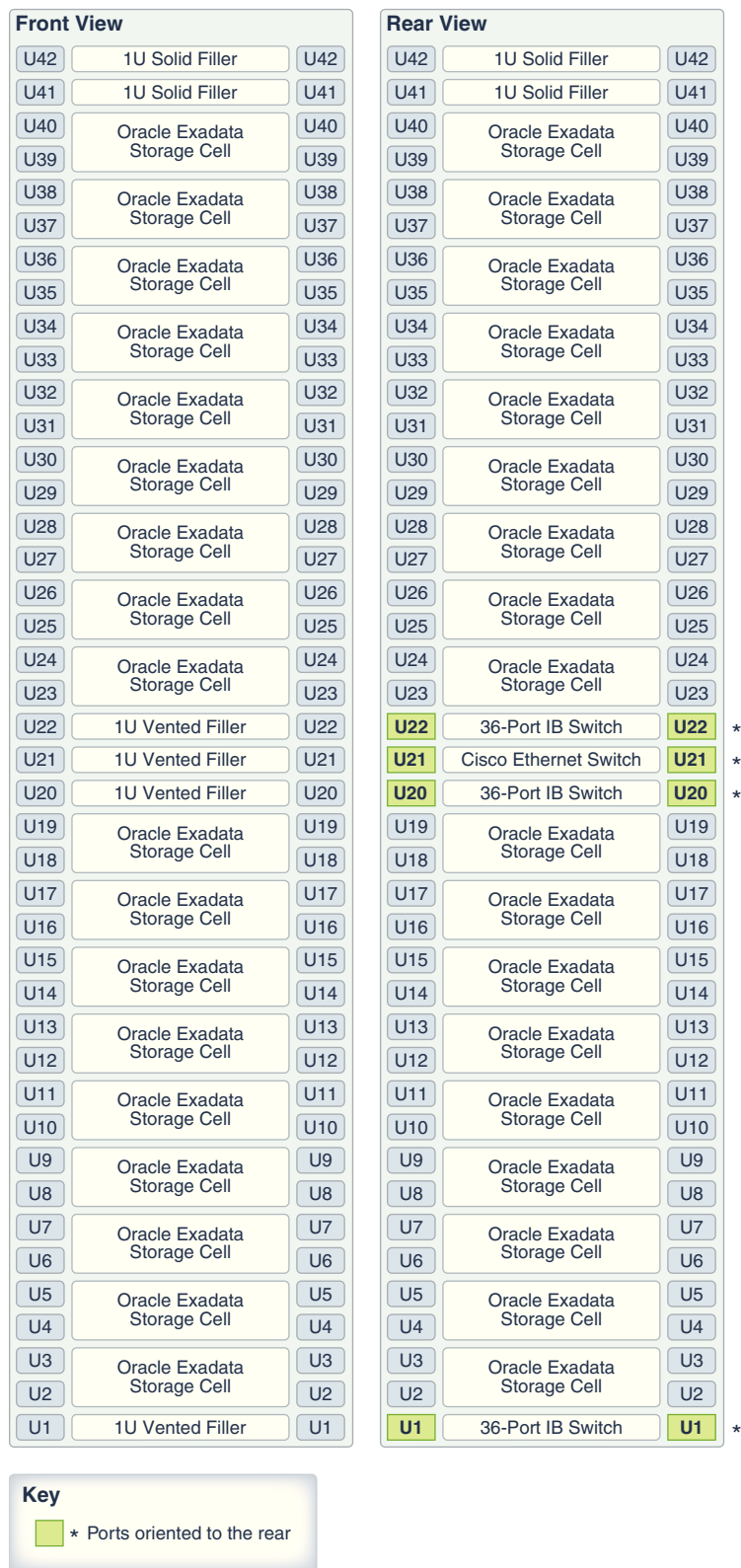
Figure 10-1 Rack Layout of Oracle Exadata Storage Expansion Full Rack X5 and Later
