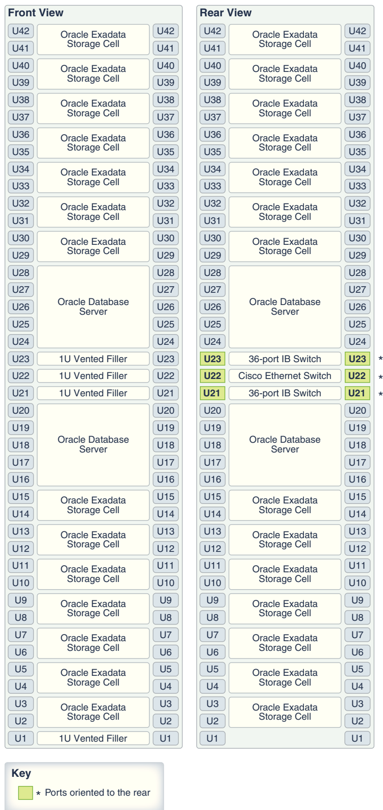
Figure 5-2 Rack Layout of Oracle Exadata Database Machine X8-8 and X7-8
