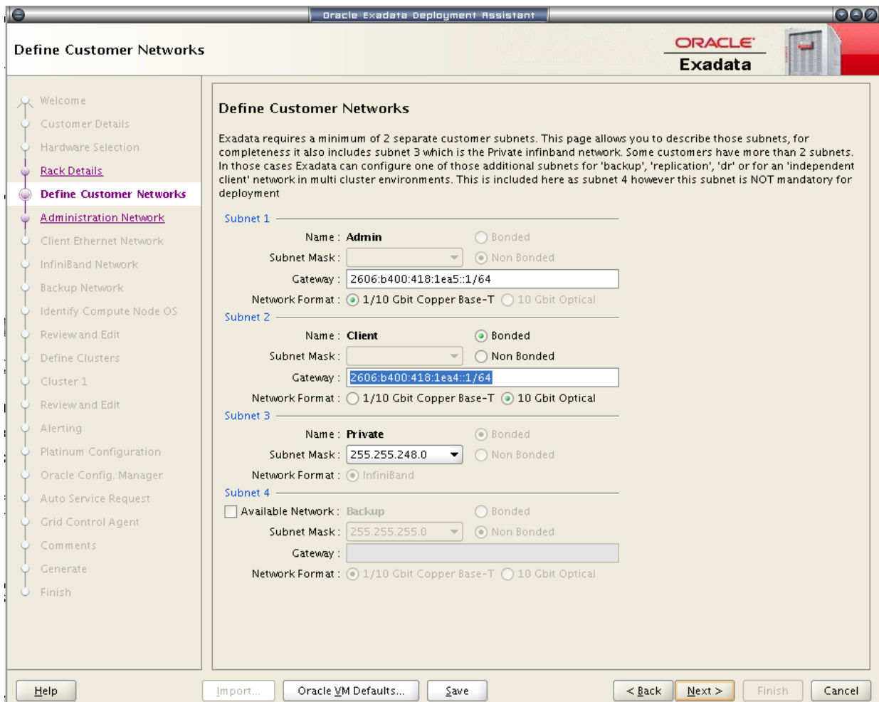
Figure 8 "Define Customer Networks" Screen in Oracle Exadata Deployment Assistant
