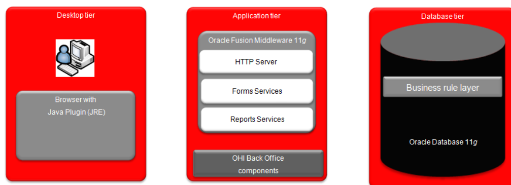
Figure 2: OHI Back Office GUI components
