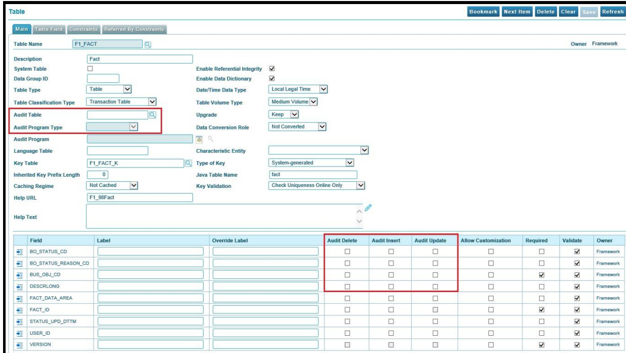
Figure 27: Table Screen
