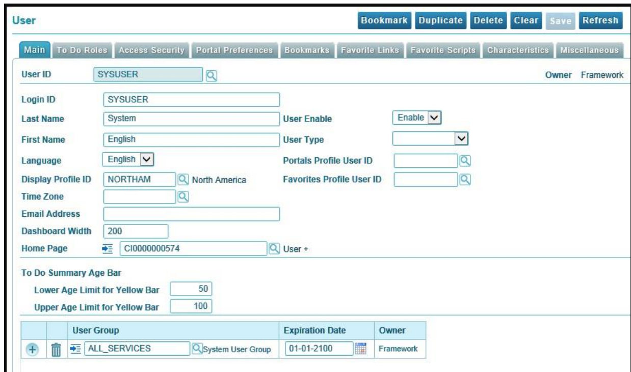
Figure 3: User Screen
