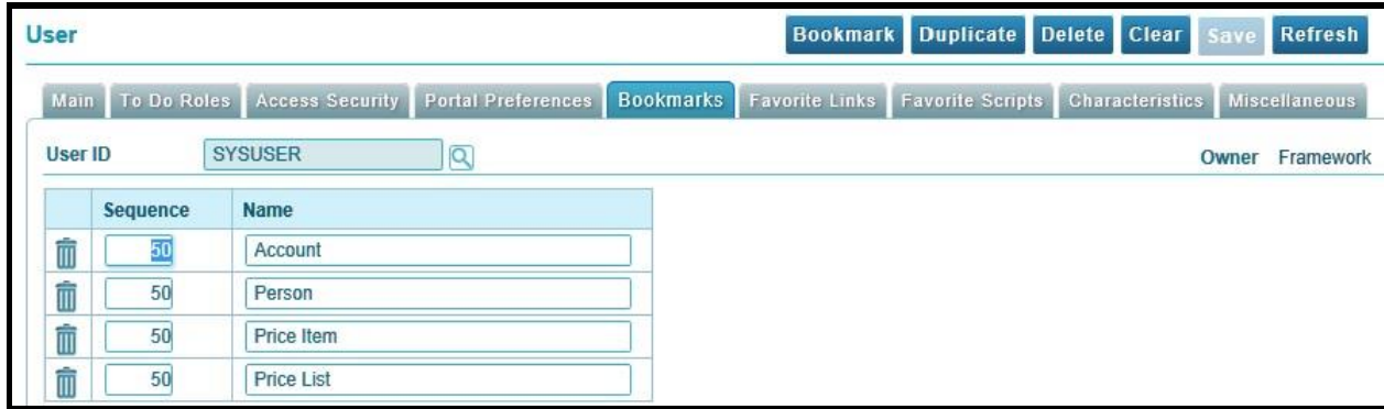
Figure 7: Bookmarks
