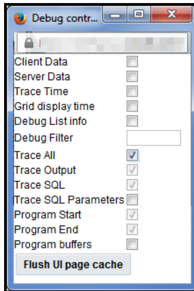
Figure 11: Debug Controls
