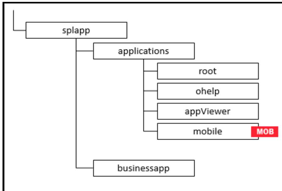
Figure 43: Expanded Format
