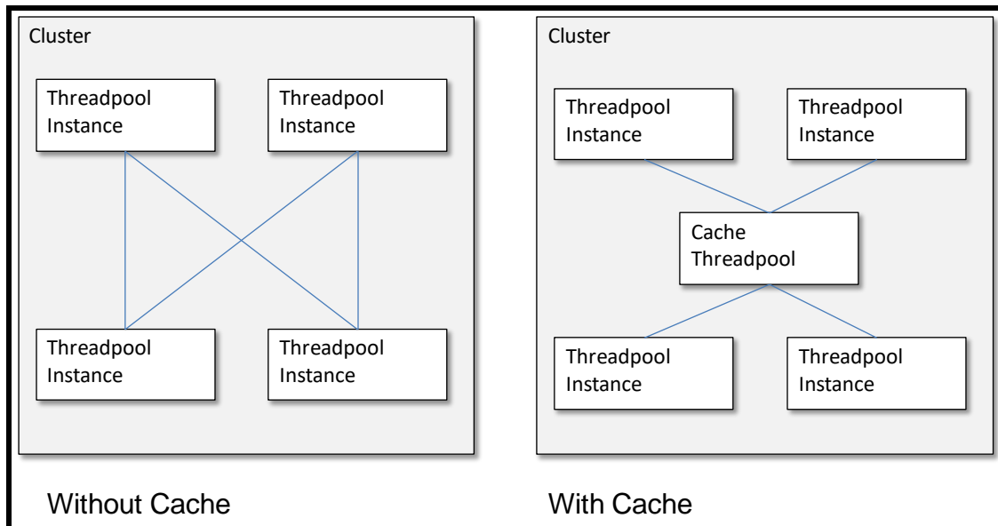
Figure 41: Cache Architecture
