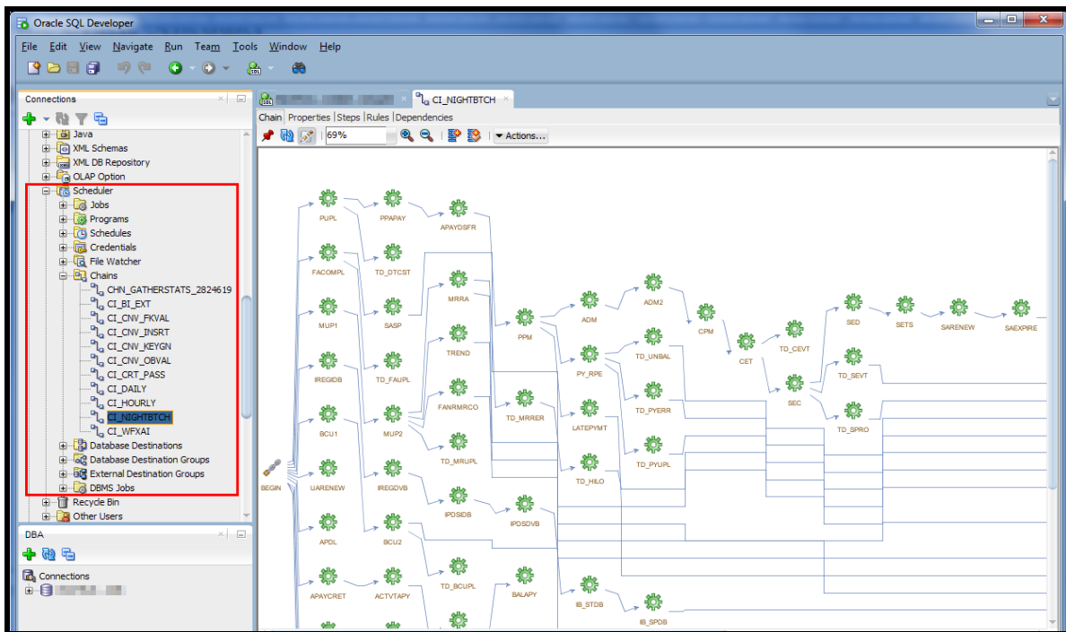
Figure 54: Example Oracle SQL Developer Oracle Scheduler Interface
