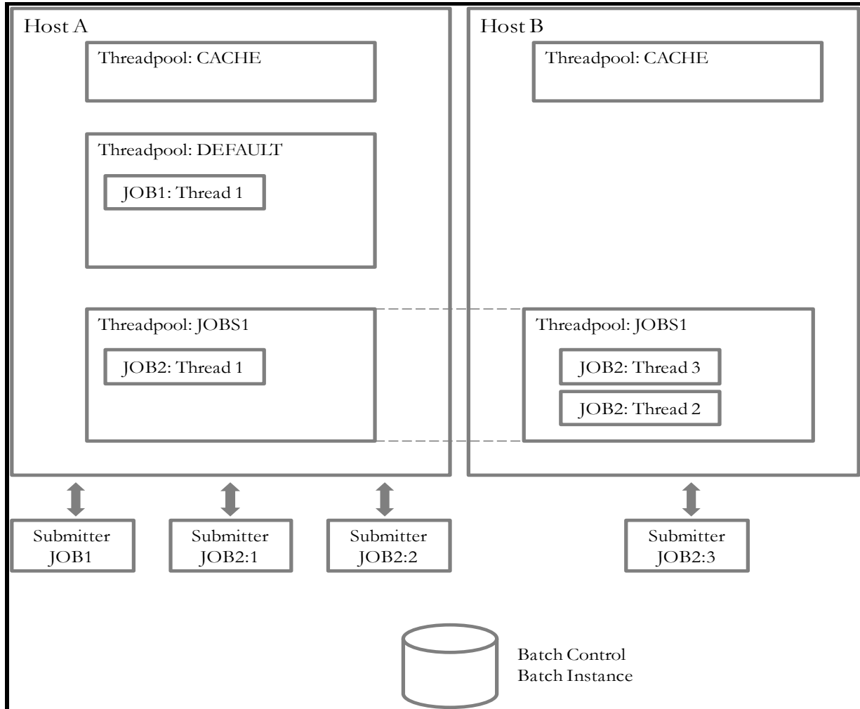
Figure 3: Batch Architecture Overview
