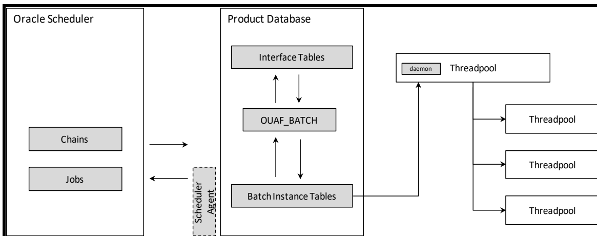
Figure 53: Oracle Scheduler Interface
