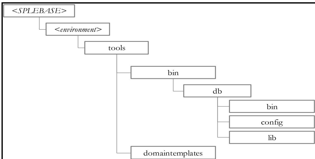
Figure 7: Tools Directory Structure
