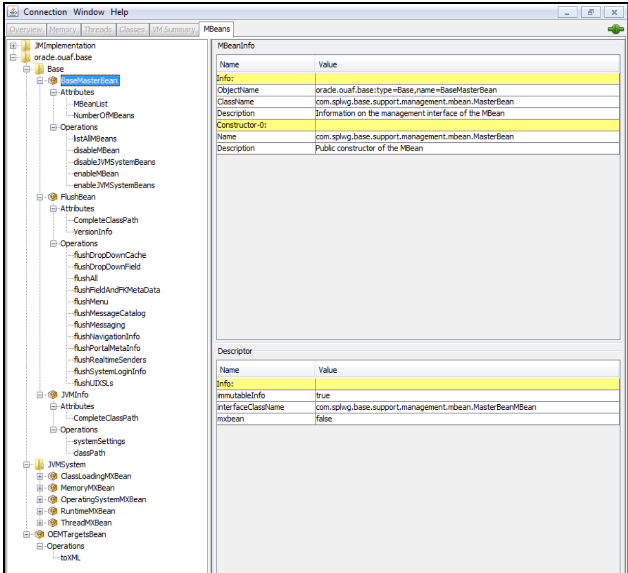
Figure 12: Example Web Application Server Mbeans in jconsole
