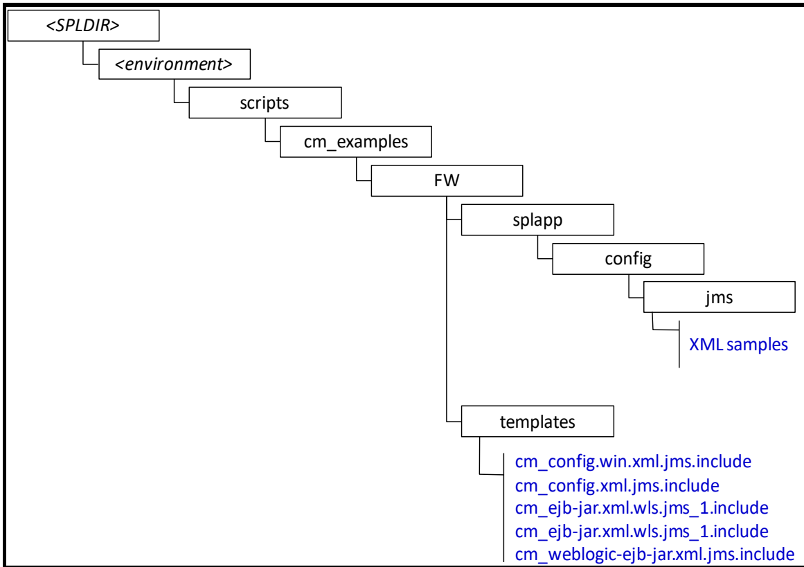
Figure 46: Custom JMS Configuration
