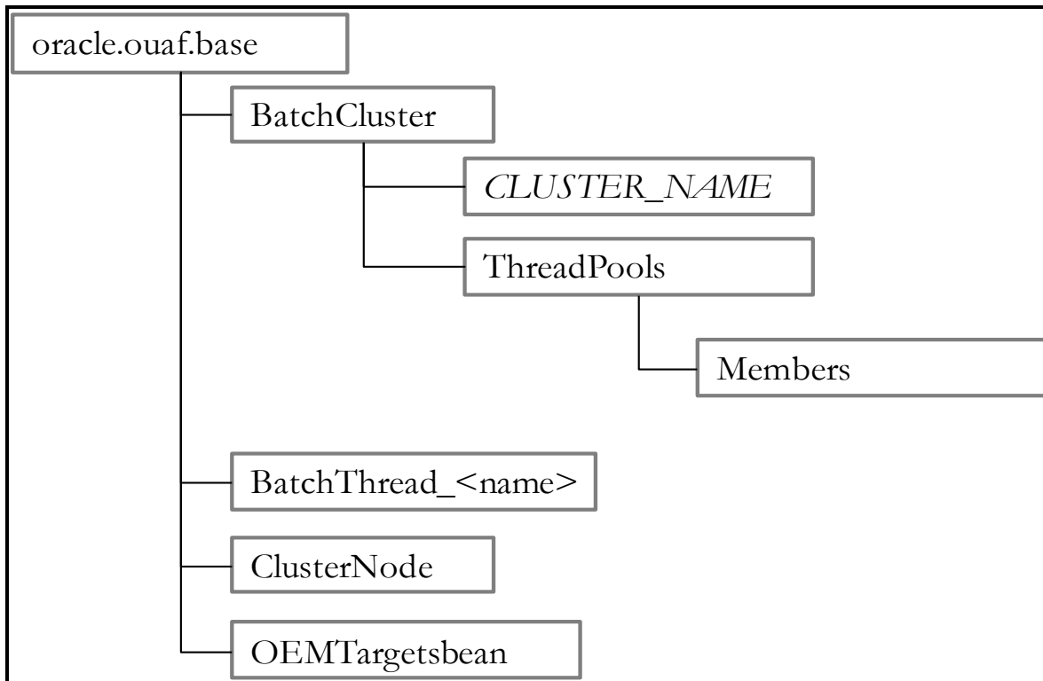
Figure 18: Batch Server Mbeans
