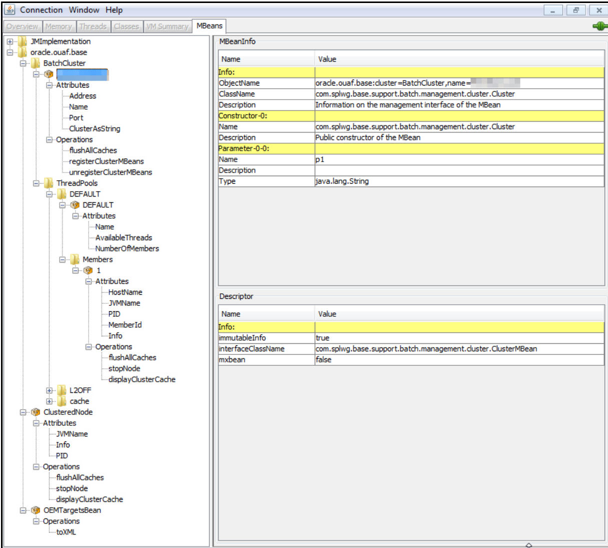
Figure 16: Batch Server Mbeans in jconsole Example
