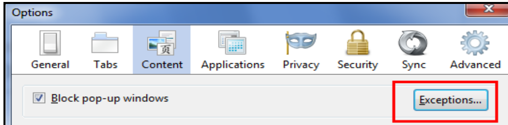
Figure 24: Exceptions
