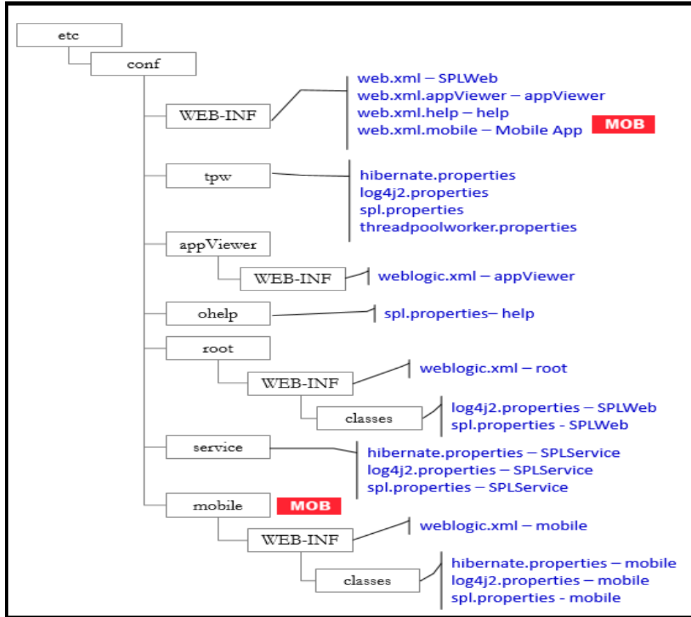
Figure 26: Configuration File Hierarchy
