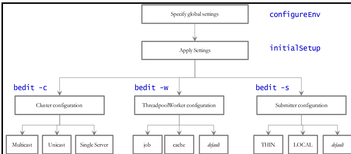
Figure 40: bedit Configuration Process
