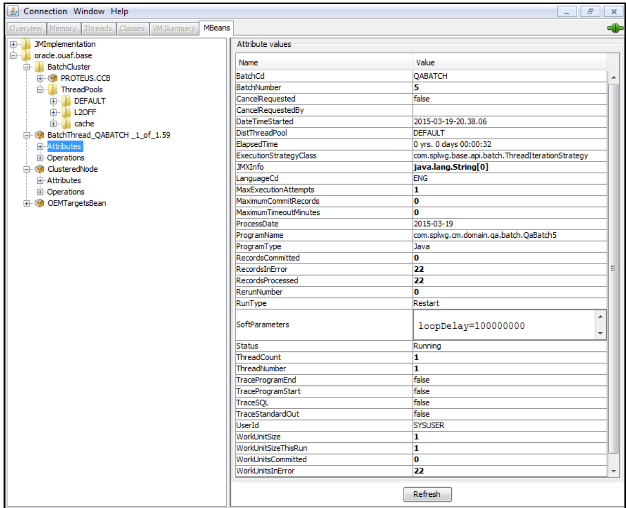
Figure 17: Batch Thread Mbean in jconsole Example
