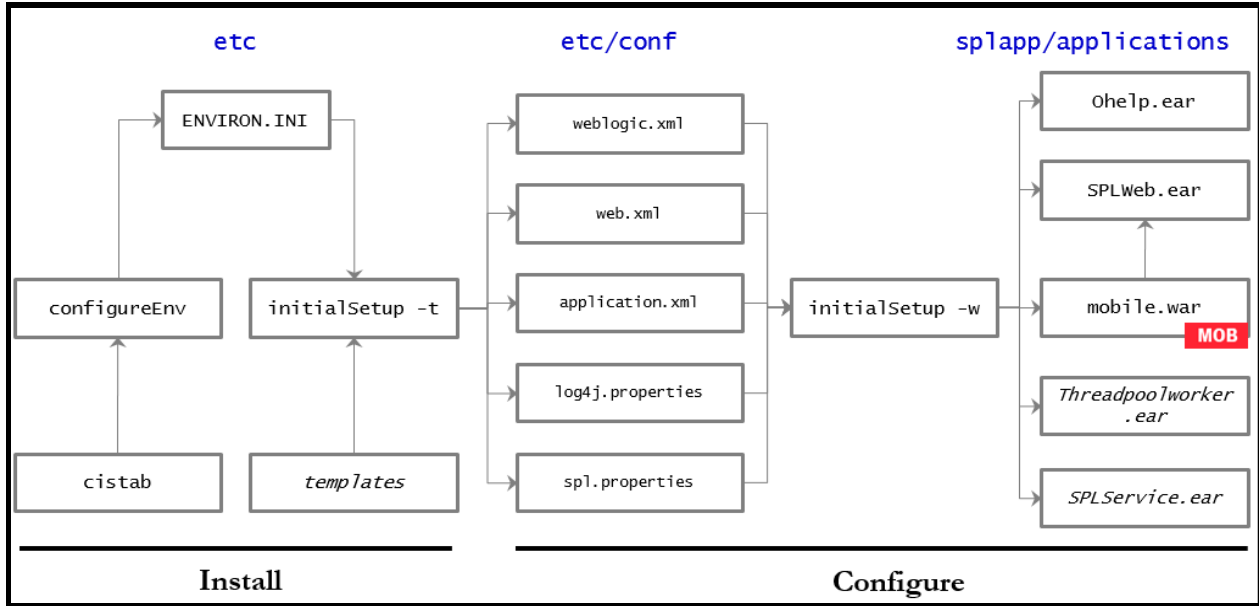
Figure 27: Web Application Server Configuration Process
