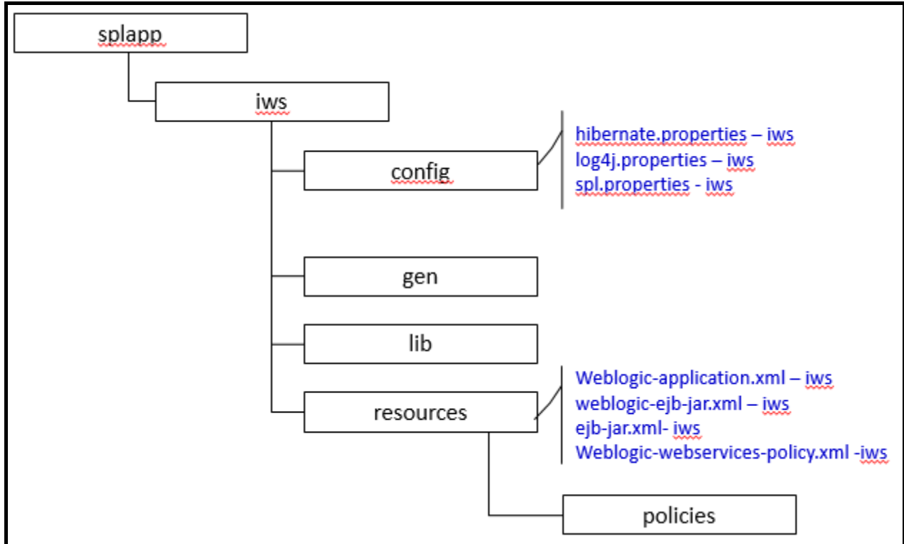
Figure 34: Inbound Web Services Structures
