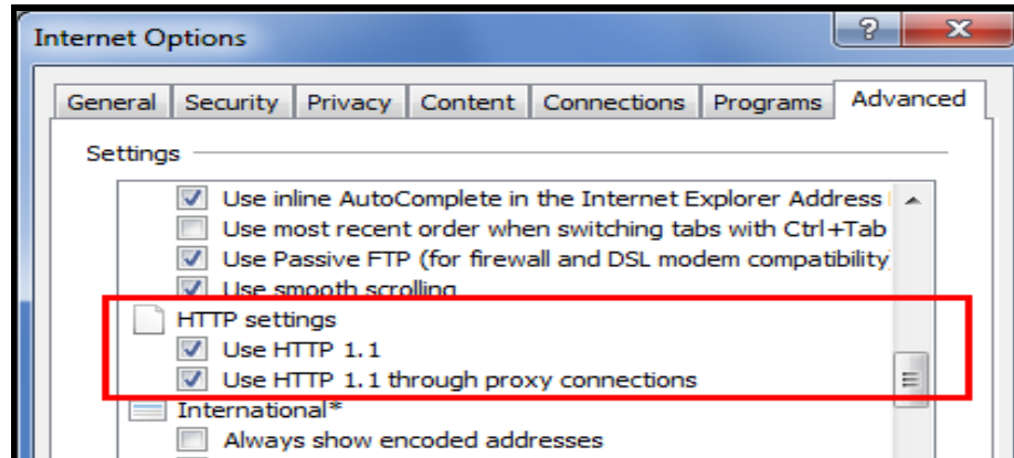
Figure 21: HTTP 1.1 Settings
