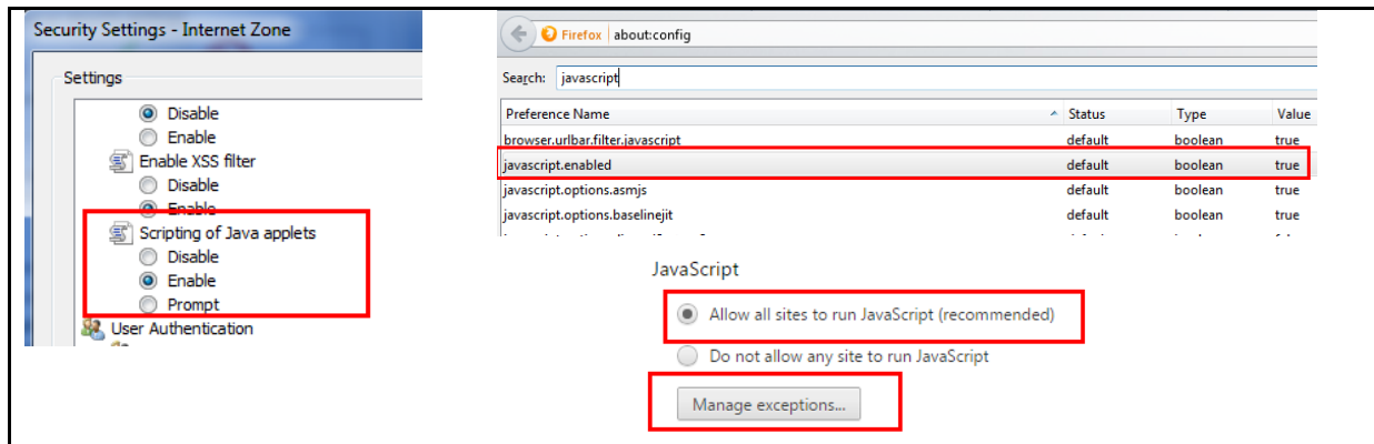
Figure 22: Javascript Settings
