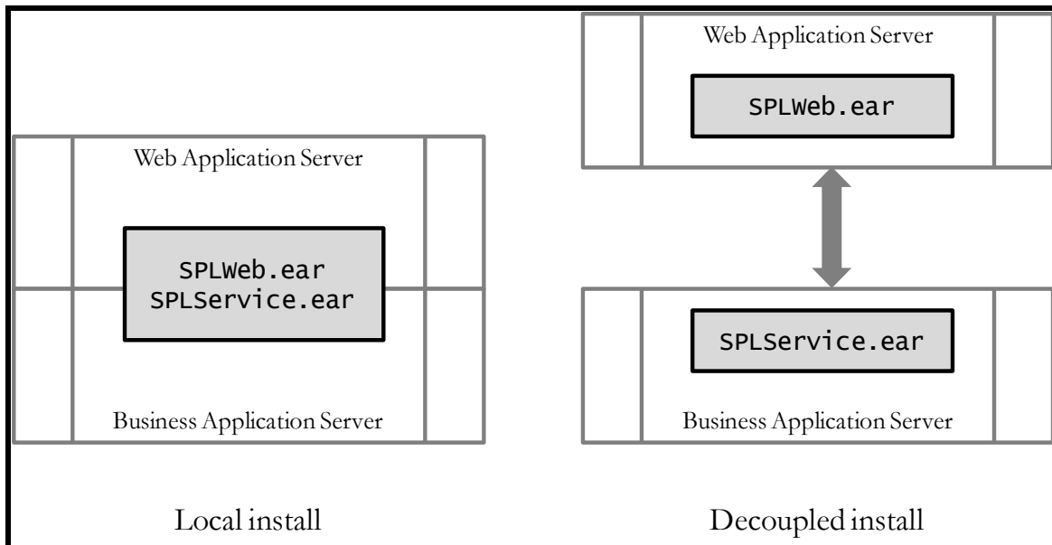
Figure 29: Installation Modes
