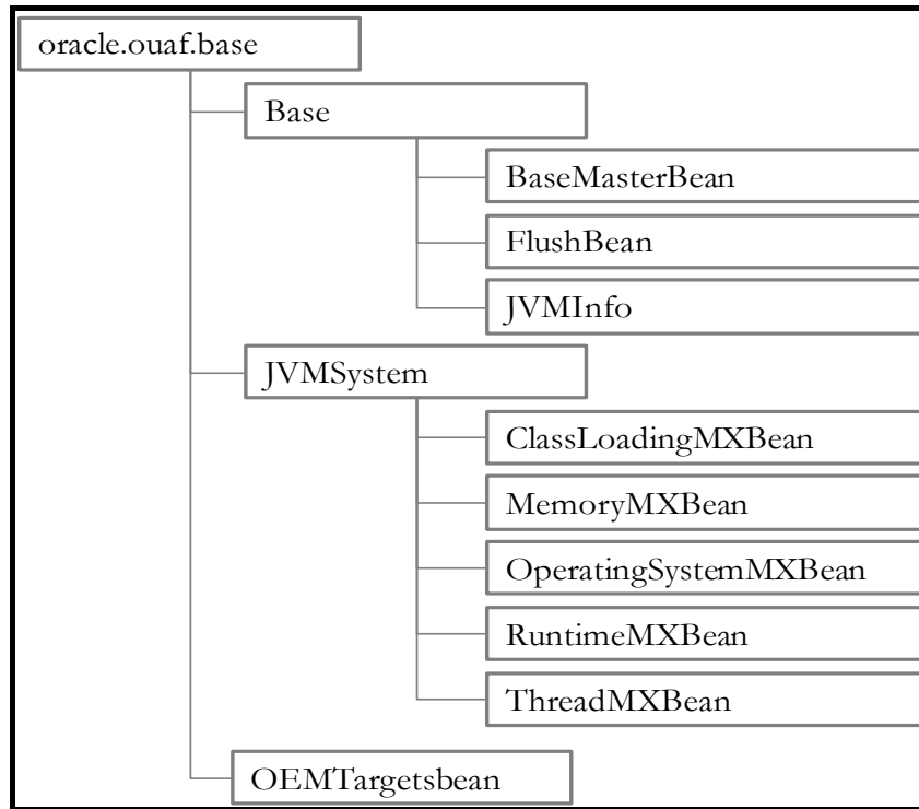
Figure 13: Web Application Server Mbeans
