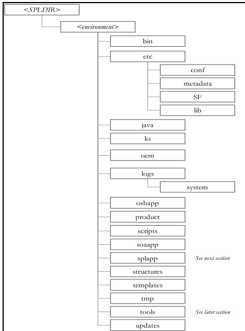
Figure 5: Software Directory Structure
