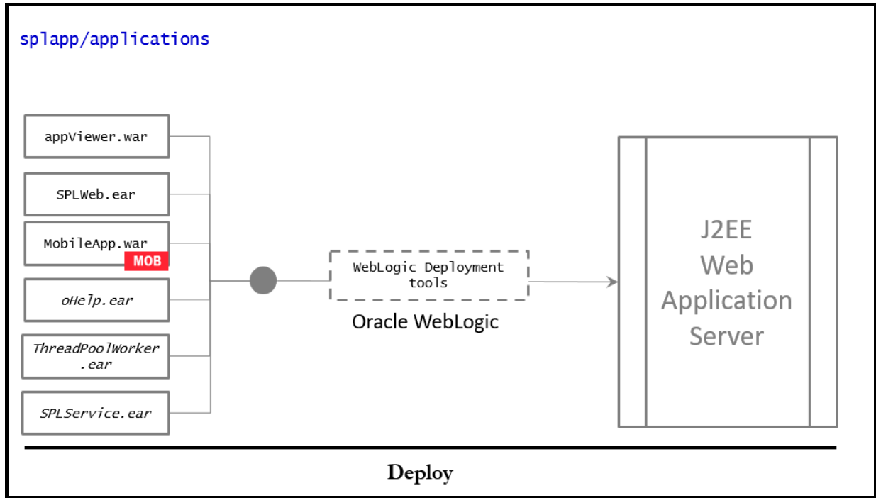
Figure 28: Web Application Server Deployment Process
