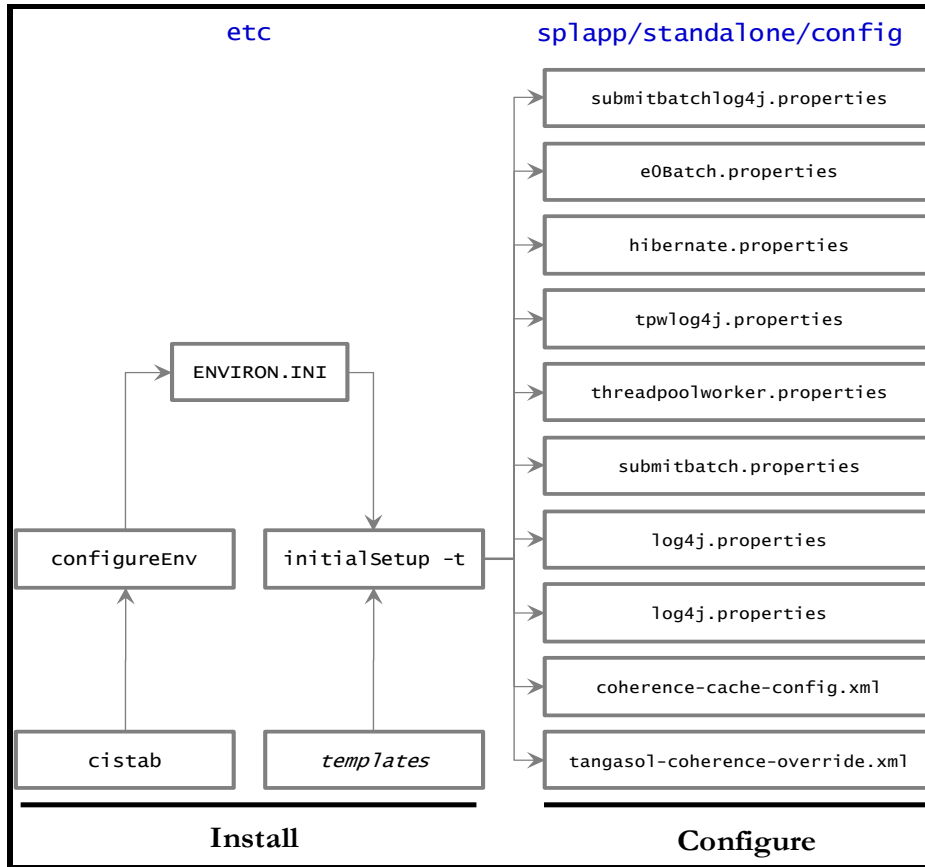
Figure 39: Batch Configuration Process
