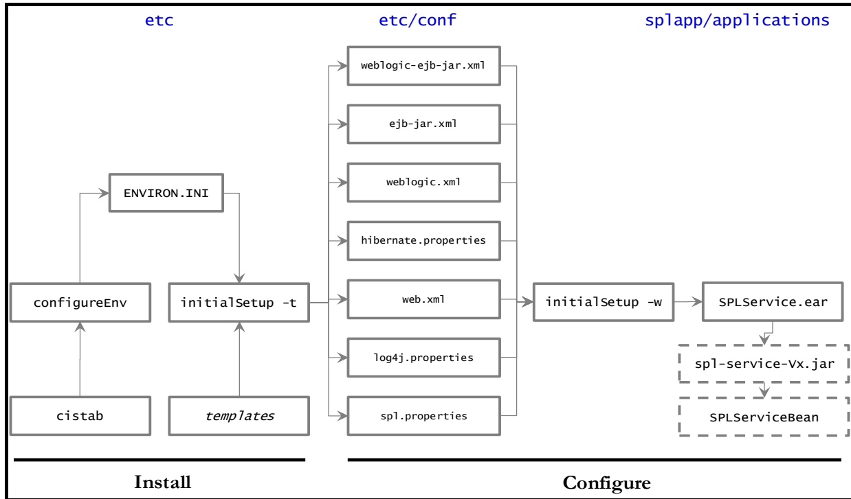
Figure 30: Business Application Server Configuration Process
