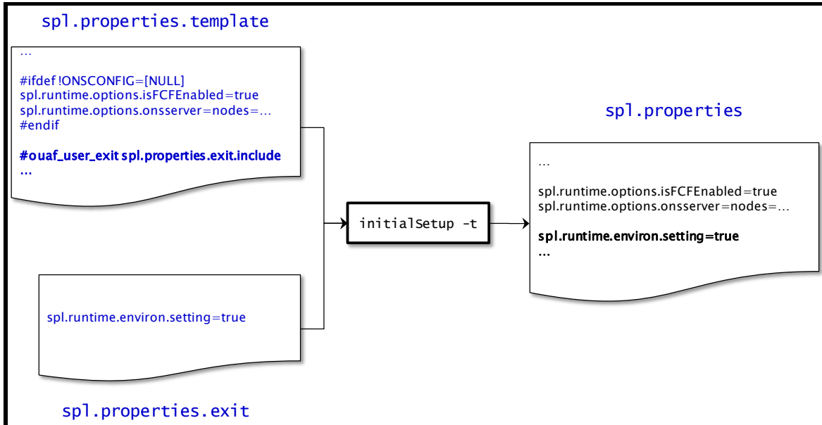
Figure 44: Include Files
