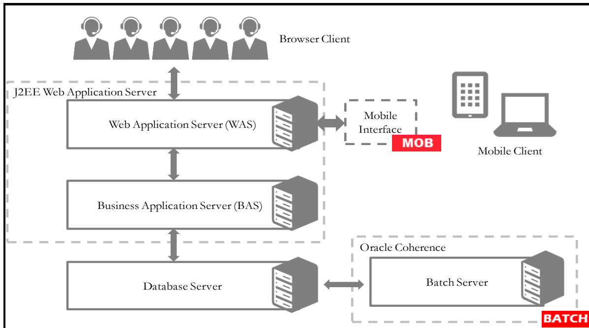
Figure 1: Product Architecture
