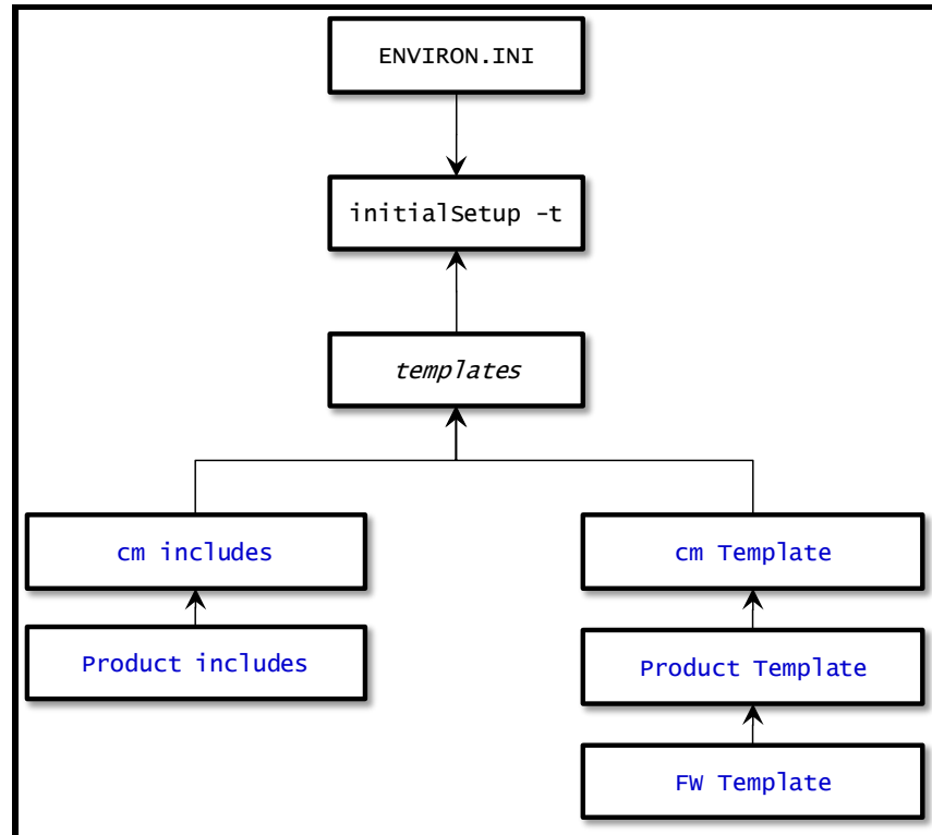
Figure 45: Template Hierarchy
