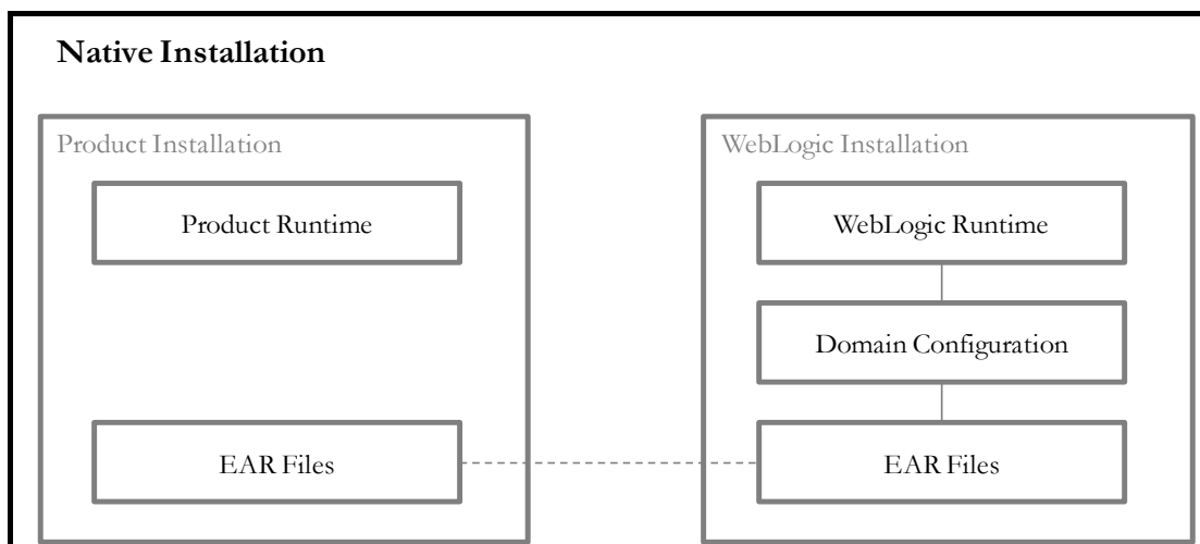
Figure 4: Native Architectures
