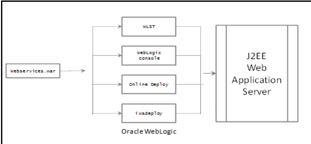
Figure 36: Inbound Web Services Deployment Process
